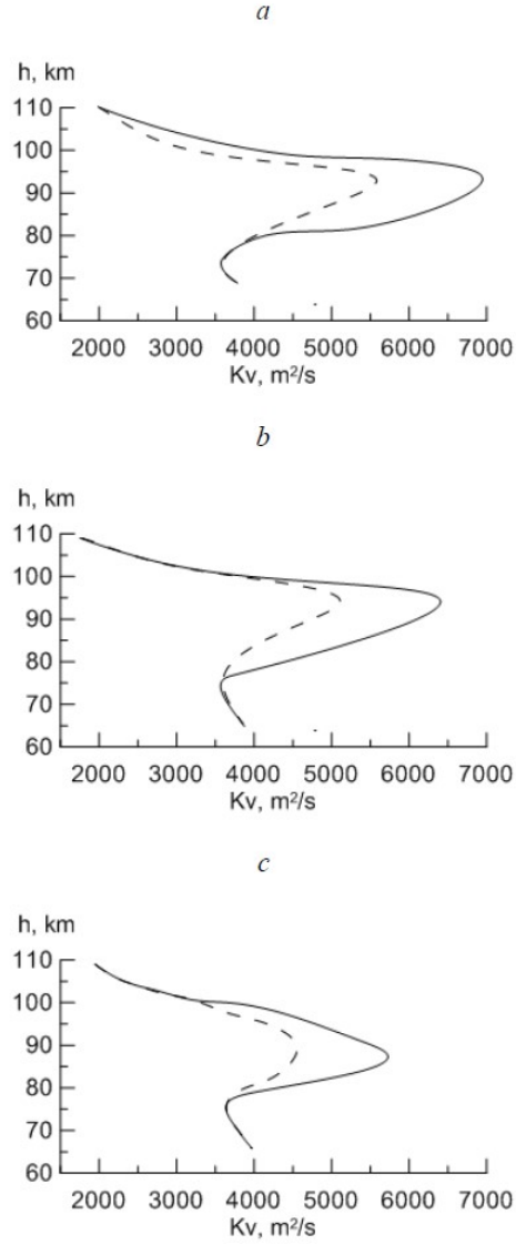
Figure 3: Turbulent viscosity coefficient: dash line - without atmospheric waves; solid line - disturbances caused by waves are accounted ( a - 28 August 2005, b - 19 October 2005, c - 18 July 2005).
