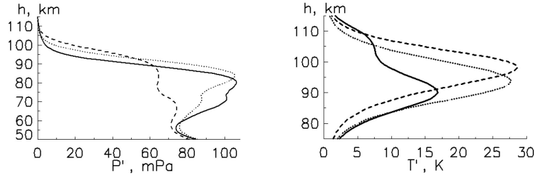
Figure 2: Change in pressure p' (a) and temperature T' (b) with the altitude as a result of passing of an AGW with a period of 65 minutes and k_x = 10^{-5} \text{ m}^{-1} (solid line - 18 July 2005, dashed line - 28 August 2005, dotted line - 19 October 2005).
