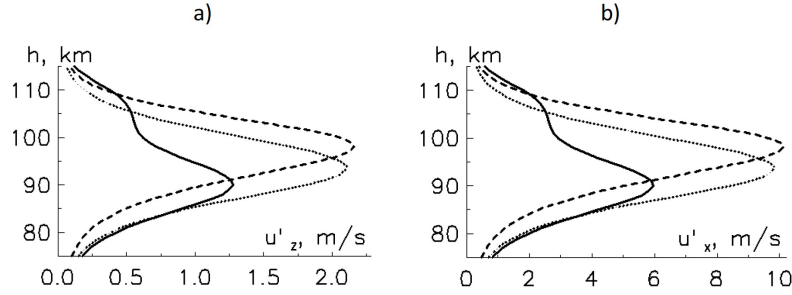
Figure 1: Change in vertical u'_z (a) and horizontal u'_x (b) component of velocity with altitude, as a result of passing of an AGW with a period of 65 minutes and k_x = 10^{-5} \text{ m}^{-1} (solid line - 18 July 2005, dashed line - 28 August 2005, dotted line - 19 October 2005).
