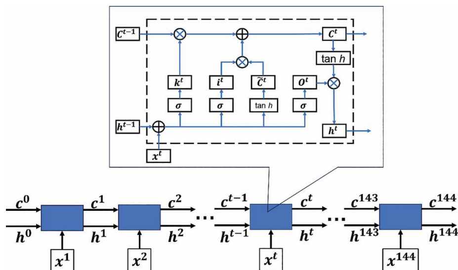
Figure 6 • The unrolled structure of proposed long short-term memory networks.
