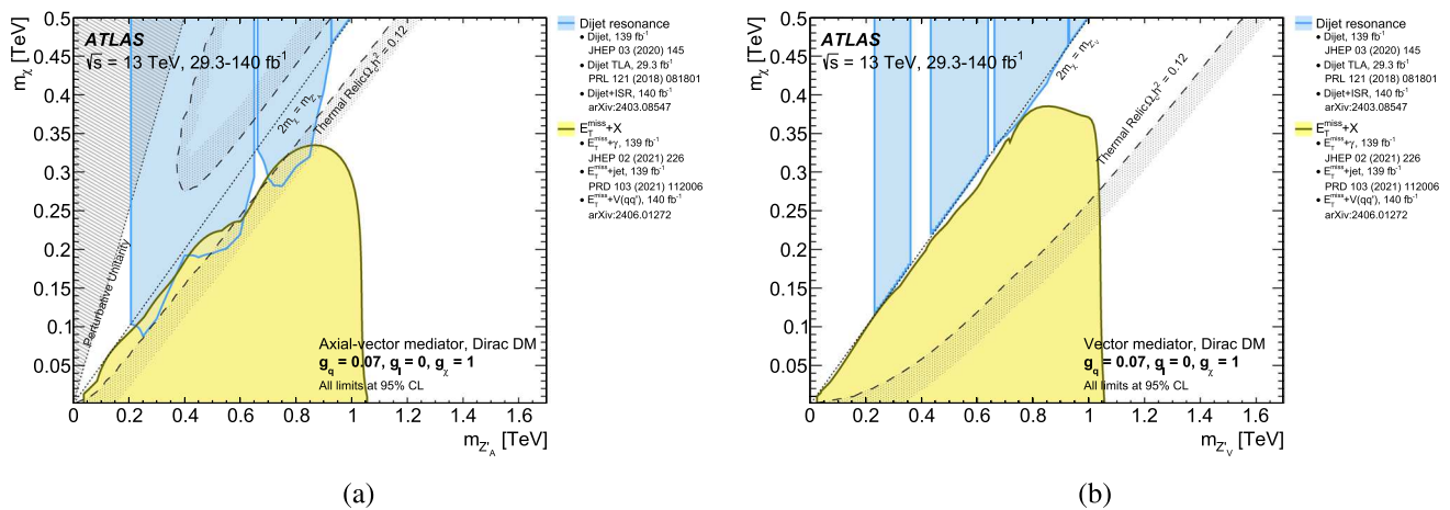
Fig. 9 Exclusions in the (m_\chi, m_{\text{Med}}) plane for benchmark models (a) A3 and (b) V3. The unions of multiple contours are plotted together as indicated in the figure legends. The dashed curves indicate points
