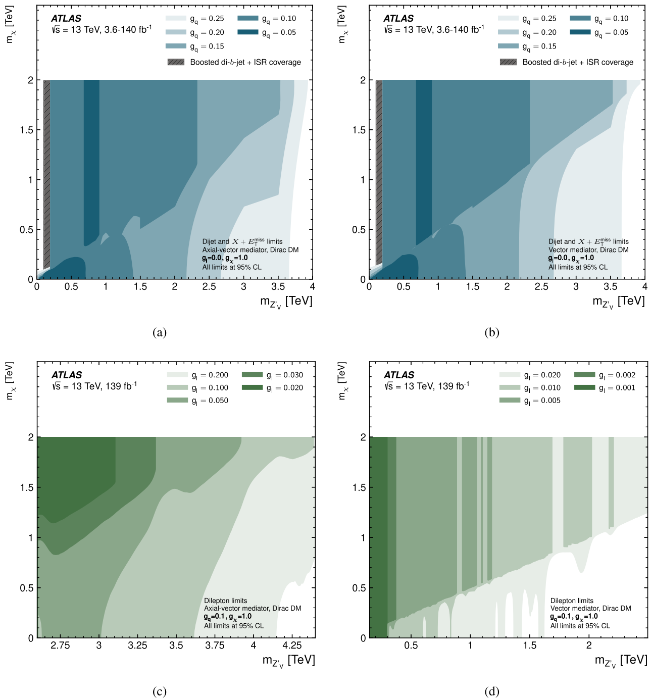
Fig. 7 Comparison of 95% CL exclusion contours for signal hypotheses (a),(b) varying in g_q for the dijet and X+E_T^{\text{miss}} analyses (dijet, dijet TLA, dijet ISR resolved, \gamma + E_T^{\text{miss}} , and Jet + E_T^{\text{miss}} ), and (c),(d) vary-
