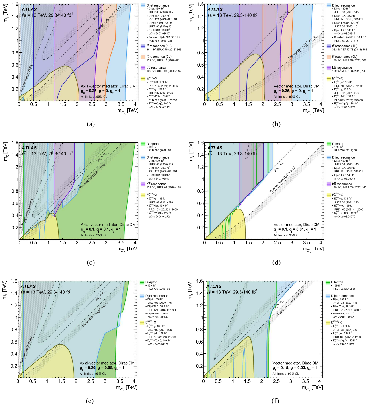
Fig. 8 Exclusions in the (m_\chi, m_{\text{Med}}) plane for axial-vector benchmark models (a) A1, (c) A2, and (e) A4, and vector benchmark models (b) V1, (d) V2, and (f) V4. The unions of multiple contours are plotted
