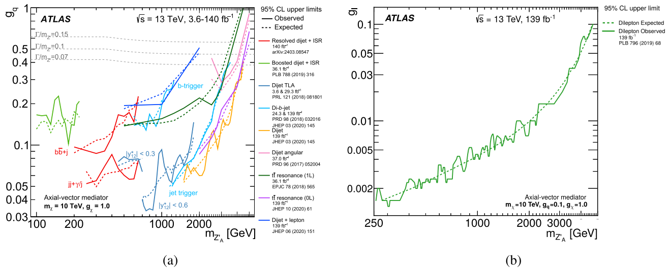
Fig. 6 95% CL upper limits on (a) g_q and on (b) g_l as a function of m_{Z'} . In these figures, m_\chi is set to 10 TeV to prevent the mediator from decaying into dark matter in the considered range of masses. The other parameters of the model are fixed to the values indicated in the figure, or equal to zero if not specified
