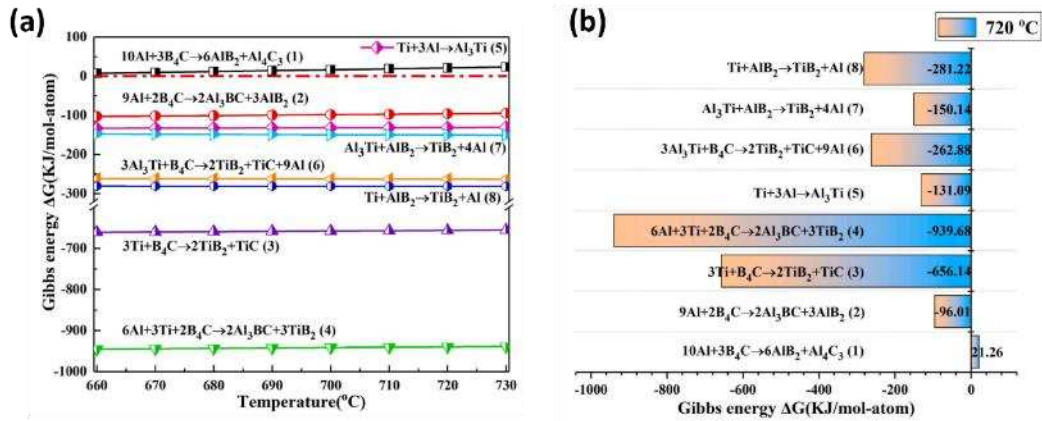
Figure 24. (a) Gibbs energy for each reaction at finite temperature; (b) Gibbs energy of different reactions at 720 °C. Reproduced with permission. [170] Copyright 2022, Elsevier.
