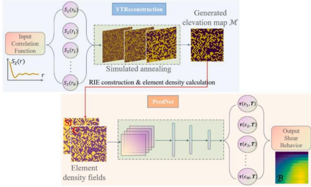
Figure 33. The overall architecture of the proposed model. Reproduced with permission. [52] Copyright 2022, Elsevier.
