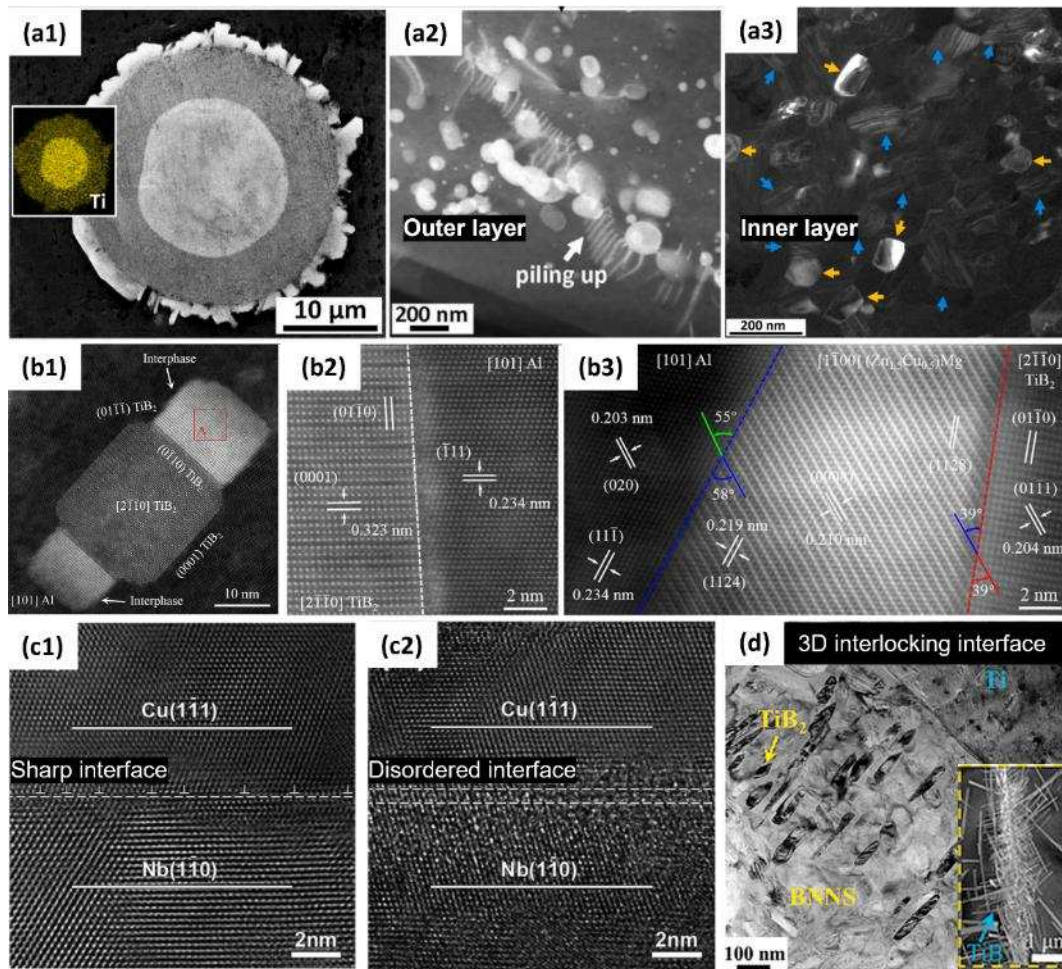
Figure 14. Some novel interfacial structures in MMCs. (a) Core-shell structure interface. Reproduced with permission. [61] Copyright 2021, Elsevier. (b) Precipitation-assisted interface. Reproduced with permission. [62] Copyright 2023, Elsevier. (c) Disordered interface. Reproduced with permission. [98] Copyright 2021, Elsevier. (d) 3D interlocking interface. Reproduced with permission. [5] Copyright 2023, Elsevier.
