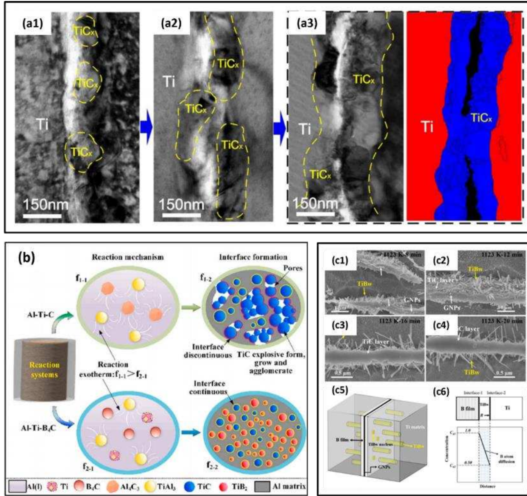
Figure 28. (a) Sequence of TEM micrographs of the in-situ TiC_x layer growth in HT 1123K samples: (a1) 120s; (a2) 300s; (a3) 600. Reproduced with permission. [191] Copyright 2021, Elsevier. (b) Schematic diagram of interface formation in the Al-Ti-C and Al-Ti-B 4 C systems, respectively. Reproduced with permission. [75] Copyright 2021, Elsevier. (c) Interfacial morphologies of TiB_w@GNPs/Ti composites after B-GNPs/Ti billets being heat treated (HT) at 1123 K for different times: (c1) 1123 K-8 min, (c2) 1123 K-12 min, (c3) 1123 K-16 min and (c4) 1123 K-20 min, (c5) illustration of the interfacial interaction between B coating and Ti matrix; (c6) reaction equation: B(\text{diffusing}) + Ti(\text{surface}) = TiB_w . Reproduced with permission. [33] Copyright 2022, Elsevier.
