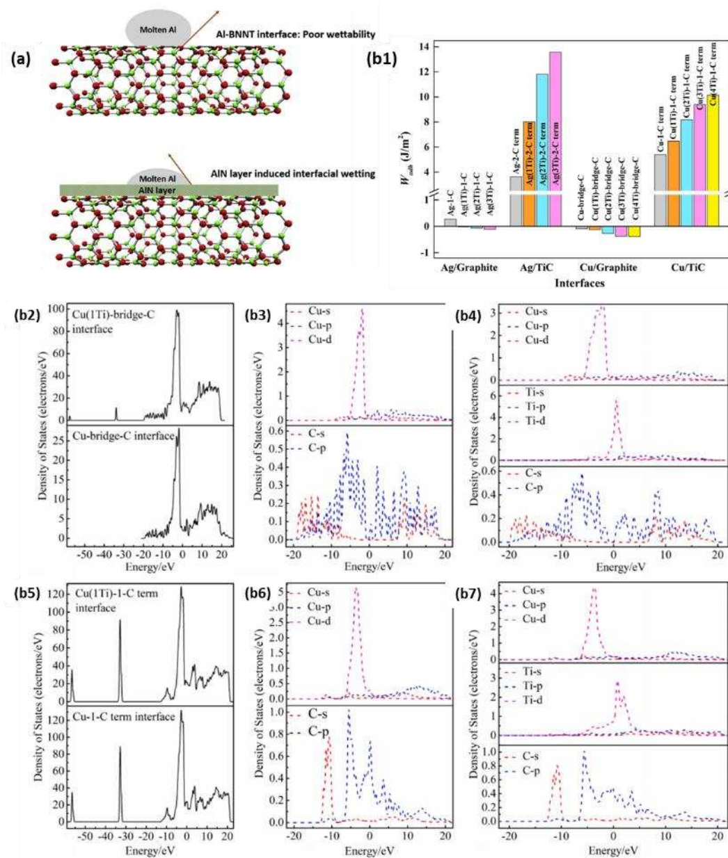
Figure 25. Interfacial reactions are effective in improving wettability. (a) Schematic representation of AlN induced wetting of BNNT by molten Al. Reproduced with permission. [185] Copyright 2017, Elsevier. (b1) Work of adhesion ( W_{ad} ) of Ag/graphite, Ag/TiC, Cu/graphite, Cu/TiC and Ti-adsorption interfaces; Density of state results of Cu/graphite and Cu/TiC interfaces. totals DOS of (b2) Cu/graphite and (b5) Cu/TiC and corresponding Ti-adsorption interfaces, PDOS results of (b3) Cu/graphite (b4) Cu(1Ti)/graphite (b6) Cu/TiC (b7) Cu(1Ti)/TiC. Reproduced with permission. [188] Copyright 2023, Elsevier.
