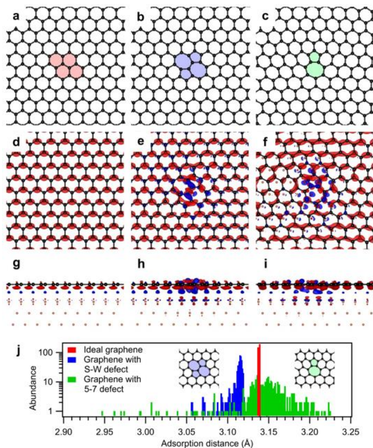
Figure 22. (a-j) Interaction of topological graphene defects with the Cu(111) surface. Reproduced with permission. [120] Copyright 2022, American Chemical Society.
