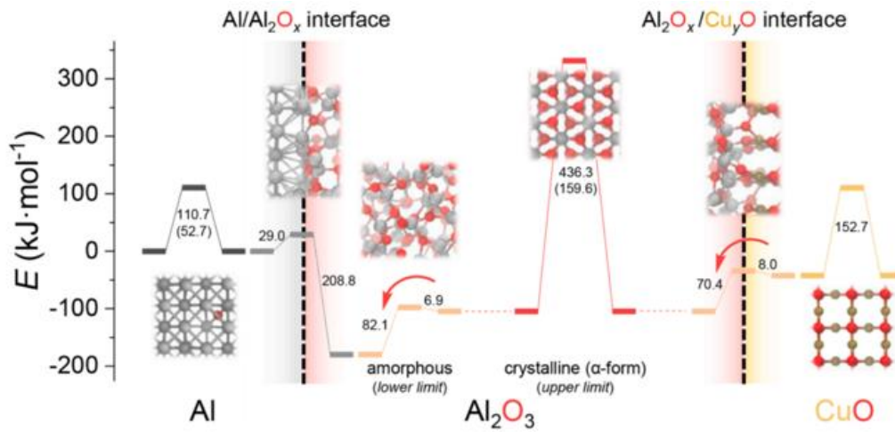
Figure 32. Barrier diagram of O migration through the Al/CuO nanolayers obtained by MD simulation. Reproduced with permission. [226] Copyright 2022, Elsevier.
