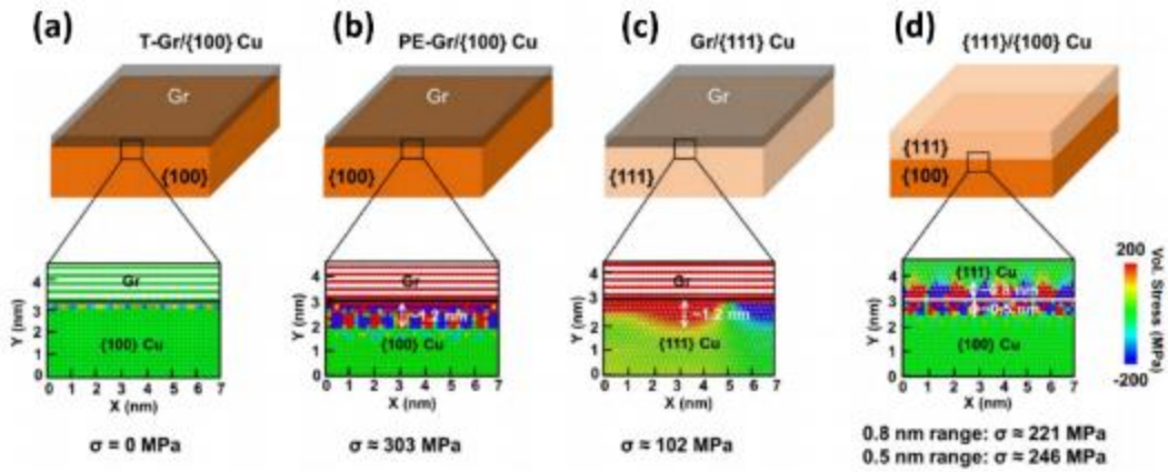
Figure 31. MD simulation results about the stress fields of the Gr/Cu interface and {111}/{100}Cu homogeneous interface. Reproduced with permission. [221] Copyright 2022, Elsevier.
