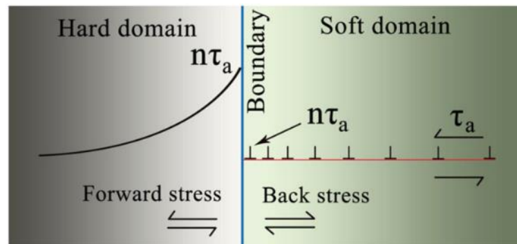
Figure 9. Schematics of a GND pile-up, inducing back stress in the soft domain, which in turn induces forward stress in the hard domain. Reproduced under terms of the CC-BY license. [86] Copyright 2019, Y. Zhu, X. Wu, published by Taylor & Francis.
