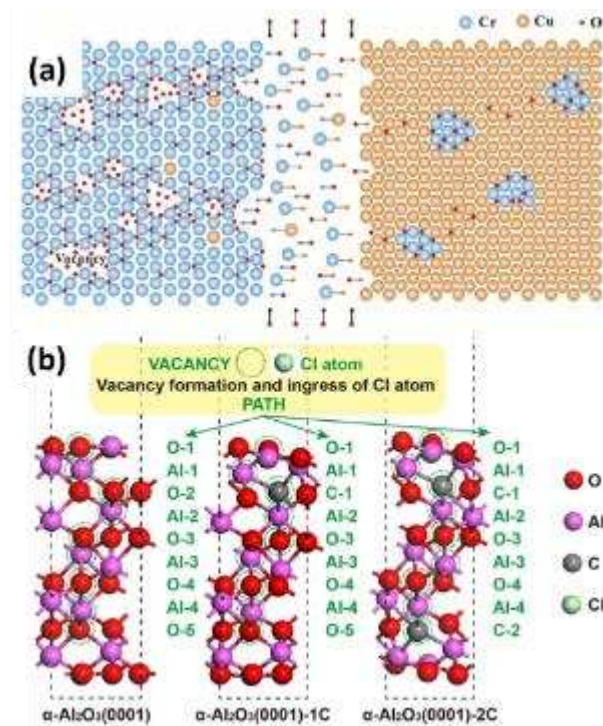
Figure 18. (a) Schematic diagram of Cu, Cr and O atoms diffusion at the Cu-Cr interface during the pressure sintering process. Reproduced with permission. [132] Copyright 2019, Elsevier. (b) Schematics of the \alpha -Al 2 O 3 (0001) slab, single-carbon-atom-doped \alpha -Al 2 O 3 (0001)-1C slab, and dual-carbon-atom-doped \alpha -Al 2 O 3 (0001)-2C slab. Reproduced with permission. [133] Copyright 2021, American Chemical Society.
