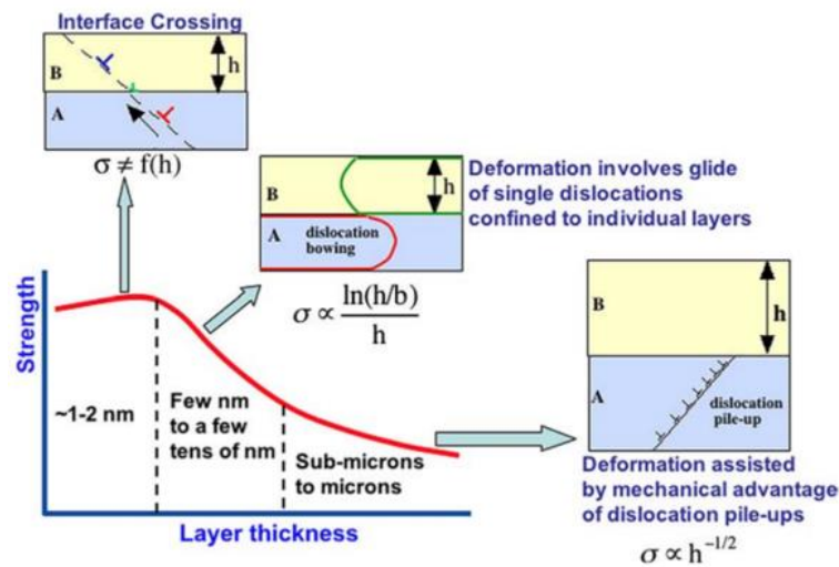
Figure 11. Schematic illustration of the dislocation mechanisms of multilayer strength operative at different length scale. Reproduced with permission. [90] Copyright 2005, Elsevier.
