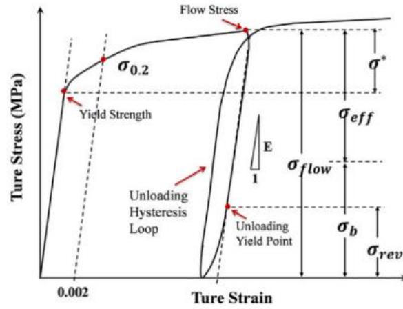
Figure 3. Schematic of hysteresis loops for characterizing the Bauschinger effect. Reproduced with permission. [63] Copyright 2019, Elsevier.
