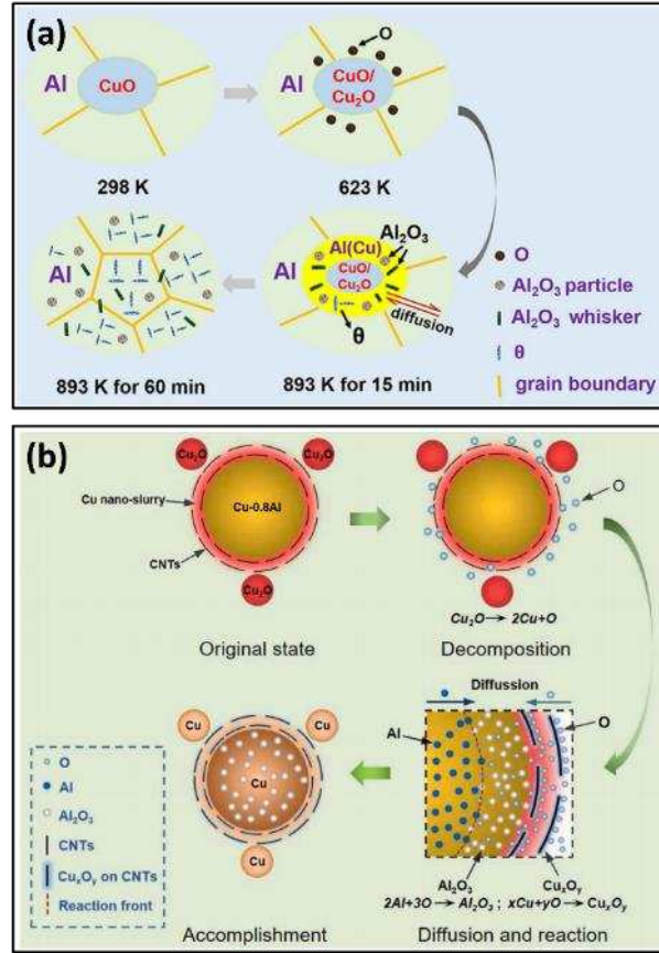
Figure 26. (a) The schematic of reaction mechanism for the Al-5CuO composite during sintering. Reproduced with permission. [164] Copyright 2021, Elsevier. (b) The schematic illustration of oxygen diffusion and in-situ solid-reaction for Cu-Al 2 O 3 -CNTs during internal oxidation. Reproduced with permission. [83] Copyright 2022, Elsevier.
