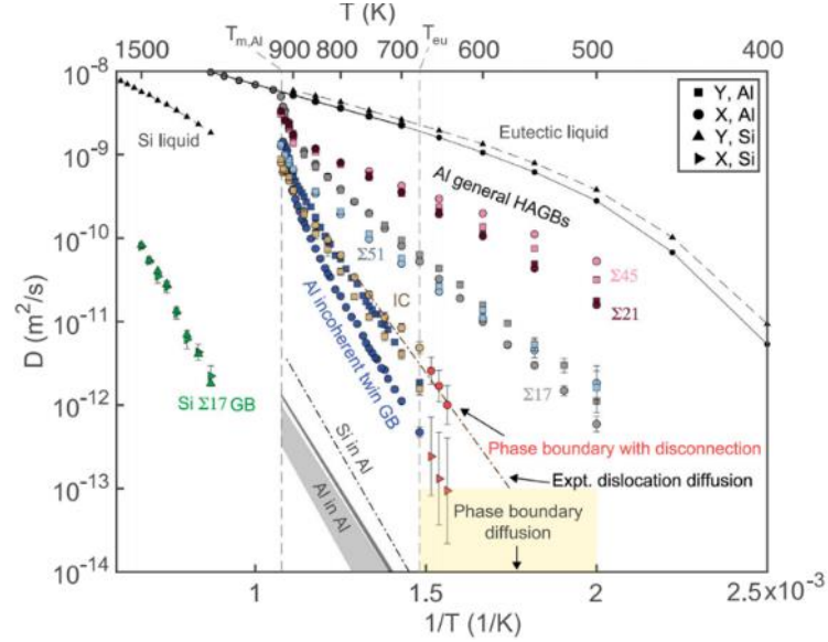
Figure 29. Arrhenius diagram of diffusion in Al, Si, and Al-Si systems. Reproduced with permission. [41] Copyright 2023, Elsevier.
