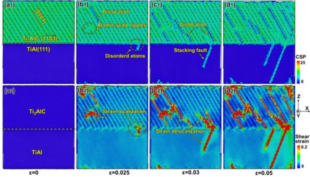
Figure 10. Defect structure and strain partitioning for \text{Ti}_2\text{AlC} ( \bar{1}\bar{1}0\bar{3} )/ \text{TiAl} (111) interfacial model at different strain. (a1, a2) \epsilon=0 ; (b1, b2) \epsilon=0.025 ; (c1, c2) \epsilon=0.03 ; (d1, d2) \epsilon=0.05 . Reproduced with permission. [4] Copyright 2023, Elsevier.
