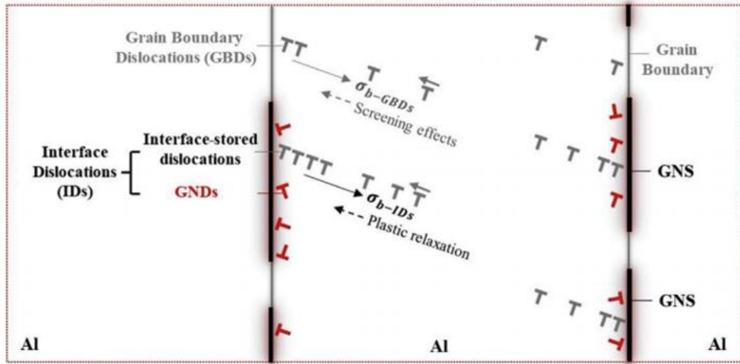
Figure 5. Illustration of the origin of forest hardening and back stress hardening induced by GNS-Al interface in GNS/Al composites. Reproduced with permission. [71] Copyright 2019, Elsevier.
