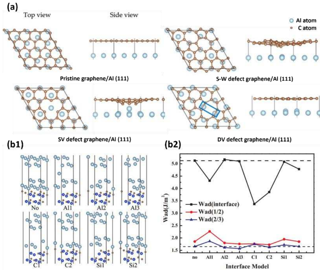
Figure 16. (a) Top views and side views of the pristine graphene, the S-W defect graphene, the SV graphene and the DV graphene on the Al (111) surface after the structural optimization. Reproduced under terms of the CC-BY license. [129] Copyright 2021, X. Zhang, S. Wang, published by MDPI. (b1) The models of tensile fracture position of the C-terminated interfaces with different point vacancy. (b2) The adhesion energy of the three interfaces at the Al side for the C-terminated interfaces. Reproduced with permission. [121] Copyright 2019, Elsevier.
