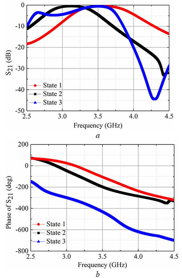
FIGURE 5 (a) Transmission amplitude and (b) transmission phase of the three states.
