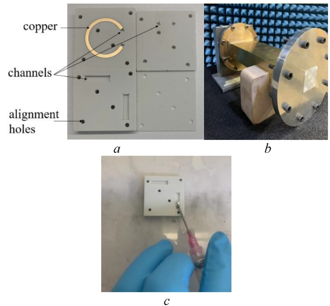
FIGURE 6 (a) The unassembled unit cell and its channels; (b) The unit cell inside at the end of waveguide; (c) The unit cell drained by a syringe.
