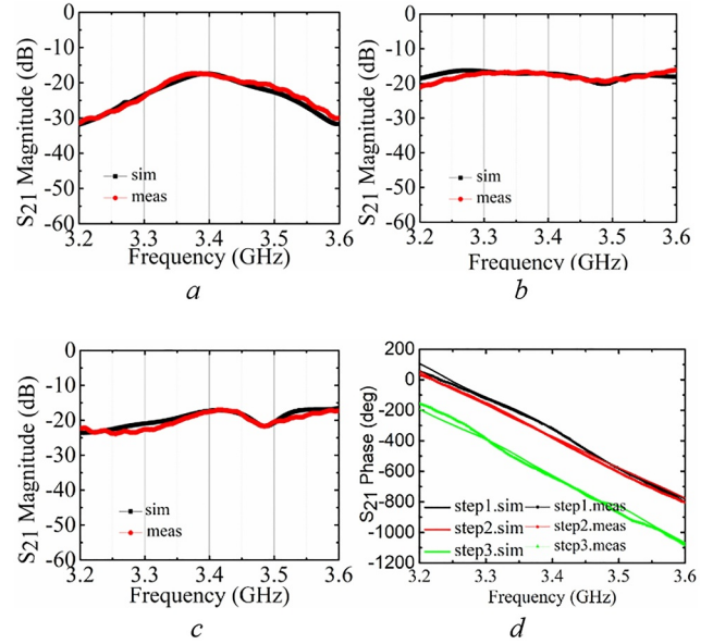
FIGURE 8 Simulated and measured transmission amplitude of the transmit-array unit cell under the measurement setup for (a) State1, (b) State2, and (c) State3. (d) Simulated and measured transmission phases of the States 1, 2, and 3 versus frequencies.
