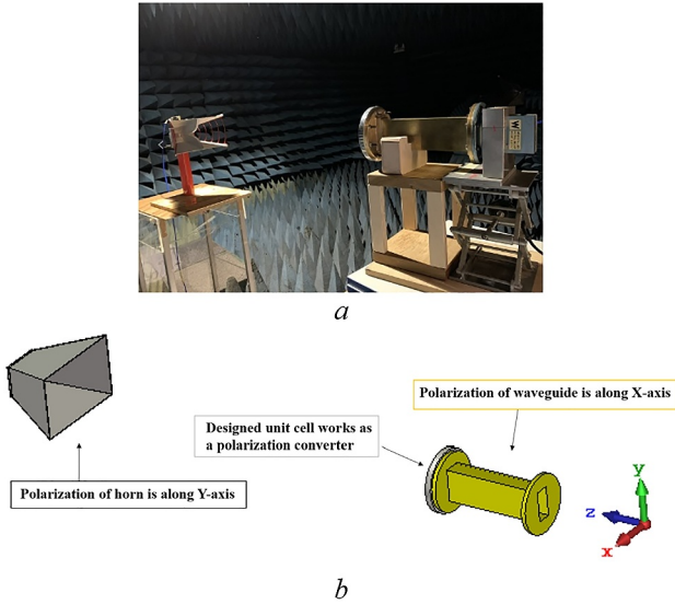
FIGURE 7 (a) The experimental setup of the open-ended waveguide; (b) The configuration of the simulation system which has the same settings as the measurement.
