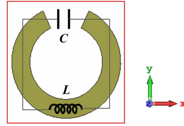
FIGURE 1 Equivalent circuit of a single split ring resonators (SRR) structure.
