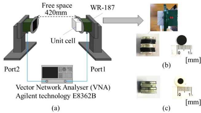
FIGURE 4 Experimental set-up (a), ferrite sample A configuration (b), and ferrite sample B configuration (c).
