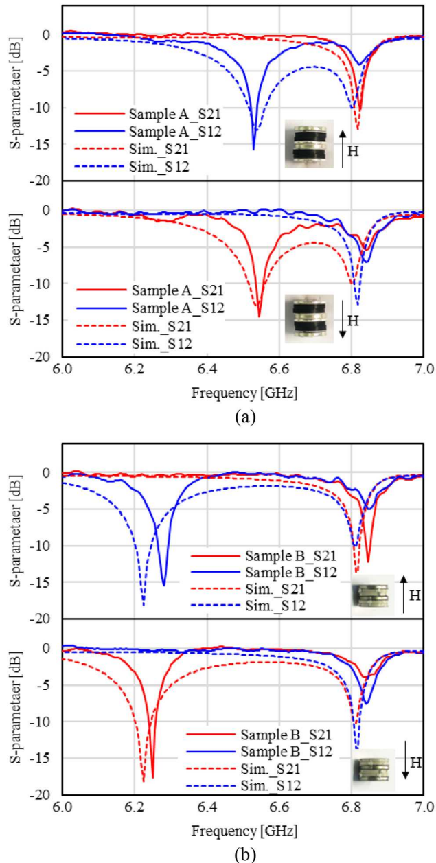
FIGURE 5 Experimental results for upward and downward magnetic fields for Sample A (a) and for Sample B (b).
