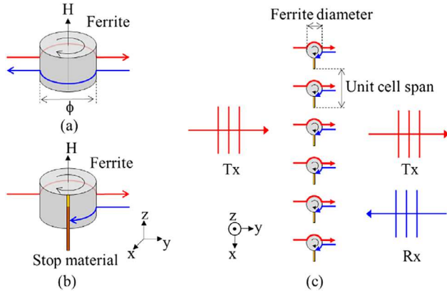
FIGURE 1 Operating principle of the proposed structure; the state of propagation in cylindrical ferrite (a), nonreciprocal structure (b), and array structure (c).
