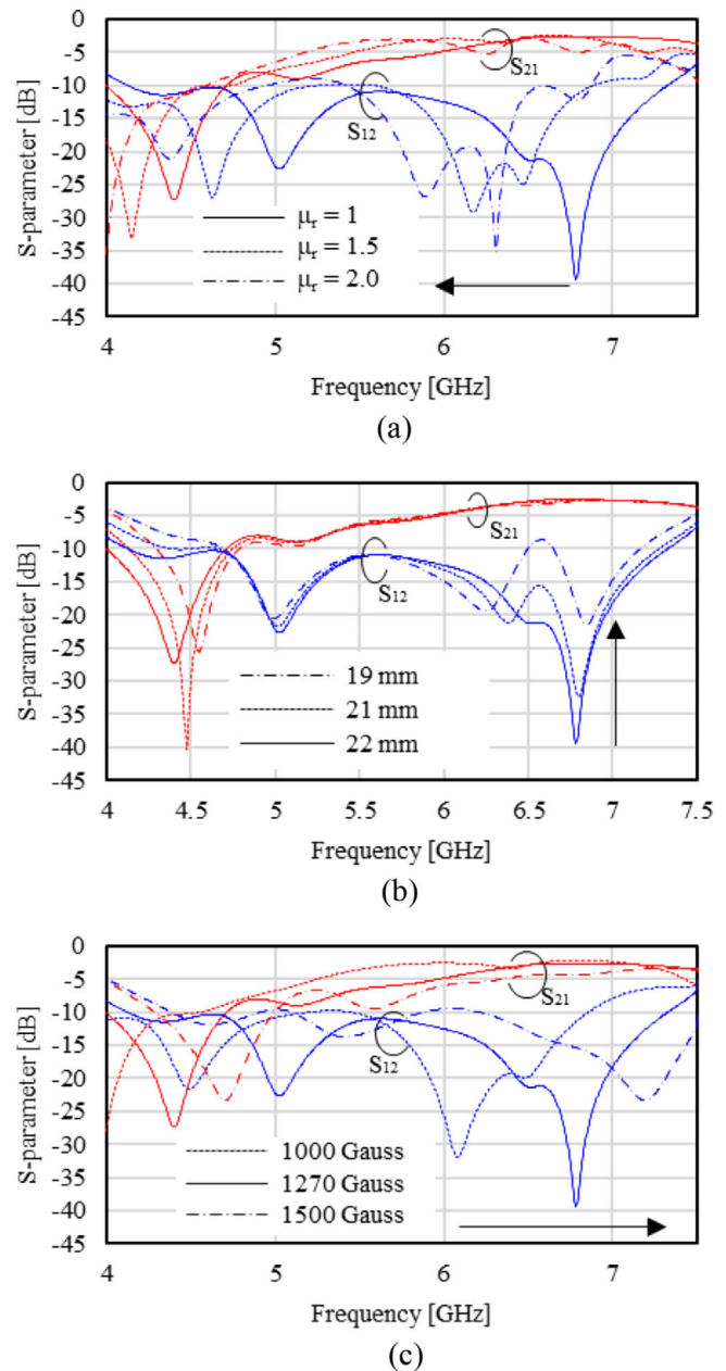
FIGURE 3 S-parameters for variations in each characteristic: (a) change in magnetic permeability, (b) change in height, and (c) change in applied magnetic field.
