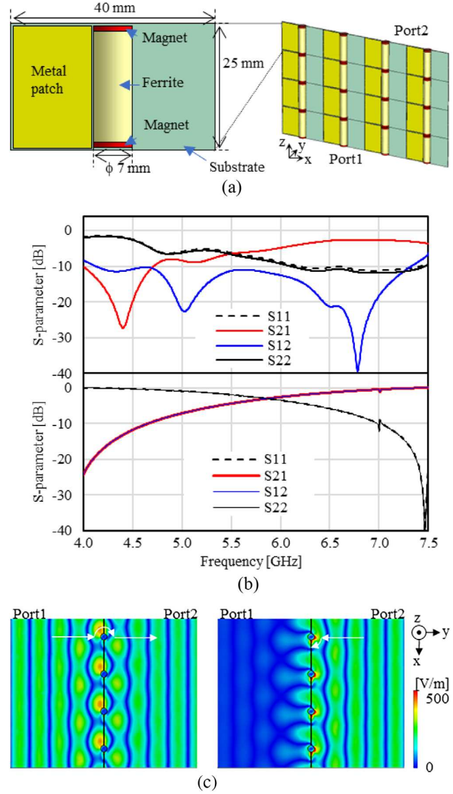
FIGURE 2 Schematic diagram of unit cell structure and infinite plane array (a), S-parameter results with ferrite and without ferrite (b) and electric field distribution diagram (c).
