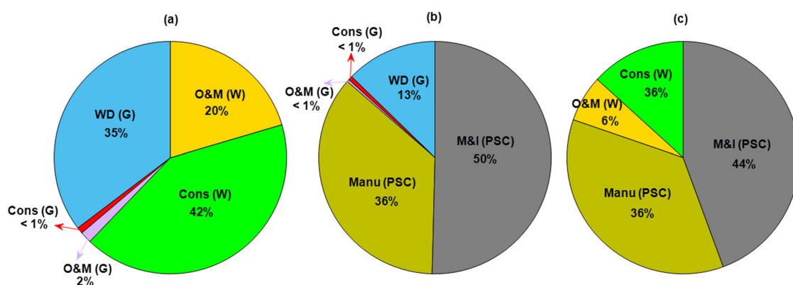
Fig. 3 | FE impact contribution of base scenarios of integrated power cycles, highlighting the contribution of different phases. These pie plots depict the percentage of FE influence of studied base scenarios for all three combined power systems, (a) the FE portion for B1, (b) the FE portion for B2, and (c) the FE portion
