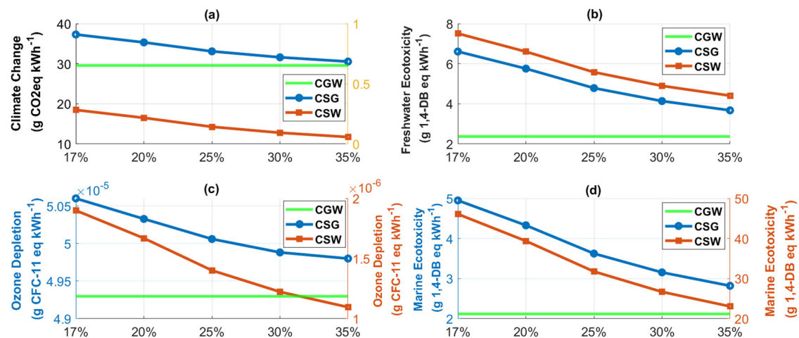
Fig. 5 | The variation of environmental impacts of four main impact categories for all scenarios and technologies assuming efficiency enhancement of PSC. These graphs illustrate the reduction in environmental impacts of impact categories considering technological improvement supposing promoting the PSC efficiency,
