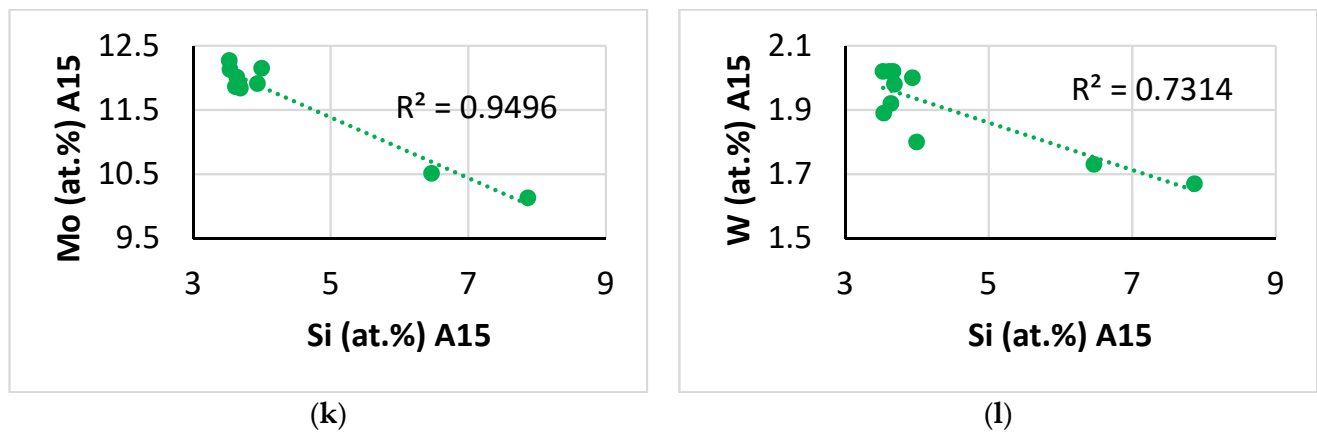
Figure 19. Relationships between solutes in A15-Nb 3 X (X = Al, Ge, Si, Sn) in NT1.1-HT200. (a) Cr versus Ti, (b) Si versus Ti, (c) Ge versus Ti, (d) Sn versus Ti, (e) Ge versus Si, (f) Sn versus Si, (g) Sn versus Ge, (h) Mo versus Ti, (i) Mo versus Ge, (j) Mo versus Sn, (k) Mo versus Si, (l) W versus Si.
