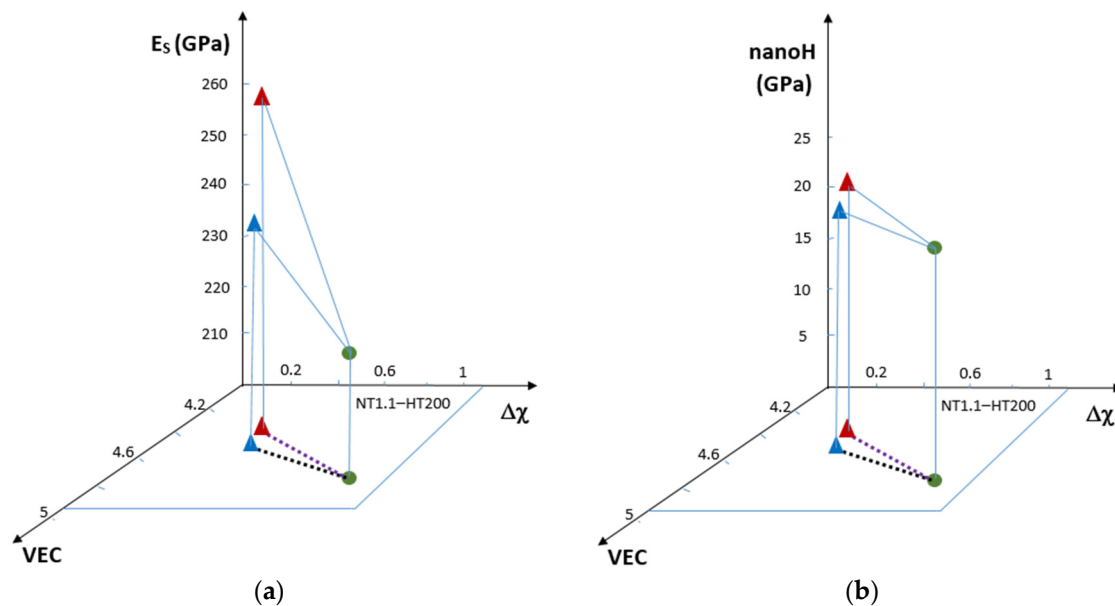
Figure 27. (a) VEC, \Delta\chi , E_s and (b) VEC, \Delta\chi , nanoH diagrams of the phases in NT1.1-HT200. For colours and shapes, see the caption of Figure 24b.
