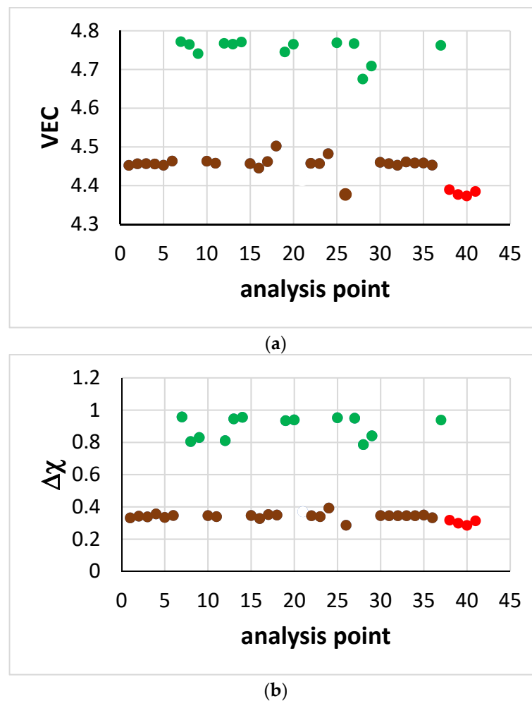
Figure 26. The parameters VEC (a) and \Delta\chi (b) of the microstructure shown in Figure 18. The analysis point numbers correspond as closely as possible to the nanoindentations. Colours as follows: brown, \beta\text{Nb}_5\text{Si}_3 ; green, A15- \text{Nb}_3\text{X} ; red, Ti-rich silicide (very dark contrast grains above points 7, 8, near 28, between 39 and 40 and below 40 in Figure 18).
