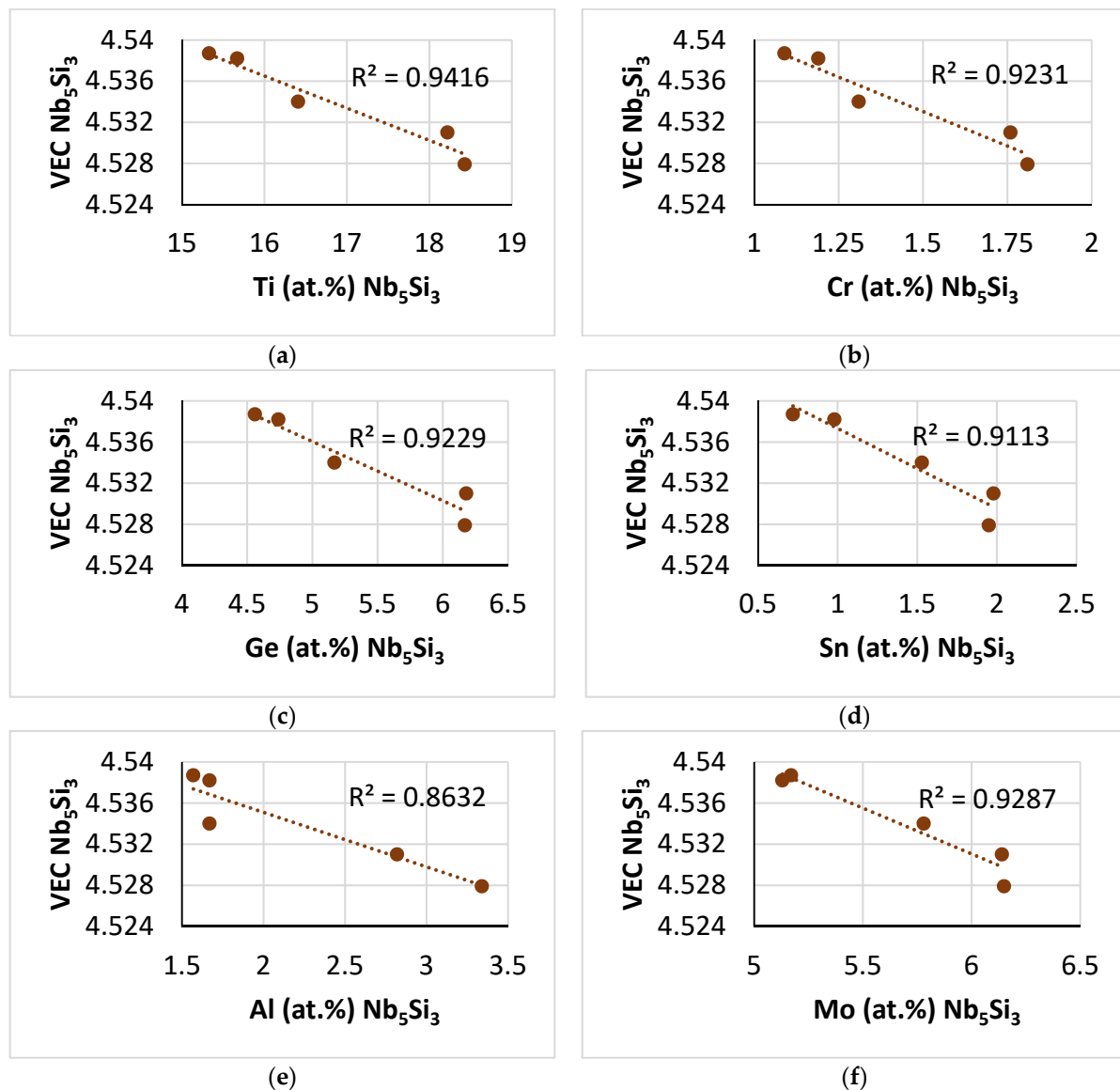
Figure 8. Relationships between the parameter VEC of \beta\text{Nb}_5\text{Si}_3 and solutes in the silicide in NT1.1–AC. (a) VEC versus Ti, (b) VEC vs. Cr, (c) VEC vs. Ge, (d) VEC vs. Sn, (e) VEC vs. Al, (f) VEC vs. Mo.
