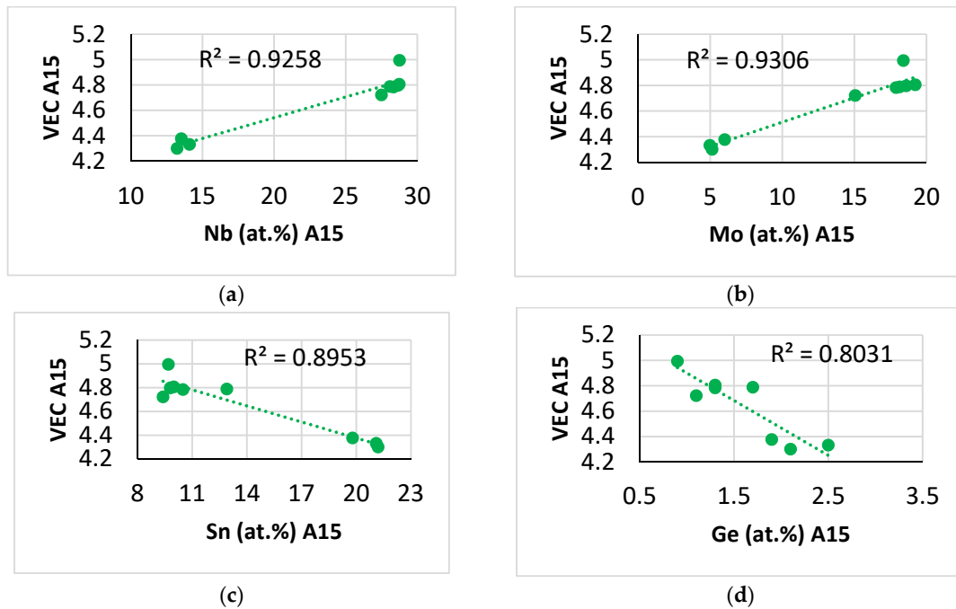
Figure 12. Relationships between the parameter VEC of A15–Nb 3 X and solutes in NT1.1–AC. (a) VEC versus Nb, (b) VEC vs. Mo, (c) VEC vs. Sn, (d) VEC vs. Ge.
