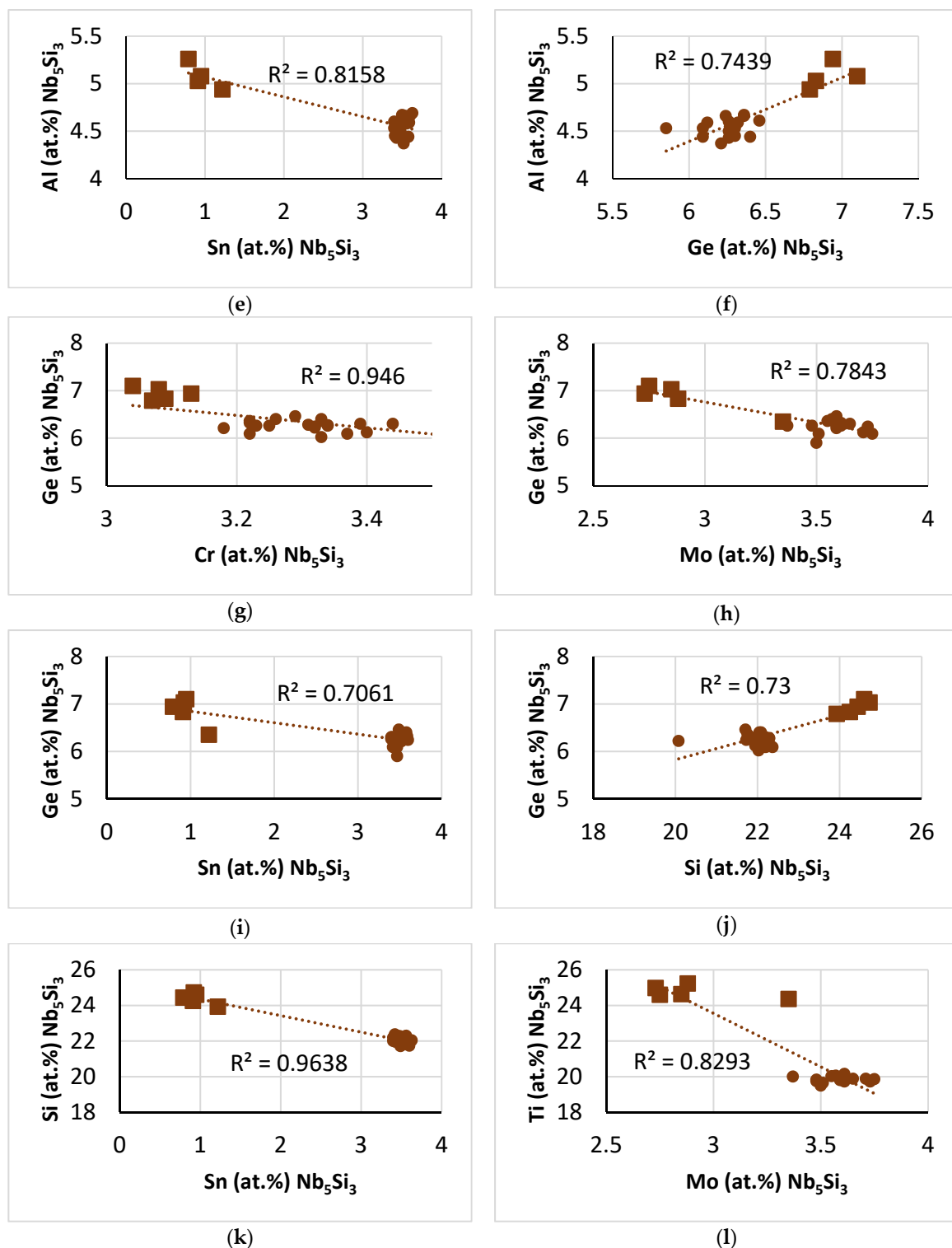
Figure 21. Relationships between solutes in \beta\text{Nb}_5\text{Si}_3 in NT1.1–HT. Squares for Ti-rich silicide. (a) Al versus Ti, (b) Al vs. Mo, (c) Al vs. Cr, (d) Al vs. Si, (e) Al vs. Sn, (f) Al vs. Ge, (g) Ge vs. Cr, (h) Ge vs. Mo, (i) Ge vs. Sn, (j) Ge vs. Si, (k) Si vs. Sn, (l) Ti vs. Mo.
