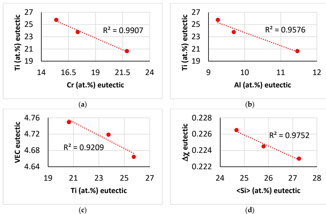
Figure 15. Relationships between solutes and between parameters and solutes for the eutectic in NT1.1–AC. (a) Ti versus Cr, (b) Ti vs. Al, (c) VEC vs. Ti, (d) \Delta\chi vs. <Si> = Al + Ge + Si + Sn.
