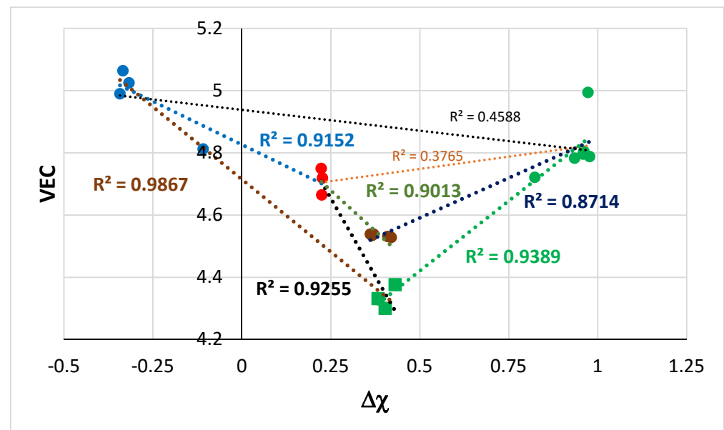
Figure 16. Map of the parameters VEC and \Delta\chi of the phases in NT1.1–AC. Colours as follows: blue, C14–NbCr 2 -based Laves phase; green, A15–Nb 3 X; brown, \beta Nb 5 Si 3 ; red, eutectic, squares for A15–Nb 3 X with high <X> value (and Ti-rich). R^2 = 0.9867 for the relationship between C14–NbCr 2 -based Laves phase and A15–Nb 3 X high <X>, R^2 = 0.9389 for A15–Nb 3 X high <X> and low <X> (see Figure 14), R^2 = 0.9255 for eutectic and A15–Nb 3 X high <X>, R^2 = 0.9152 for C14–NbCr 2 -based Laves phase and eutectic, R^2 = 0.9013 for \beta Nb 5 Si 3 and eutectic, R^2 = 0.8714 for \beta Nb 5 Si 3 and A15–Nb 3 X low <X>, R^2 = 0.4588 for C14–NbCr 2 -based Laves phase and A15–Nb 3 X low <X>, R^2 = 0.3765 for eutectic and A15–Nb 3 X low <X>. Note that the same colours were used for the data of the phases in Figures 3–16. <X> = Al + Ge + Si + Sn.
