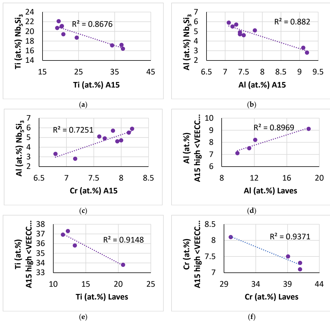
Figure 17. Relationships between solutes in \beta Nb_5Si_3 -, A15- Nb_3X - and C14 NbCr_2 -based Laves in NT1.1-AC. (a) Ti in silicide versus Ti in A15, (b) Al in silicide vs. Al in A15, (c) Al in silicide vs. Cr in A15, (d) Al in A15 high <X> vs. Al in Laves, (e) Ti in A15 high <X> vs. Ti in Laves, (f) Cr in A15 high <X> vs. Cr in Laves.
