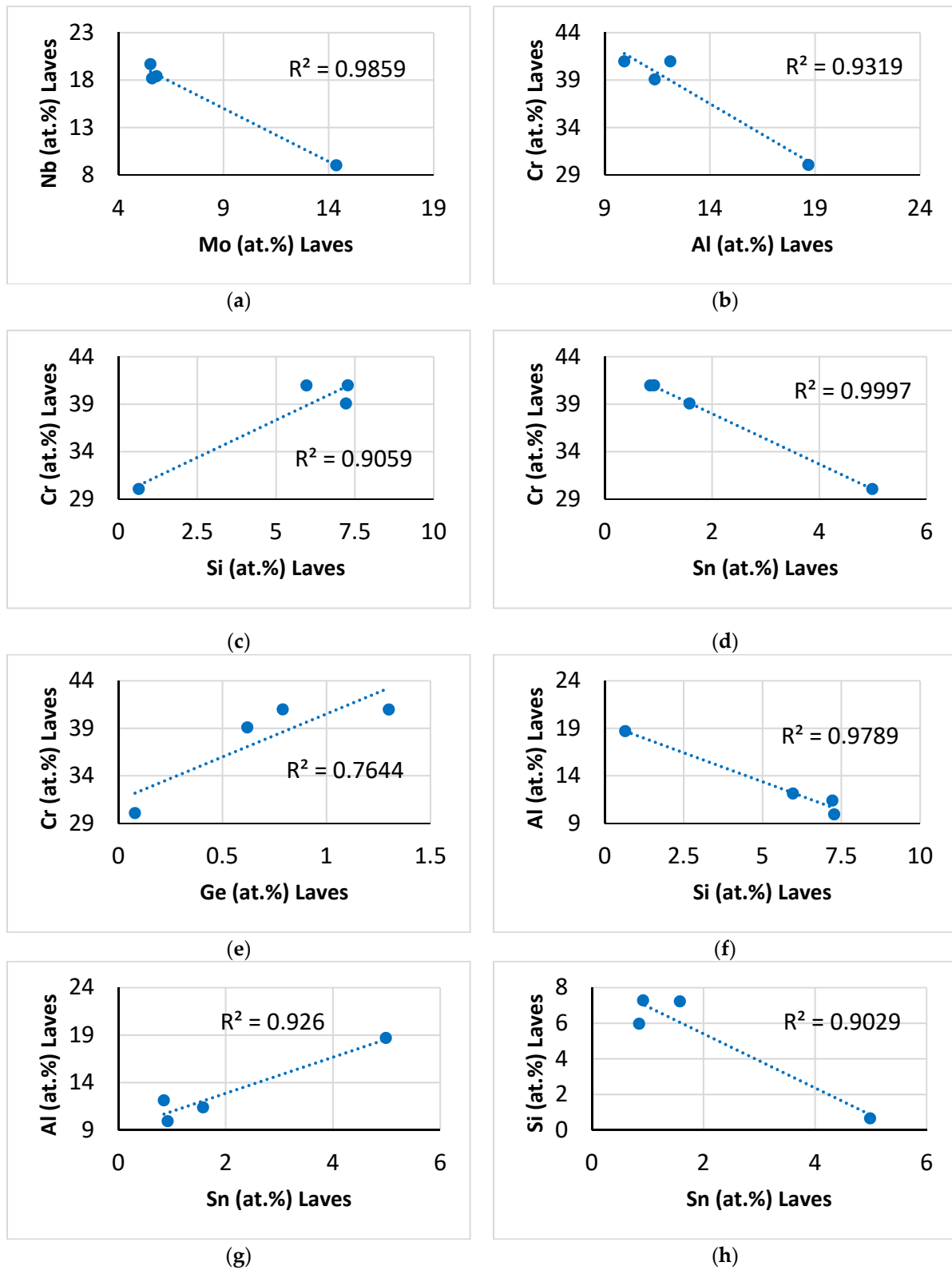
Figure 4. Relationships between solutes in the C14-NbCr 2 based Laves phase in NT1.1-AC. (a) Nb versus Mo, (b) Cr vs. Al, (c) Cr vs. Si, (d) Cr vs. Sn, (e) Cr vs. Ge, (f) Al vs. Si, (g) Al vs. Sn, (h) Si vs. Sn.
