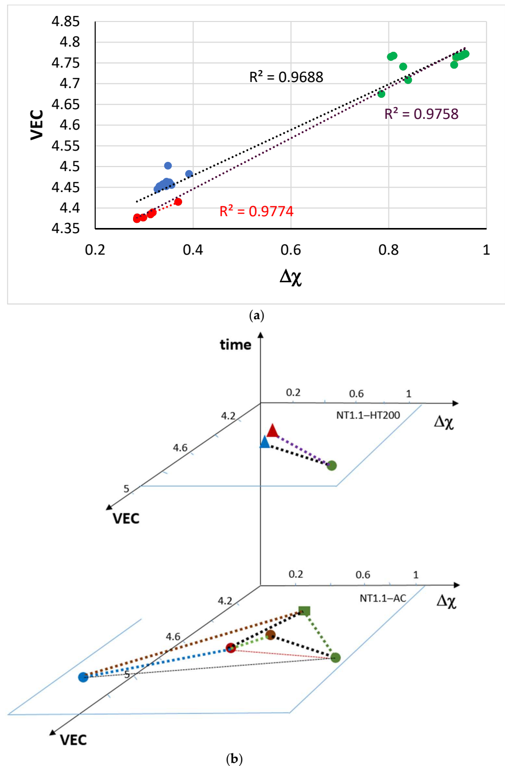
Figure 24. (a) VEC versus \Delta\chi map of the phases in NT1.1–HT200. Data are shown with filled circles. Colours as follows: green, A15–Nb 3 X; blue, \beta Nb 5 Si 3 ; red, Ti-rich silicide. Correlations as follows: R^2 = 0.9774 data for Ti-rich silicide, R^2 = 0.9758 data for A15–Nb 3 X and Ti-rich silicide, R^2 = 0.9688 data for A15–Nb 3 X and \beta Nb 5 Si 3 . (b) VEC, \Delta\chi , time diagram showing “evolution” of microstructure at T = 1500^\circ\text{C} . See Figure 16 for the NT1.1–AC. For the VEC versus \Delta\chi map of the as-cast alloy, the colours are as follows: blue for C14–NbCr 2 -based Laves phase, red for eutectic, brown for \beta Nb 5 Si 3 , green for A15–Nb 3 X. Square for A15–Nb 3 X with high \langle X \rangle . For the VEC versus \Delta\chi map of the heat-treated alloy, the triangles correspond to the silicide and the colours are as follows: green for A15–Nb 3 X, red for Ti-rich silicide and blue for \beta Nb 5 Si 3 .
