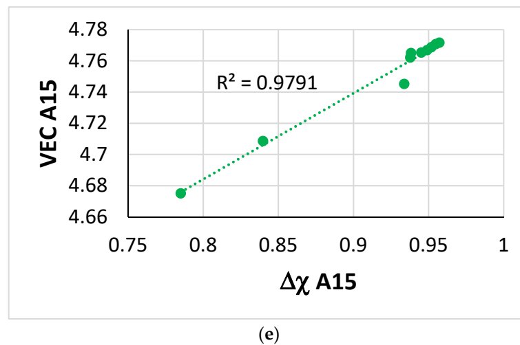
Figure 20. Relationships between the parameters VEC, \Delta\chi and solutes in A15–Nb 3 X in NT1.1–HT. (a) \Delta\chi versus Mo, (b) VEC vs. Mo, (c) \Delta\chi vs. \langle X \rangle , (d) VEC vs. \langle X \rangle , (e) VEC vs. \Delta\chi map. \langle X \rangle = \text{Al} + \text{Ge} + \text{Si} + \text{Sn} .
