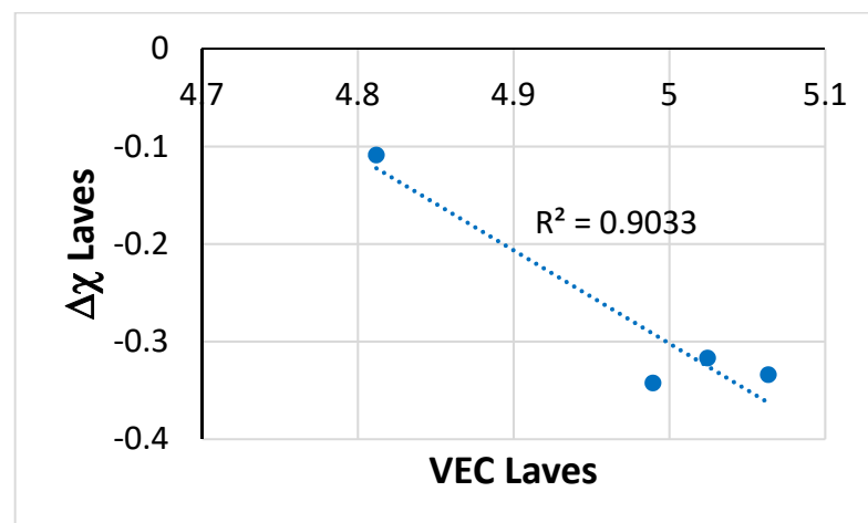
Figure 6. Map of the parameters \Delta\chi and VEC of the C14–NbCr 2 -based Laves phase in NT1.1–AC.
