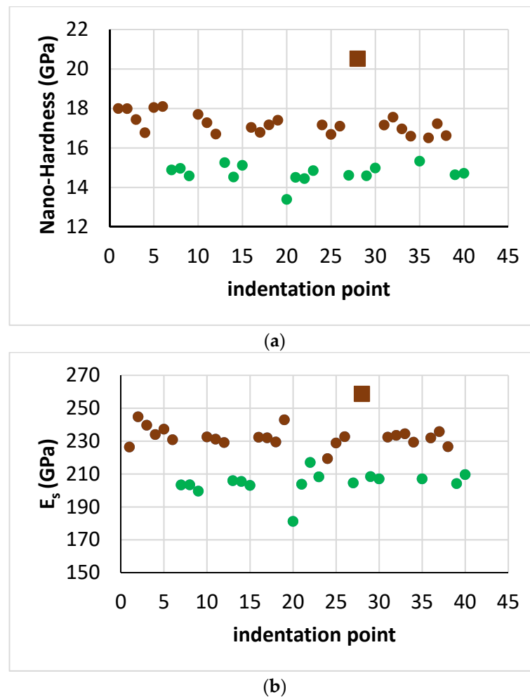
Figure 25. (a) Nano-hardness and (b) Young's modulus data for the microstructure shown in Figure 18. Colours as follows: brown— \beta\text{Nb}_5\text{Si}_3 , green— \text{A15-Nb}_3\text{X} , square for Ti-rich silicide (indentation point 28 in Figure 18).
