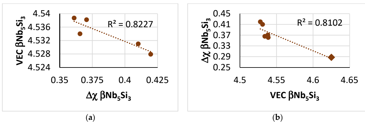
Figure 10. Maps of the parameters VEC and \Delta\chi of the alloyed \beta\text{Nb}_5\text{Si}_3 in NT1.1–AC. (a) VEC versus \Delta\chi , (b) \Delta\chi vs. VEC with data (diamond) for the binary (unalloyed) \beta\text{Nb}_5\text{Si}_3 .
