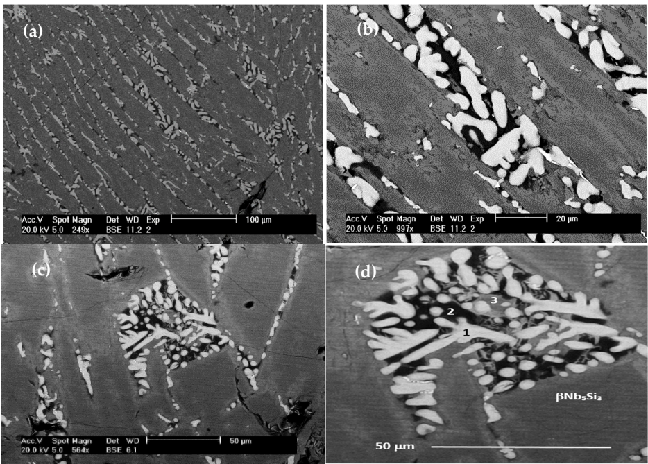
Figure 2. Back scatter electron images of the microstructure of NT1.1-AC. (a,b) show low and higher magnification images of the microstructure, where the grey phase is the \beta\text{Nb}_5\text{Si}_3 , the dark phase is the C14-NbCr 2 -based Laves and the brighter phase is the A15-Nb 3 X, (c) shows microstructure with eutectic and (d) shows the magnified eutectic in (c), where 1 = A15-Nb 3 X low <X> (<X> = Al + Ge + Si + Sn), 2 = Laves phase, 3 = A15-Nb 3 X high <X>. In (d), the very thin and bright contrast phase between A15-Nb 3 X low <X> grains in the bottom left-hand corner of the image is hafnia. Average values for 1, 2 and 3 are as follows: the A15-Nb 3 X low <X> had <X> = 21.9 at.%, Ti = 19.8 at.%, Ge + Sn = 11 at.%, Sn/Ge = 8, Mo + W = 21.5 at.%, the Laves phase had <Cr> = 58.9 at.%, Ti = 12.4 at.%, Ge + Sn = 2.8 at.%, Al + Cr = 50.8 at.%, Mo + W = 7.2 at.%, and the A15-Nb 3 X high <X> had <X> = 35 at.%, Ti = 34.4 at.%, Ge + Sn = 21.4 at.%, Mo + W = 5.8 at.%, Sn/Ge = 9.6. <Cr> = Al + Cr + Ge + Si.
