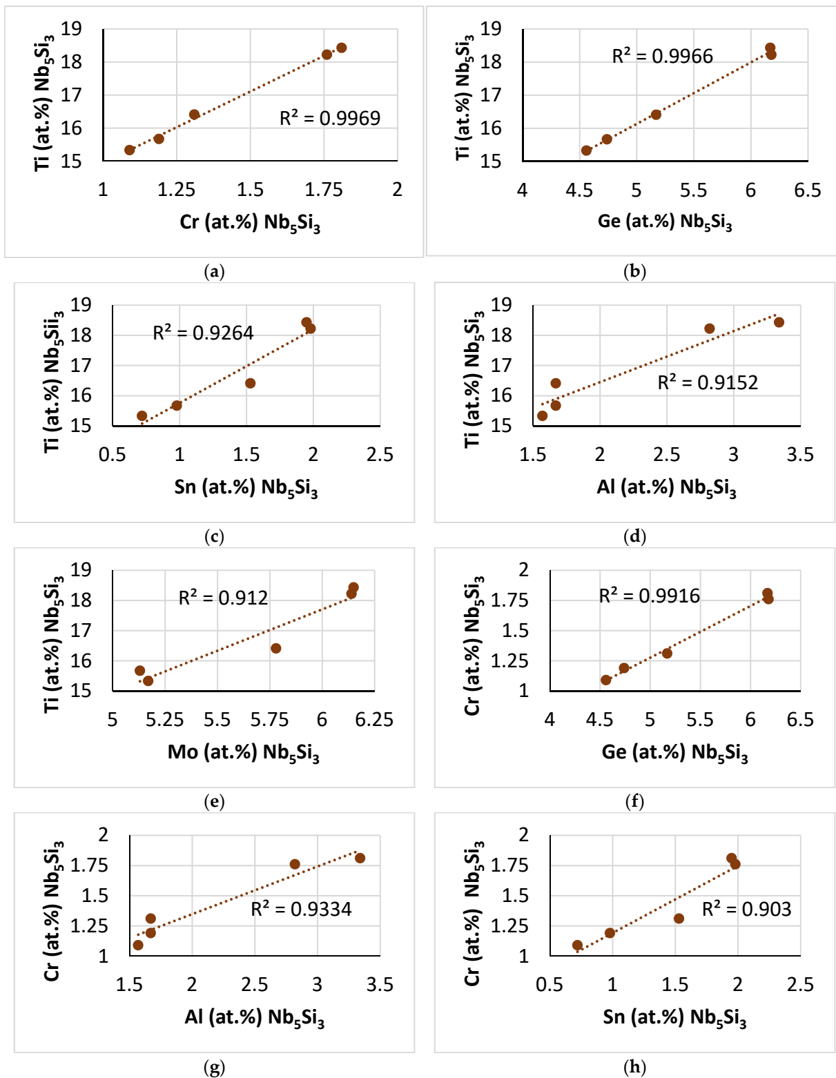
Figure 7. Relationships between solutes in \beta\text{Nb}_5\text{Si}_3 in NT1.1-AC. (a) Ti versus Cr, (b) Ti vs. Ge, (c) Ti vs. Sn, (d) Ti vs. Al, (e) Ti vs. Mo, (f) Cr vs. Ge, (g) Cr vs. Al, (h) Cr vs. Sn.
