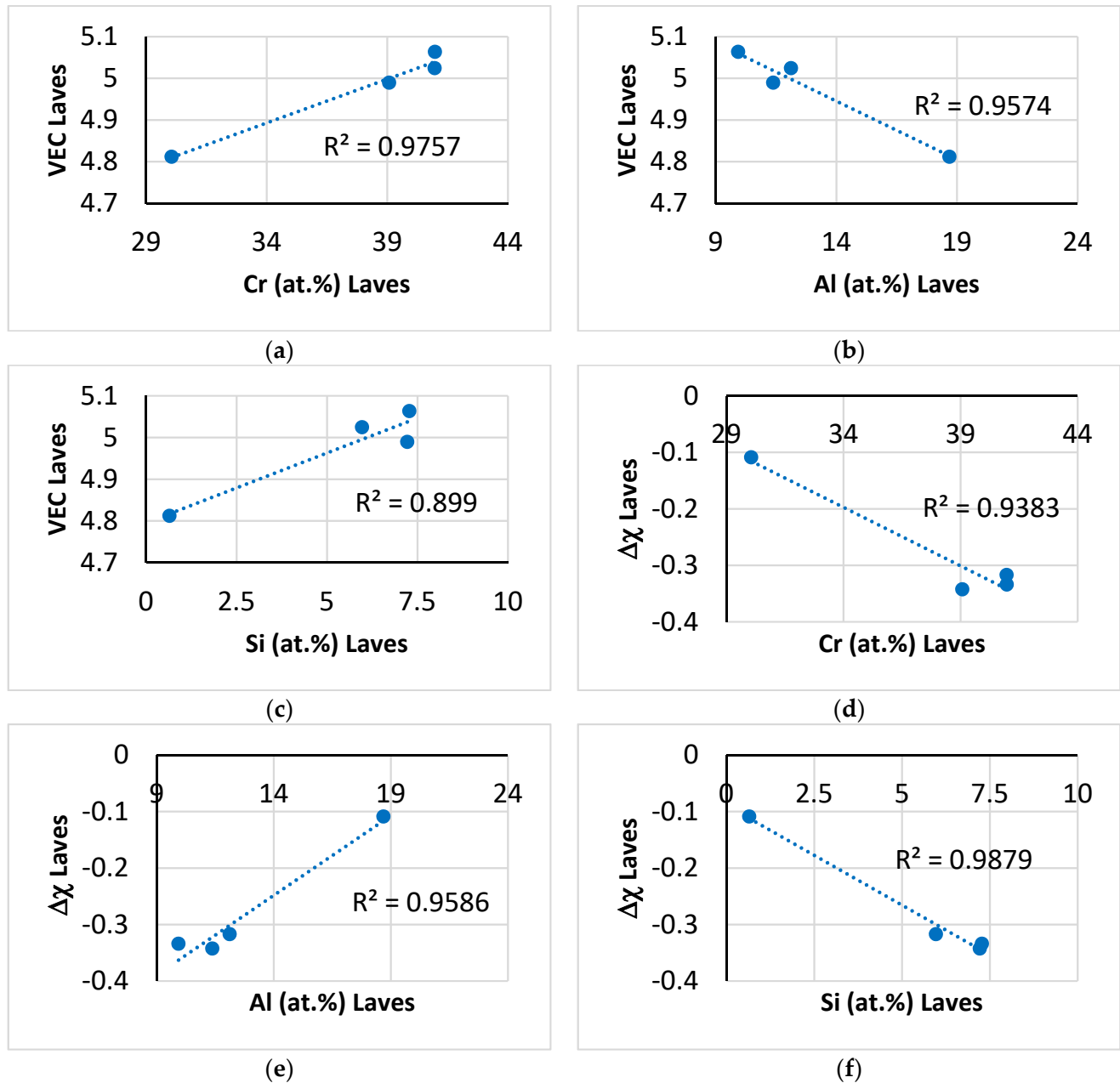
Figure 5. Relationships between the solutes Al, Cr and Si and the parameters VEC and \Delta\chi in the C14–NbCr 2 -based Laves phase in NT1.1–AC. (a) VEC versus Cr, (b) VEC vs. Al, (c) VEC vs. Si, (d) \Delta\chi vs. Cr, (e) \Delta\chi vs. Al, (f) \Delta\chi vs. Si.
