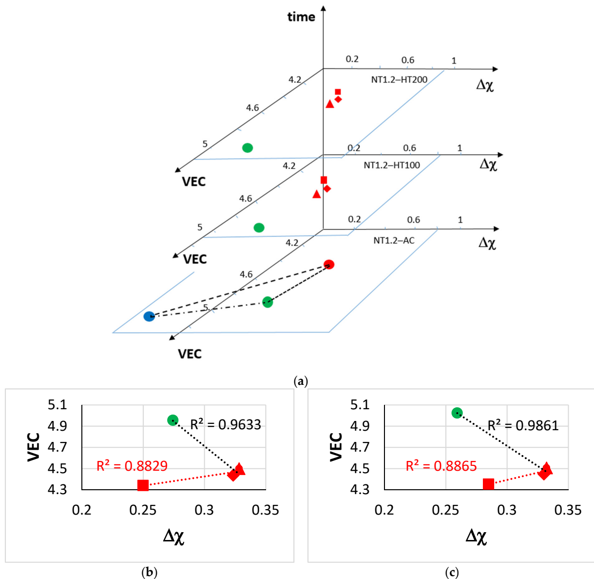
Figure 28. (a) VEC, \Delta\chi , time diagram of the alloy NT1.2 showing the “evolution” of microstructure at 1500 °C. Colours as follows: blue C14–NbCr 2 Laves phase, green A2 solid solution, red Nb 5 Si 3 silicide. (b,c) VEC versus \Delta\chi maps of phases in NT1.2–HT100 and NT1.2–HT200, respectively. Triangle for the “core” silicide, diamond for the “boundary” silicide, square for the Ti-rich silicide, see text and [46]. (b) R^2 = 0.9633 for A2 solid solution and “core” and “boundary” silicide, and R^2 = 0.8829 for “core”, “boundary” and Ti-rich silicide. (c) R^2 = 0.9861 for A2 solid solution and “core” and “boundary” silicide, and R^2 = 0.8865 for “core”, “boundary” and Ti-rich silicide.
