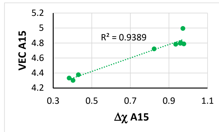
Figure 14. Map of the parameters VEC and \Delta\chi of A15–Nb 3 X in NT1.1–AC.
