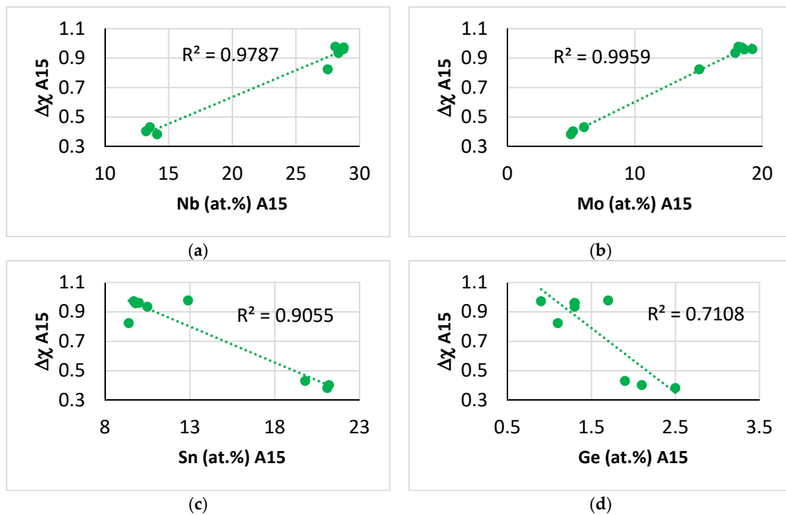
Figure 13. Relationships between the parameter \Delta\chi of A15–Nb 3 X and solutes in NT1.1–AC. (a) \Delta\chi versus Nb, (b) \Delta\chi vs. Mo, (c) \Delta\chi vs. Sn, (d) \Delta\chi vs. Ge.
