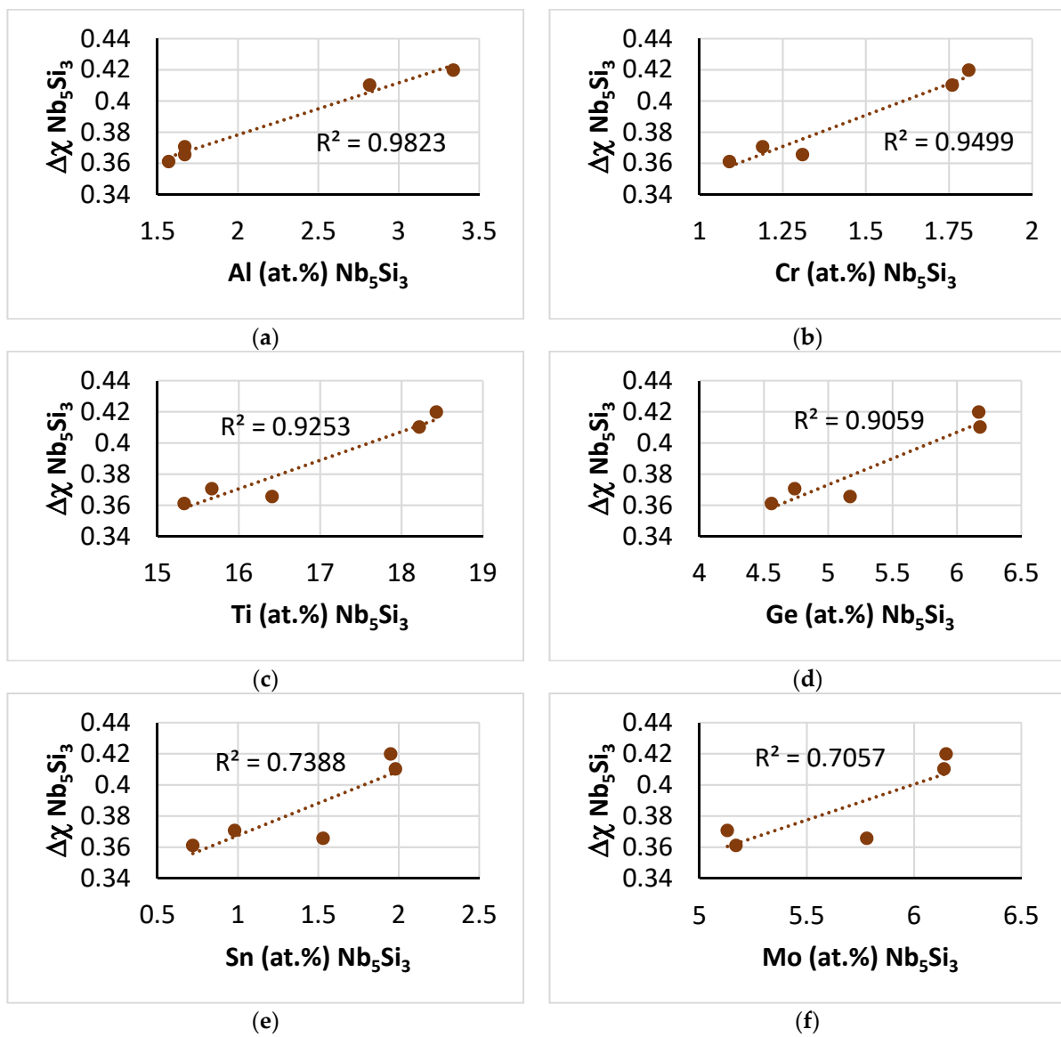
Figure 9. Relationships between the parameter \Delta\chi of \beta\text{Nb}_5\text{Si}_3 and solutes in the silicide in NT1.1–AC. (a) \Delta\chi versus Al, (b) \Delta\chi vs. Cr, (c) \Delta\chi vs. Ti, (d) \Delta\chi vs. Ge, (e) \Delta\chi vs. Sn, (f) \Delta\chi vs. Mo.
