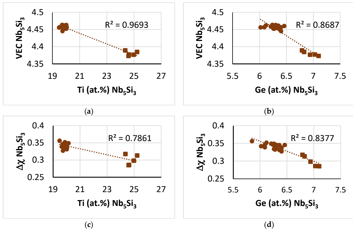
Figure 22. Relationships between the parameters VEC and \Delta\chi and solutes in \text{Nb}_5\text{Si}_3 in NT1.1-HT. Squares for Ti-rich silicide. (a) VEC versus Ti, (b) VEC vs. Ge, (c) \Delta\chi vs. Ti, (d) \Delta\chi vs. Ge.
