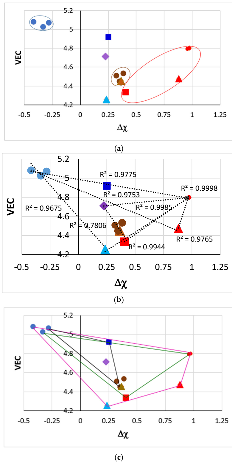
Figure 29. (a) VEC versus \Delta\chi map of phases in the as-cast RCCAs alloys JZ5, NT1.1 and NT1.2 with Al, Cr, Ge, Hf, Mo, Nb, Si, Sn, Ti, W. Shapes and colours as follows: blue filled circles C14-NbCr 2 -based Laves phase, blue square A2 solid solution, light blue triangle TM 5 Sn 2 X, purple diamond eutectic of C14-NbCr 2 -based Laves phase, A15-Nb 3 X low \langle X \rangle and A15-Nb 3 X high \langle X \rangle where \langle X \rangle = \text{Al} + \text{Ge} + \text{Si} + \text{Sn} , brown filled circles Nb 5 Si 3 , brown triangle Ti-rich Nb 5 Si 3 , red square A15-Nb 3 X high \langle X \rangle , red circles A15-Nb 3 X low \langle X \rangle , red triangle Ti-rich A15-Nb 3 X. Blue ellipse for C14-NbCr 2 -based Laves phase "territory", brown ellipse for Nb 5 Si 3 "territory" and red ellipse for
