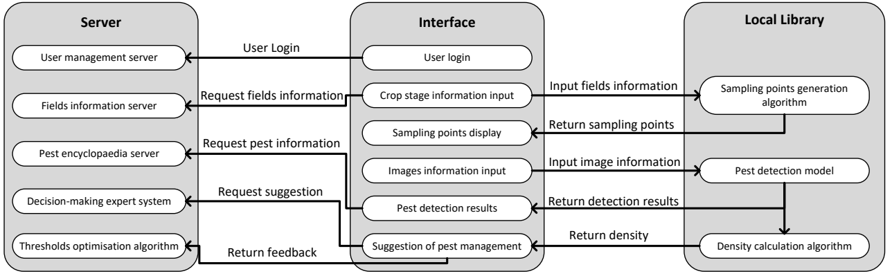
Figure 2: Interaction between server, interface and local library
