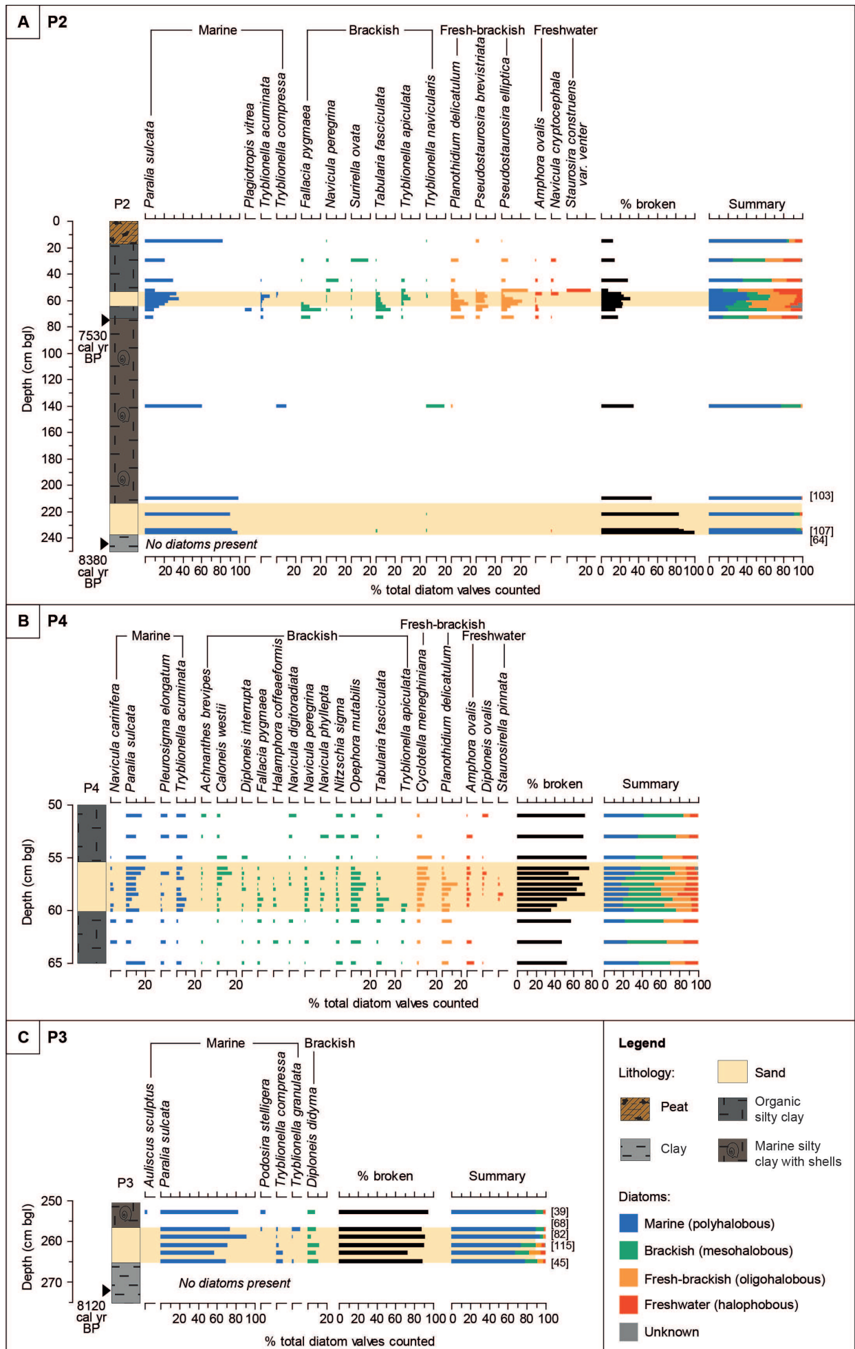
Figure 4 | Diatom assemblages of cores (A) P2, (B) P4 and (C) P3, showing species constituting >5% of any one sample. Where a minimum count of 250 valves could not be achieved from a sample, the total valves counted are indicated in brackets on the far right of the plot. Median calibrated radiocarbon ages are shown.
