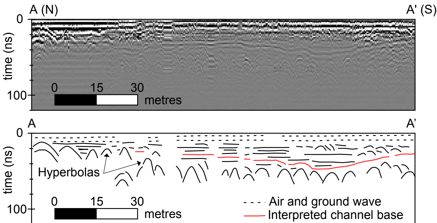
Figure 5 | Uninterpreted (top panel) and line interpretation (bottom panel) of GPR line 1.
