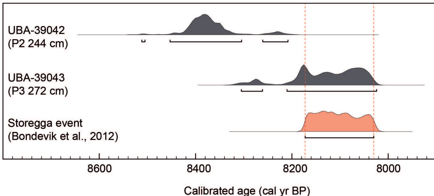
Figure 7 | Probability density functions for calibrated ages of samples below the lower sand layers in P2 and P3, which are compared to the age of the Storegga slide previously reported by Bondevik et al. (2012), and recalibrated here using IntCal20 in OxCal 4.4 (Bronk Ramsey, 2009; Reimer et al., 2020).
