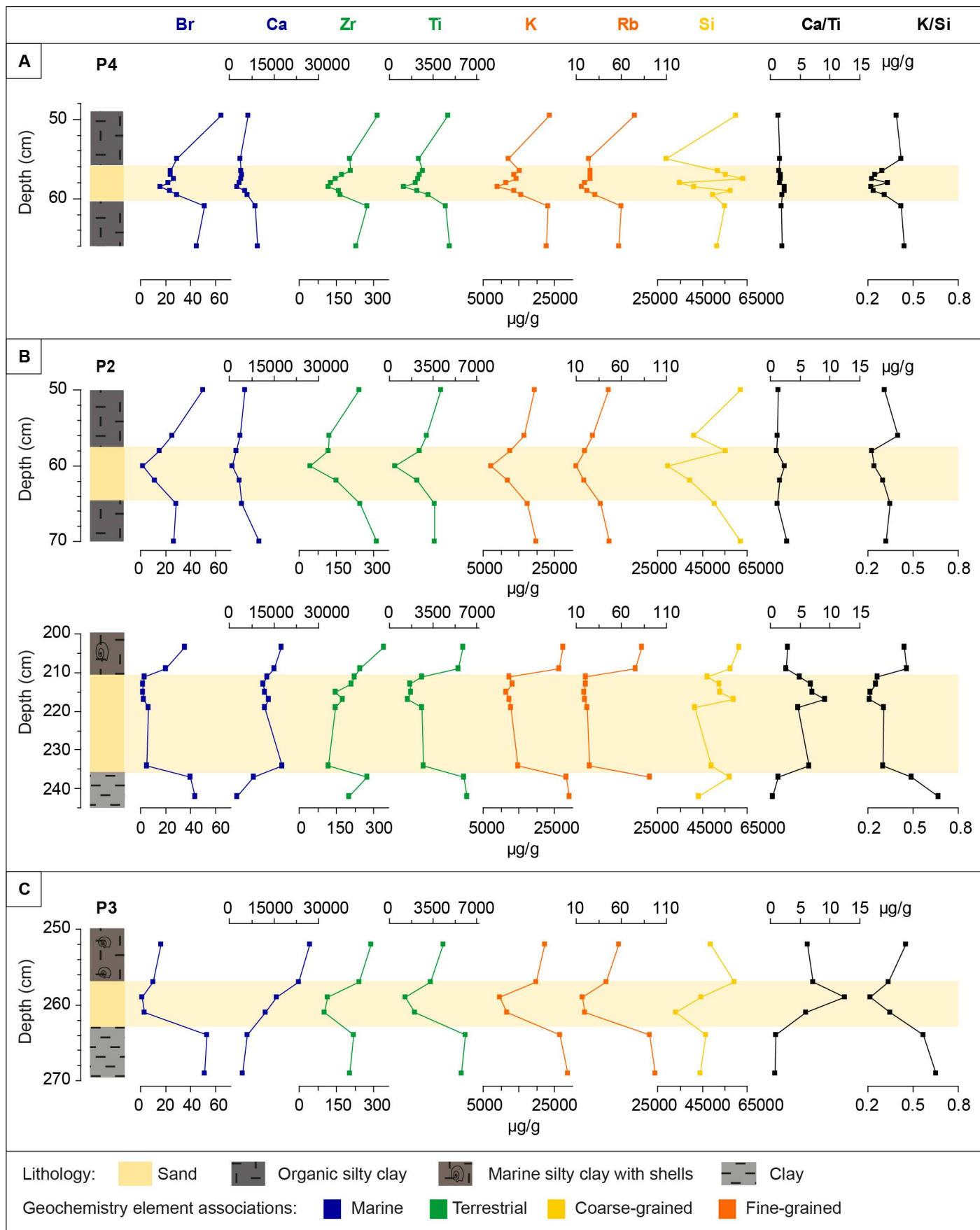
Figure 3 | Geochemical composition of the (A) upper sand in P4, (B) upper and lower sands in P2, and (C) lower sand in P3. The unit of measurement for all plots is \mu\text{g/g} .
