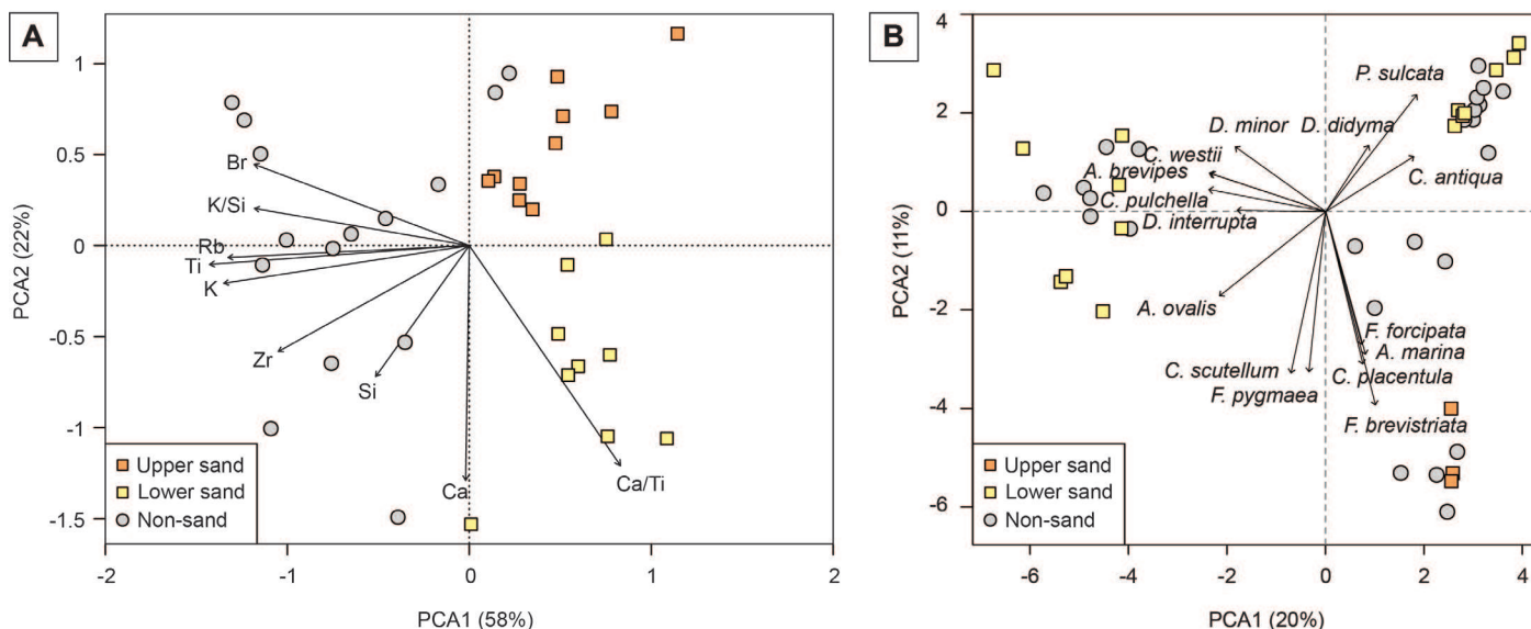
Figure 6 | Principal component analysis of (A) geochemical data from P4 and (B) diatom data from P2.
