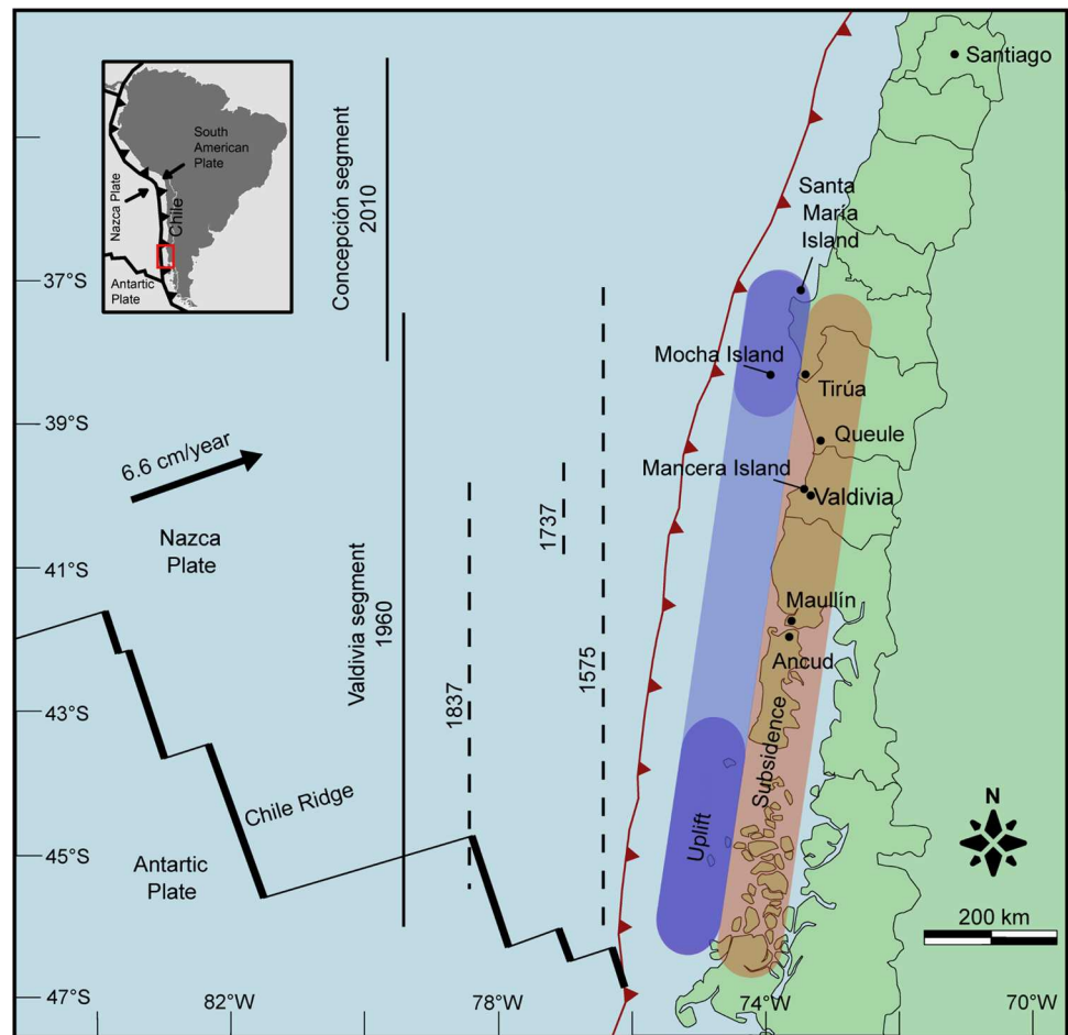
Fig. 1 Tectonic context and extent of the subduction zone's historical ruptures in south-central Chile. Solid lines show earthquake ruptures from 1960 and 2010. Dashed lines show estimated rupture lengths based on historical reports. Spatial distribution of uplift (blueish shaded areas) and subsidence (redish shaded areas) zones during the 1960 earthquake are also shown. Modified from Ely et al. (2014) and Garrett et al. (2015)
