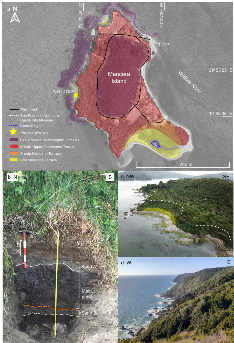
Fig. 8 Paleoseismic site of Mancera Island. a) Aerial image of Mancera Island in the Los Ríos Region, showing the location of the paleoseismic site. b) Stratigraphic profile of the paleoseismic site of Mancera Island, where solid white lines indicate sharp lower contact of sands A and B. Solid orange line indicates lower contact of the main peat. c) Western beach on Mancera Island where the white dotted line marks the upper terrace level, and the yellow shaded area indicates the surface of the lower terrace. d) Valdivian Rainforest in the Punta Curiñanco Protected Coastal Area
