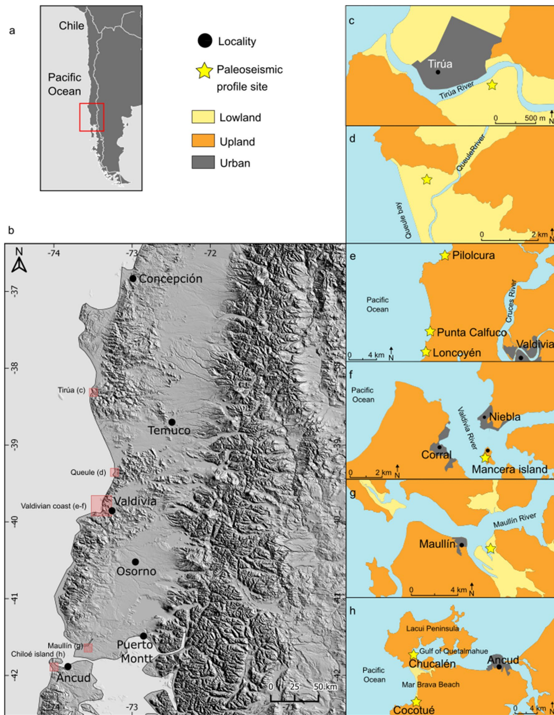
Fig. 4 a) Map of southern South America and Chile showing the study area with the red rectangle, together with symbols and legend used in figures c-h; b) Digital elevation model (DEM) image of
