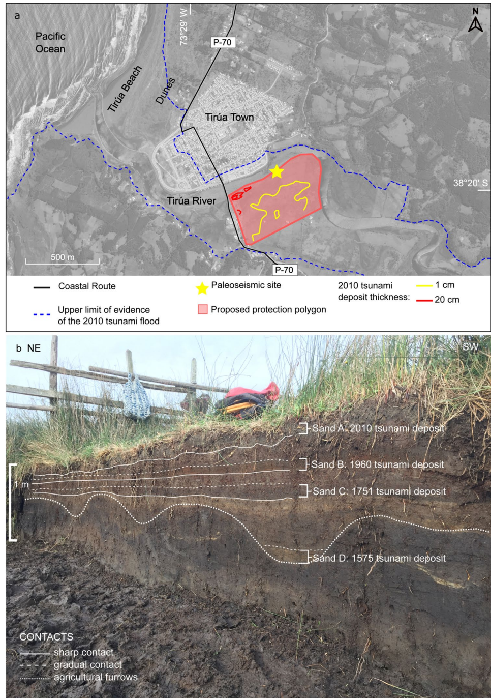
Fig. 5 Paleoseismic site of Tirúa. a) Aerial image of Tirúa paleoseismic site, Biobío Region. b) Tirúa riverbank where layers A, B, C and D represent sand deposits left by tsunamis in the last 600 years
