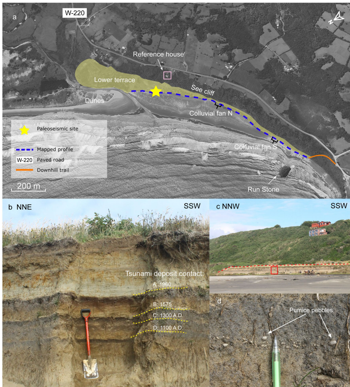
Fig. 11 Paleoseismic site of Cocotué a) Aerial image of Cocotué paleoseismic site, Los Lagos Region. b) Section of the stratigraphic profile of the lower Cocotué marine terrace where the dotted yellow line indicates the sharp lower contacts produced by the 4 earthquakes and tsunami events described by Cisternas et al. (2017a, b). c) Lower
