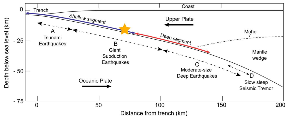
Fig. 2 Earthquake rupture domains in subduction zones (domains A, B, C and D) adapted from Lay et al. (2012). Also shown are the shallow and deep segments, and the estimated depth of the 1960 great earthquake rupture (yellow star) adapted from Moreno et al. (2018)
