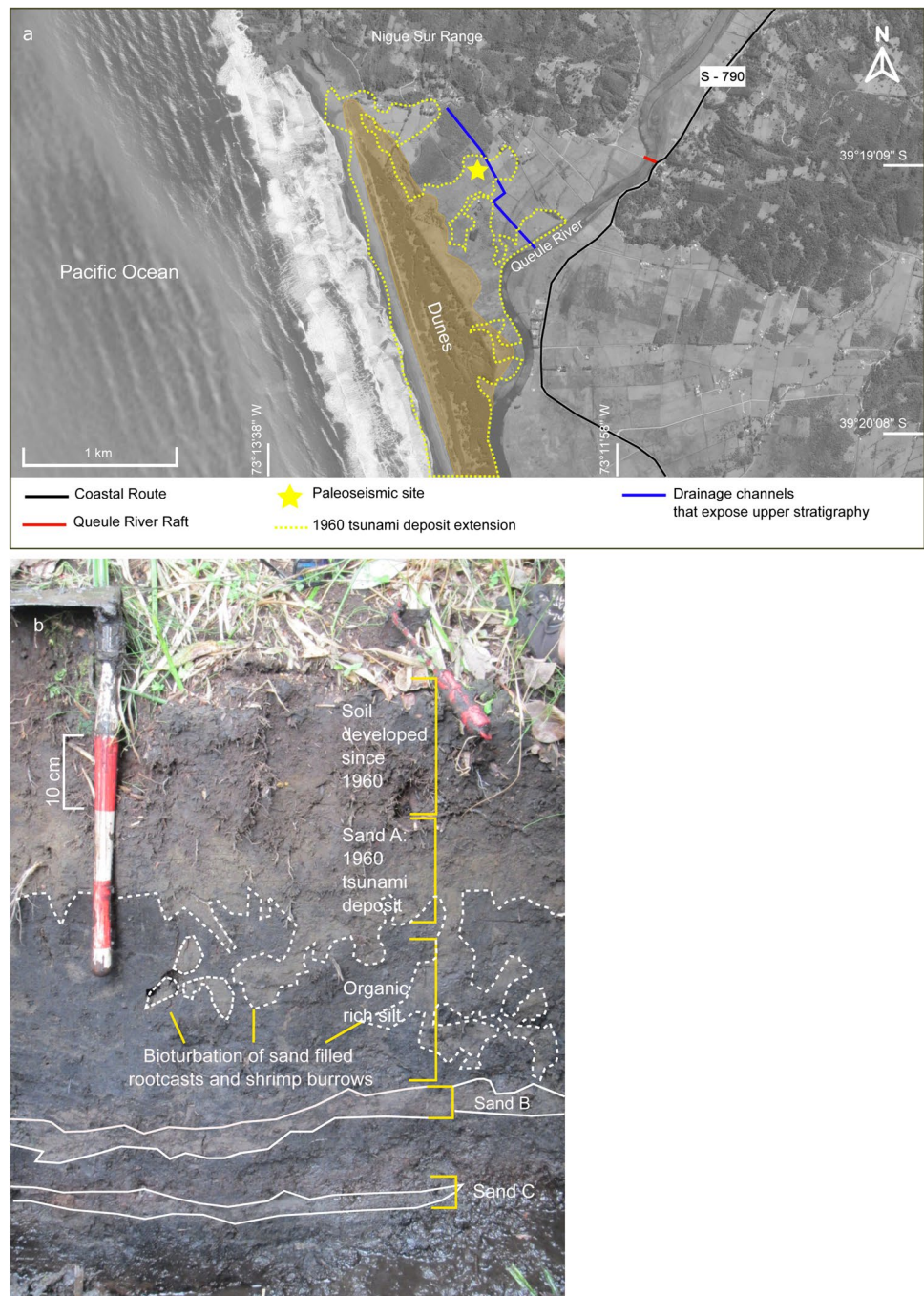
Fig. 6 Paleoseismic site of Queule. a) Aerial image of Queule paleoseismic site, Araucanía Region. b) Stratigraphic section of Queule site (Nigue Sur sector) with 3 sand deposits of tsunamis and peaty soils intercalated. Modified from Matos (2019)
