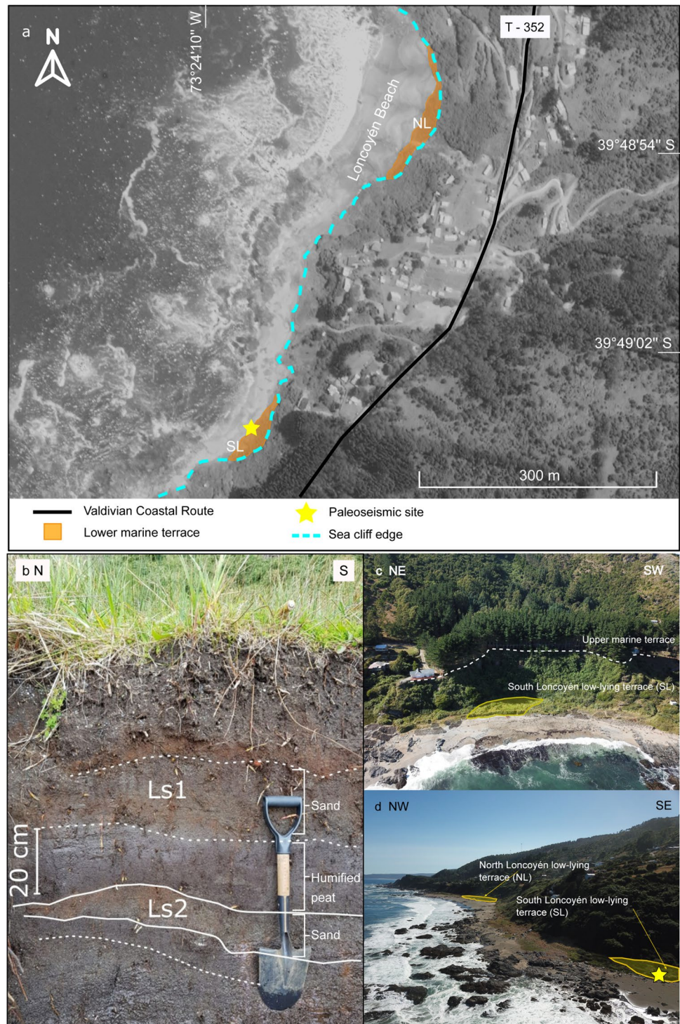
Fig. 7 Paleoseismic site of Loncoyén. a) Aerial image of Loncoyén paleoseismic site, Los Ríos Region. b) Profile of the lower terrace in South Loncoyén where dotted white lines indicate gradual contacts and solid white lines indicate sharp contacts. Ls1 and Ls2 corresponds to sand layers (modified from Ditzel (2019)). c) Marine terraces in South Loncoyén where dotted white line indicates the edge of the upper terrace of middle-upper Pleistocene age (Villalobos 2005) and the yellow shaded area indicates the surface of the lower Holocene terrace. d) Loncoyén beach that shows the lower terraces of North and South Loncoyén
