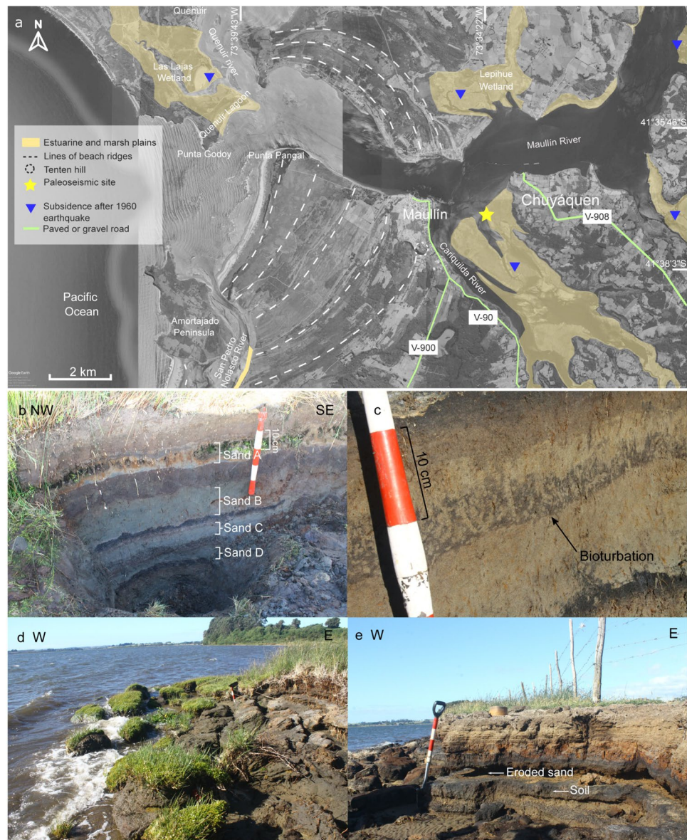
Fig. 9 Paleoseismic site of Mauullín. a) Aerial image of Mauullín paleoseismic site, Los Lagos Region. b) Stratigraphic units of the paleoseismic site of Mauullín showing sharp and erosive contact of the layers related to tsunami deposits described by Cisternas et al. (2005). c) Evidence of bioturbation in one of the buried soils overlaid by sand. d) Natural degradation of the marsh with truncated soils due to wind and waves in Mauullín River estuary. e) Natural degradation due to the waves in the estuary where it is possible to observe the erosion of the exposed layers left by tsunamis in Mauullín estuary
