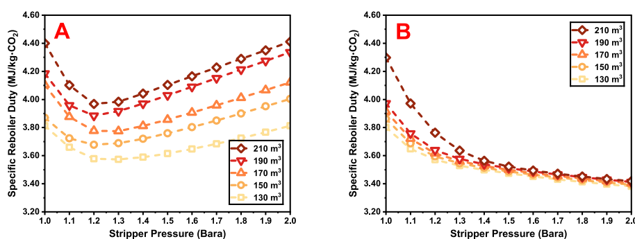
Fig. 11. Specific reboiler duty against stripper pressure for various gas flow rates with a CO 2 concentration of 20 mol%, achieving 90 % capture efficiency at their optimal L/G ratios for cross-heat exchanger duty of 43 kW (A) and minimised hot rich and hot lean solvent approach temperature (B).
