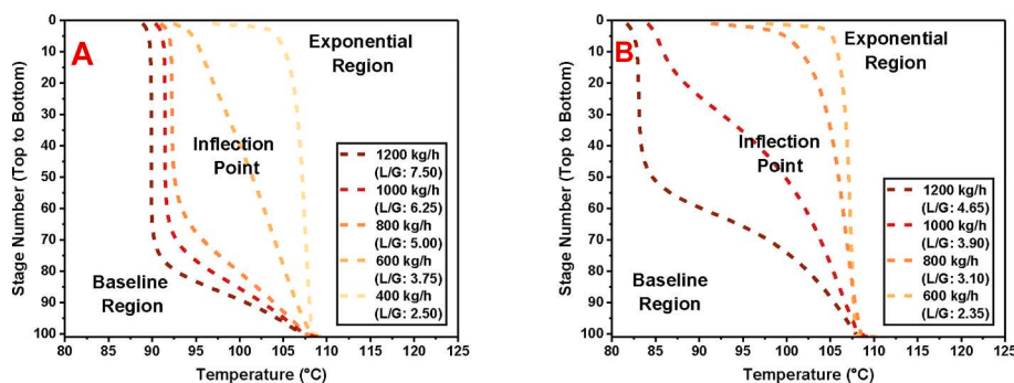
Fig. 8. Stripper temperature profiles with gas flow rates of 130 Nm 3 /h (A) and 210 Nm 3 /h (B) with a CO 2 concentration of 20 mol%, treated with 35 wt% MEA solvent flow rates to achieve 90 % capture efficiency.
