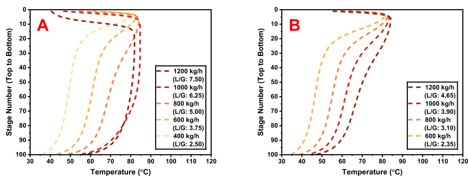
Fig. 7. Absorber temperature profiles with gas flow rates of 130 Nm 3 /h (A) and 210 Nm 3 /h (B) with a CO 2 concentration of 20 mol%, treated with 35 wt% MEA solvent flow rates to achieve 90 % capture efficiency.
