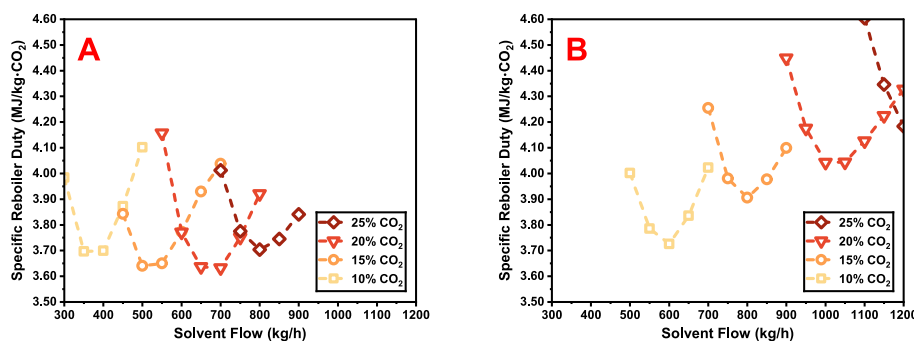
Fig. 6. Specific reboiler duty against solvent flow rate for gas flow rates of 130 Nm 3 /h (A) and 210 Nm 3 /h (B) for a range of CO 2 concentrations at 95 % capture efficiency.
