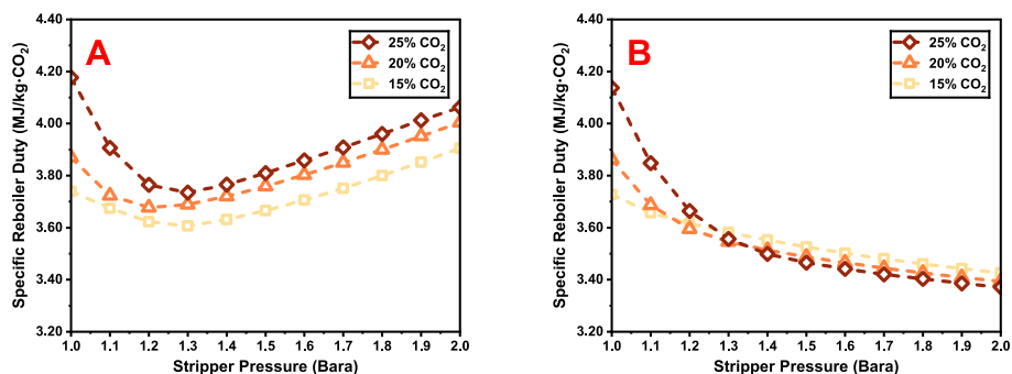
Fig. 13. Specific reboiler duty against stripper pressure for 150 \text{ Nm}^3/\text{h} gas flow rates with a range of \text{CO}_2 concentrations achieving 90 % capture efficiency with a cross-heat exchanger duty of 43 kW (A) and minimised hot rich and hot lean approach temperature (B).
