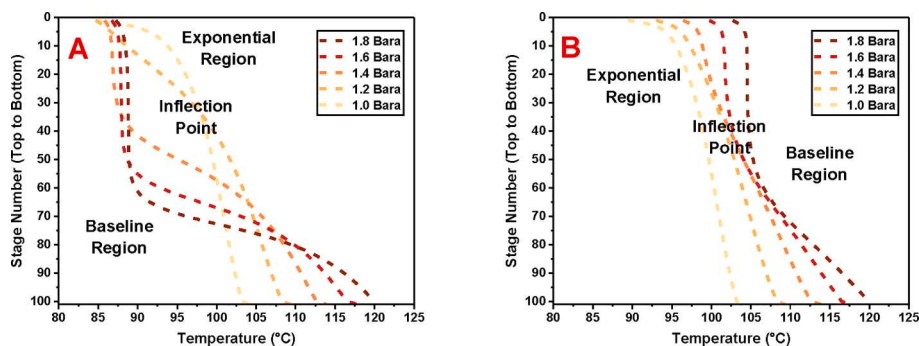
Fig. 12. Stripper temperature profiles with gas flow of 210 \text{ Nm}^3/\text{h} with a \text{CO}_2 concentration of 20 mol% for a range of stripper pressures achieving 90 % capture efficiency with a cross-heat exchanger duty of 43 kW (A) and minimised hot rich and hot lean solvent approach temperature (B).
