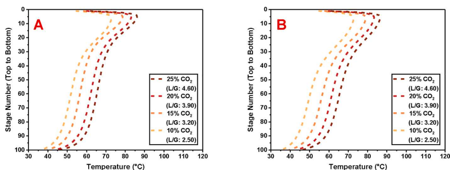
Fig. 9. Absorber temperature profiles with gas flow rates of 130 Nm 3 /h (A) and 210 Nm 3 /h (B) for a range of CO 2 concentrations at predicted optimal L/G ratios to achieve 90 % capture efficiency.
