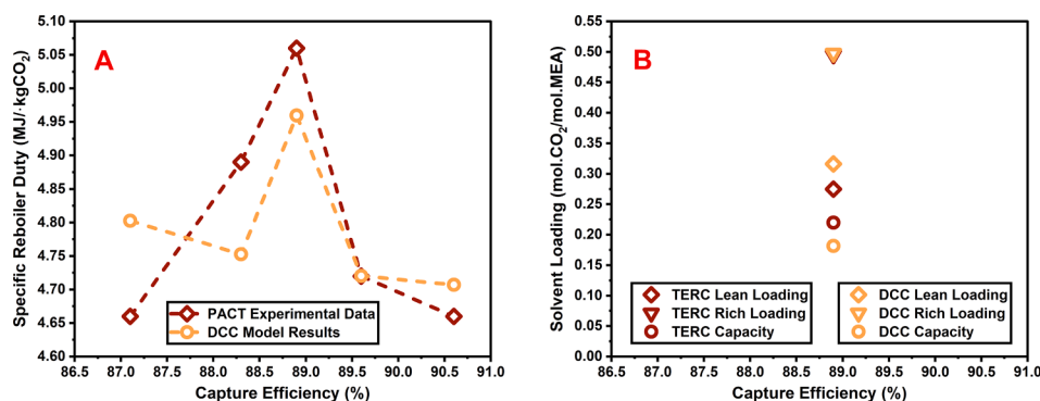
Fig. 4. Specific reboiler duty against capture efficiency for preliminary TERC ACP cases (A), with corresponding CO 2 loadings data for 88.9% capture efficiency (B).
