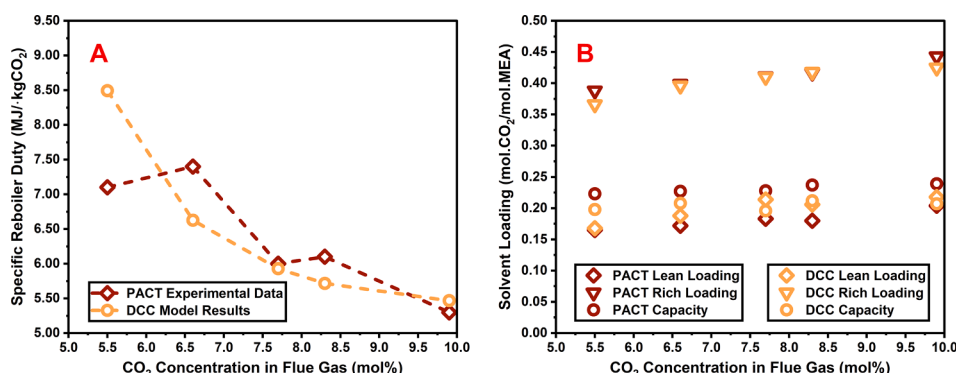
Fig. 2. Specific reboiler duty against flue gas CO 2 concentration for the PACT ACP (A), with corresponding CO 2 loadings data (B).
