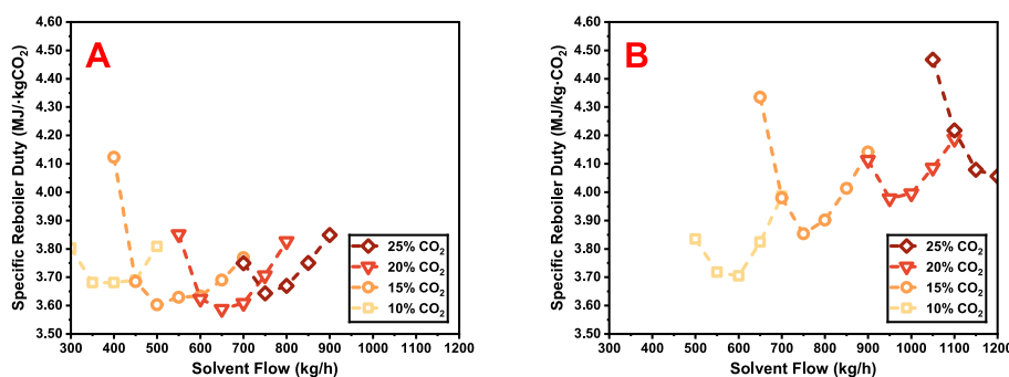
Fig. 5. Specific reboiler duty against solvent flow rate for gas flow rates of 130 Nm 3 /h (A) and 210 Nm 3 /h (B) for a range of CO 2 concentrations at 90 % capture efficiency.
