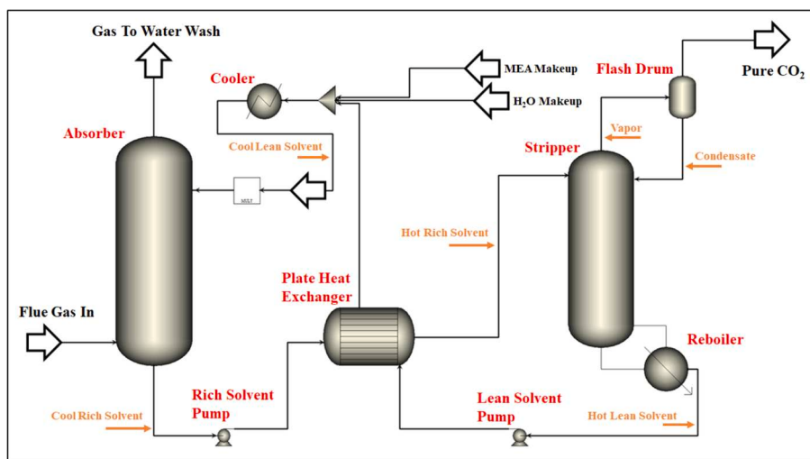
Fig. 1. Process flow diagram of the TERC ACP Aspen Plus V11.0.
