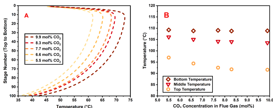
Fig. 3. Absorber temperature profiles with different flue gas CO 2 concentration cases for the PACT ACP (A), with corresponding stripper temperature monitoring (B).
