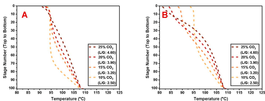
Fig. 10. Stripper temperature profiles with gas flow rates of 130 Nm 3 /h (A) and 210 Nm 3 /h (B) for a range of CO 2 concentrations, at predicted optimal L/G ratios to achieve 90 % capture efficiency.
