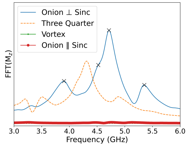
Fig. 2. Fourier transform of the M_z component for each of the ring states shown in Fig. 1 following the application of a sinc pulse in the x -direction. Black crosses mark position of main modes identified.
