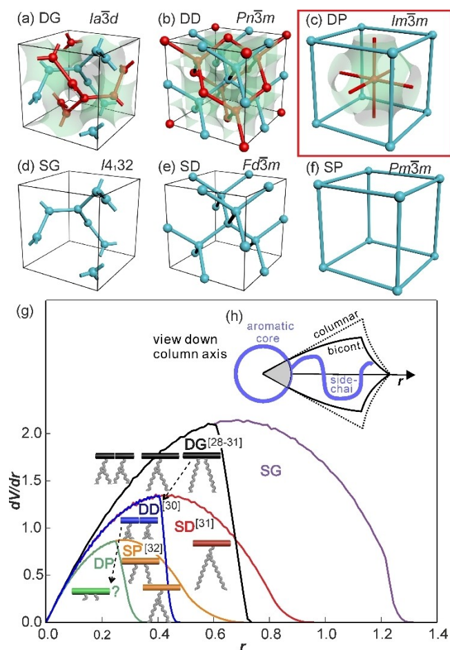
Figure 1. (a–c) Three double-network cubic phases with their infinite minimal surfaces (green) and (d–f) the corresponding single-network cubic phases, showing their abbreviations and space groups. (g) Radial distribution of volume functions dV/dr for the corresponding phases, where V(r) is the fraction of the volume in the unit cell that is closest to a given network segment and at a distance r from it. The color-coded stylized molecules are actual published examples of glycerol-capped rod-like compounds with side-chains displaying bundle-type cubic mesophases of the corresponding type (references in brackets). Side-chain size is to scale with real molecules. The missing compound of unknown shape in DP is marked with “?”. (h) A schematic view down a bundle (blue circle) with the time-averaged envelope of the side-chain(s) of one of its molecule.
