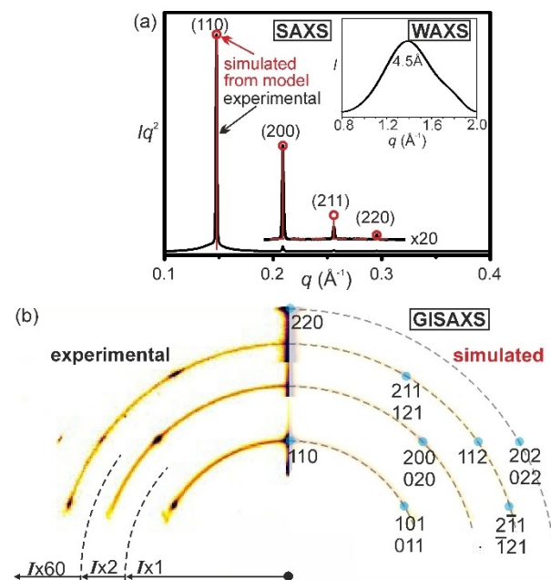
Figure 2. (a) Powder SAXS/WAXS pattern of FO-MeC16 recorded in the cubic phase at 50 °C; (b) experimental and simulated GISAXS pattern of FO-MeC16 recorded at 50 °C. The experimental GISAXS pattern is composed of three patterns on different intensity scales, as indicated. Simulated diffraction spots are shown on the right for (110) orientation of the body-centered cubic Im \bar{3}m .
