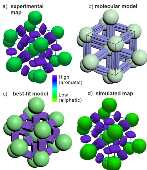
Figure 3. Electron density maps reconstructed from (a) experimental Bragg intensities and (d) best-fit model in (c). The model consists of (b) prisms and spheres representing bundles of rods and aggregated alkyl chains, respectively.
