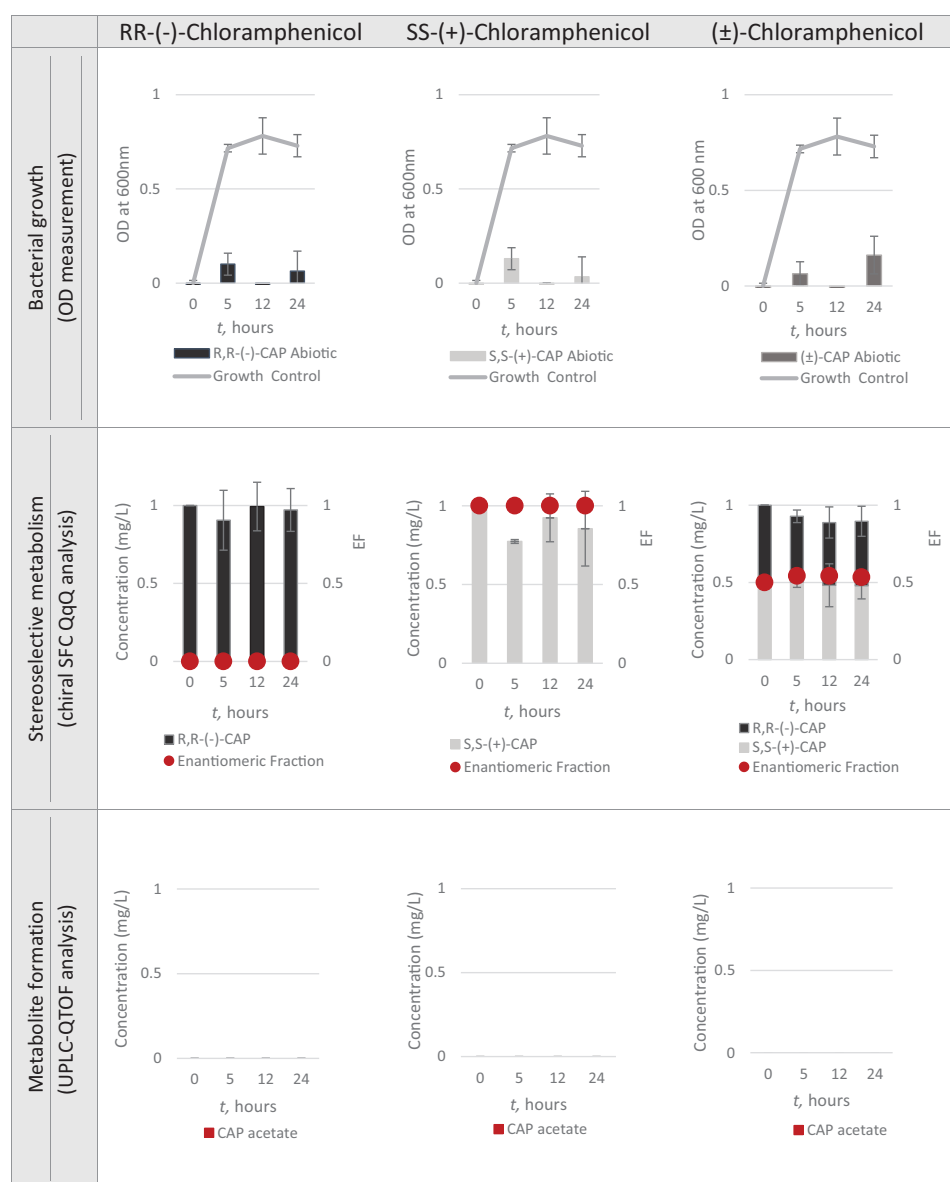
FIGURE 5 | Nanocosm assay – abiotic conditions ( n = 3 ).
