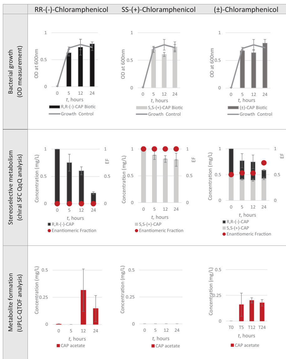
FIGURE 4 | Nanocosm assay - biotic conditions ( n = 3 ).
