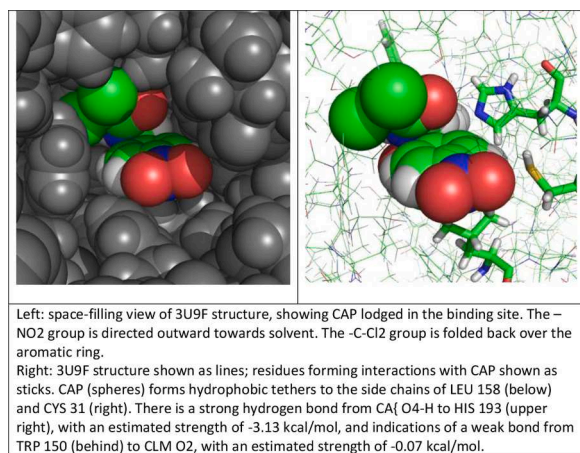
Fig. 8. CAP bound in a Type I CAT, 3U9F
