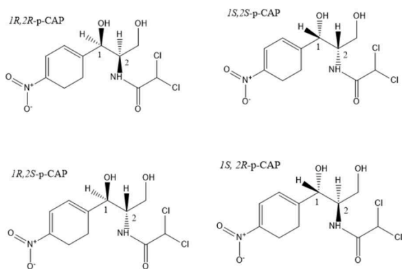
Fig. 1. Chloramphenicol isomers
