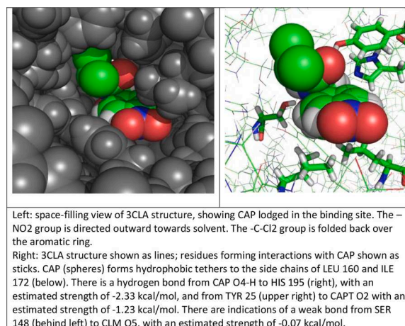
Fig. 9. CAP bound in a Type III CAT, 3CLA.
