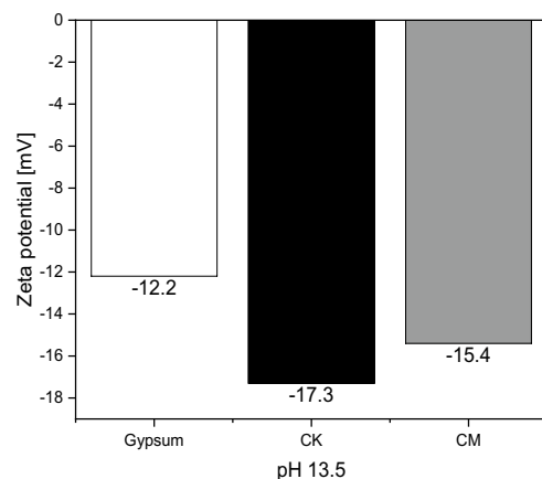
Fig. 8 Zeta potential of GYP, \text{CK}_{\text{finer}} and \text{CM}_{\text{finer}} in the artificial pore solution
