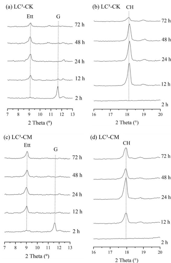
Fig. 11 XRD patterns of LC 3 -CK (a, b) and LC 3 -CM (c, d) hydrated pastes. Ett Ettringite, G Gypsum, CH Portlandite
