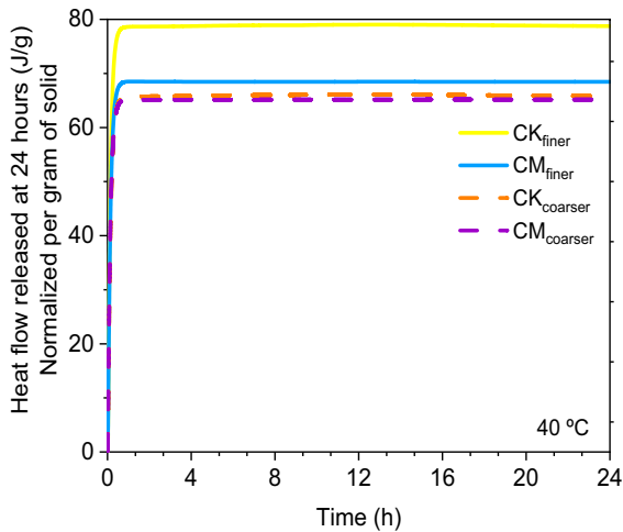
Fig. 2 Reactivity of calcined clays by R^3 test
