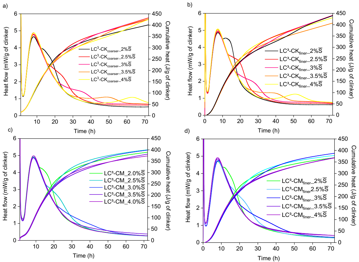
Fig. 4 Calorimetry results. a \text{LC}^3\text{-CK}_{\text{coarser}} b \text{LC}^3\text{-CK}_{\text{finer}} c \text{LC}^3\text{-CM}_{\text{coarser}} and d \text{LC}^3\text{-CM}_{\text{finer}} . Heat flow (left) and cumulative flow (right) of the \text{LC}^3 cement pastes
