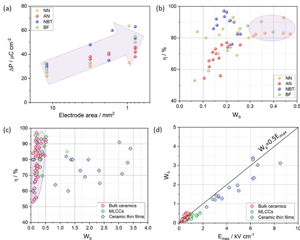
Fig. 20 The relationship between (a) electrode area and \Delta P in NN, AN, NBT, and BF-based ceramics (b) normalised W_{\text{b}} and \eta in NN, AN, NBT, and BF-based ceramics (c) normalised W_{\text{b}} and \eta in bulk ceramics, MLCCs, and thin films (d) normalised W_{\text{b}} and E_{\text{max}} in bulk ceramics, MLCCs, and thin films.
