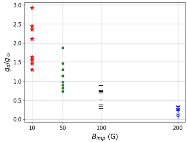
Figure 7. Plot showing the normalized deceleration vs. the imposed magnetic field for eight tallest spicules for each B_{imp} .
