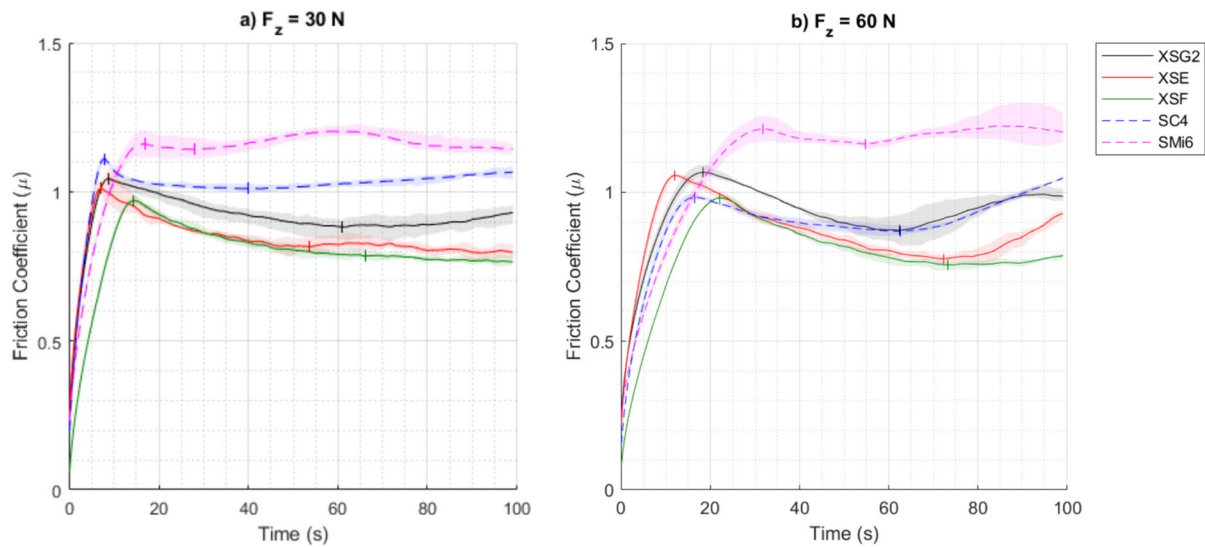
Fig. 6 Friction coefficient ( \mu ) against time for all compared brands under a normal load of a 30 N and b 60 N; highlighting the points where static and dynamic friction coefficients ( \mu_s , \mu_d ) are noted with vertical dashes, and one standard deviation ( N=5 ) denoted by shaded overlays
