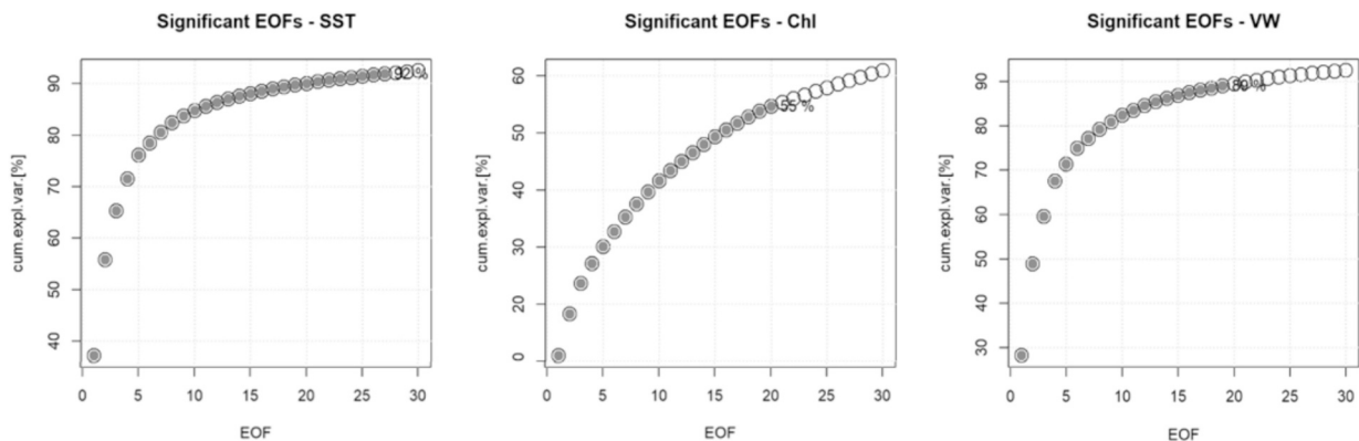
Fig. 3. The cumulative sum of the variance in the percentage of SST, Chl and VW. The grey points showed the temporal EOF selected in the construction. Note that The Y-axis, showing the cumulative explained variance, has a different scale for each graph.
