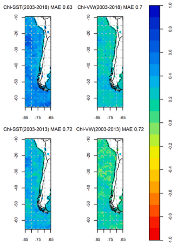
Fig. 4. Correlation R of the Chl vs the Chl predicted fields using SST and VW. The first row shows the CCA prediction using Full Chl data (2003–2018). The bottom row shows the Chl predicted over 2003–2018 years using the Training Mode (2003–2013) correlated with the Chl data (2003–2018).
