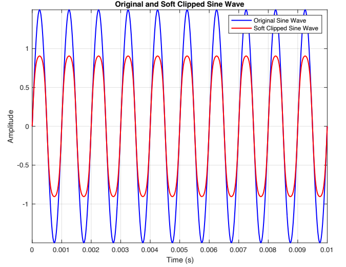
Fig. 2. Visual representation of soft clipping.
