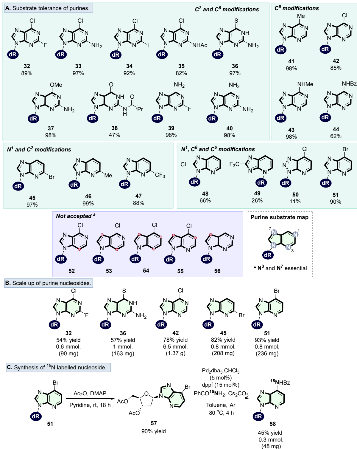
Figure 5. (A) Substrate scope of transglycosylation using purine nucleobases. General reaction conditions: 8 (dC) or Thymidine (5-10 equiv.), nucleobase (1 equiv.), solvent (organic:H 2 O,1:4), LINDT-2 (0.2% v/v to
