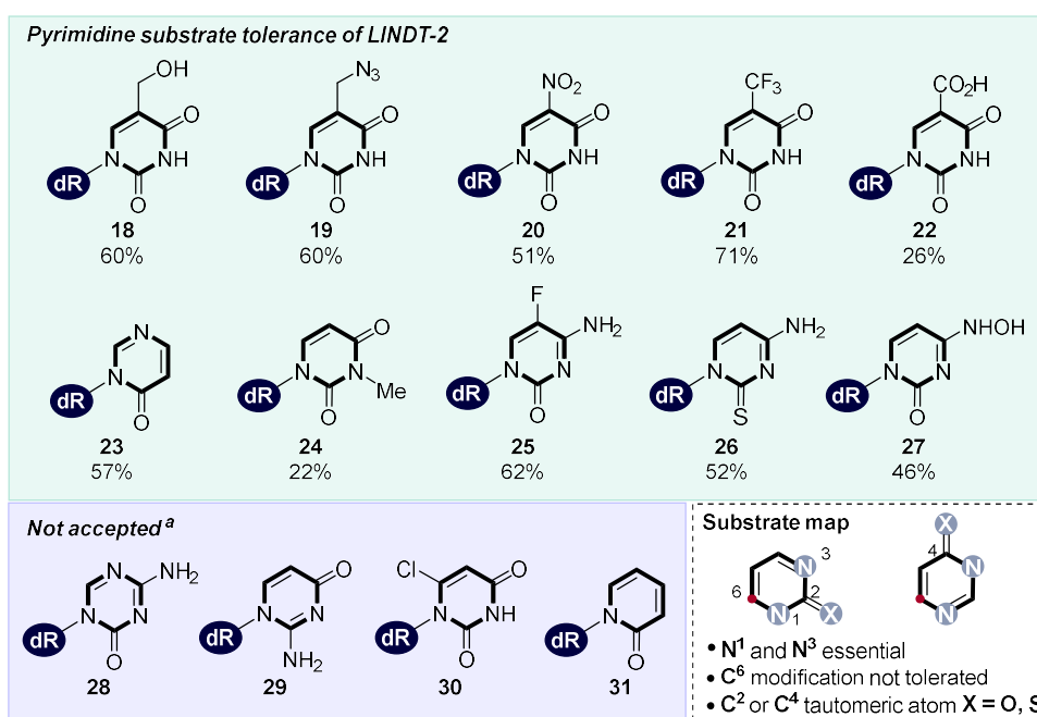
Figure 4. Substrate scope of transglycosylation using pyrimidine nucleobases. General reaction conditions: 8 (dC) or Thymidine (5-10 equiv.), nucleobase (1 equiv.), solvent (organic:H 2 O, 1:4), L INDT-2 (2 to 4 μg·mL -1 ), 40 °C, 24h. a Not accepted correlates to < 10% conversion.
