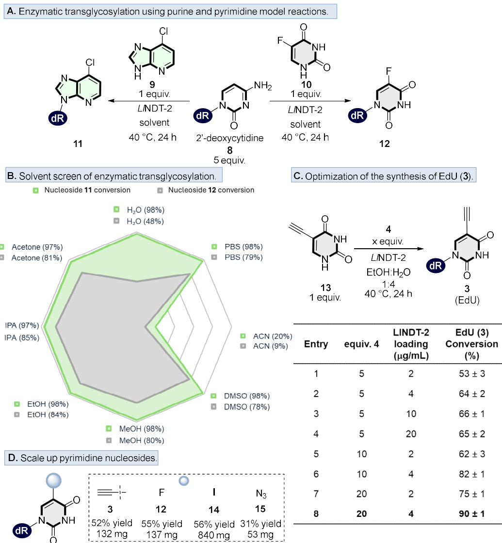
Figure 2. (A) Overview of the model reactions used to screen solvent dependency of transglycosylation catalysed by LINDT-2 . (B) % Conversion to nucleoside products 11 and 12 as a function of solvent. The % conversion was calculated by the ratio of the peak area of nucleobase to the peak area of the nucleoside product. (C) Optimization of the conversion of 3 (EdU) by surveying the number of equivalents of 2'-deoxyribosyl donor and LINDT-2 . General reaction conditions: 4 (5-20 equiv.), nucleobase (1 equiv.), solvent (EtOH:H 2 O,1:4), LINDT-2 (2 to 20 µg.mL -1 ). (D) Scale up of pyrimidine nucleoside analogues.
