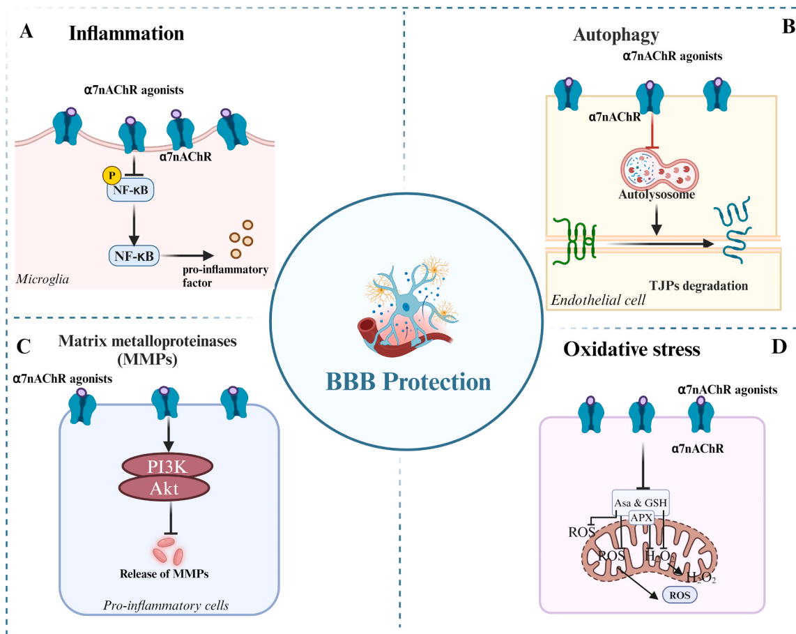
Fig. 2. Mechanisms of activation of \alpha 7 nAChR for BBB protection after stroke. (A) Activation of \alpha 7 nAChR inhibits NF- \kappa B nuclear translocation and release of inflammatory factors, and blocks microglia-induced inflammation. (B) \alpha 7 nAChR agonists protect BBB integrity by affecting autophagy-mediated degradation of tight junction proteins (TJPs). (C) Activation of \alpha 7 nAChR promotes phosphorylation of PI3K and Akt and inhibits the release of MMPs. (D) \alpha 7 nAChR agonists inhibit oxidative stress by reducing oxygen radical production through inhibition of NADPH oxidase.
