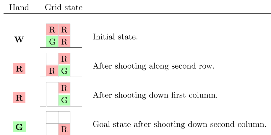
Fig. 15 Small instance admitting solutions of 1, 2 and 3 steps for a goal of single block remaining. 3-step solution presented
