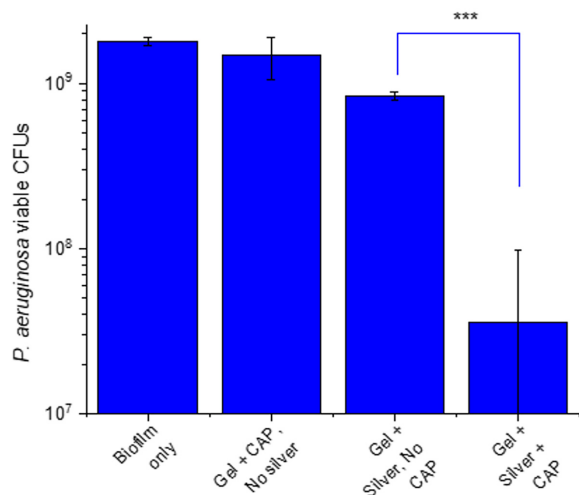
FIG. 4. Viable cell count of 8 h P. aeruginosa biofilms after 18 h of incubation with control composite hydrogels with no silver ( H_2O gel), with (CAP + H_2O Gel) silver loaded gels without CAP and silver loaded gels with CAP (CAP + Ag + Gel), and without (Ag + Gel) CAP activation relative to untreated control biofilms. Error bars represent the standard deviation of the mean and a 2-sample unpaired t test: *** p < 0.001 .
