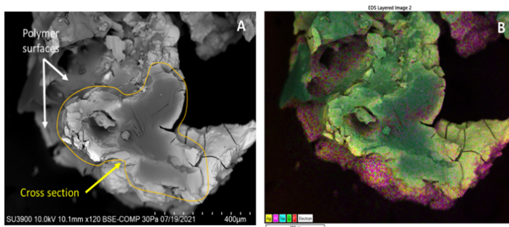
FIG. 2. Cross section of silver nitrate loaded PAA particle: (a) SEM and (b) EDX analysis [Ag (yellow), aluminum (pink), sodium (blue), oxygen (green), and carbon (red)]. Aluminum is used to externally cross-link the outside of the PAA particles.
