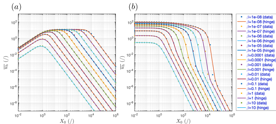
Fig. B.12. Comparison of (a) \bar{u}_h against \hat{u}_h , and (b) \bar{u}_v against \hat{u}_v for the set of \beta values adopted in Fig. 3. The fit of the hinge models to the numerical solution is generally strong but some discrepancies may be observed for values of \beta less than 10^{-3} , and at radial distances X_0 where the displacement components start decreasing monotonically.
