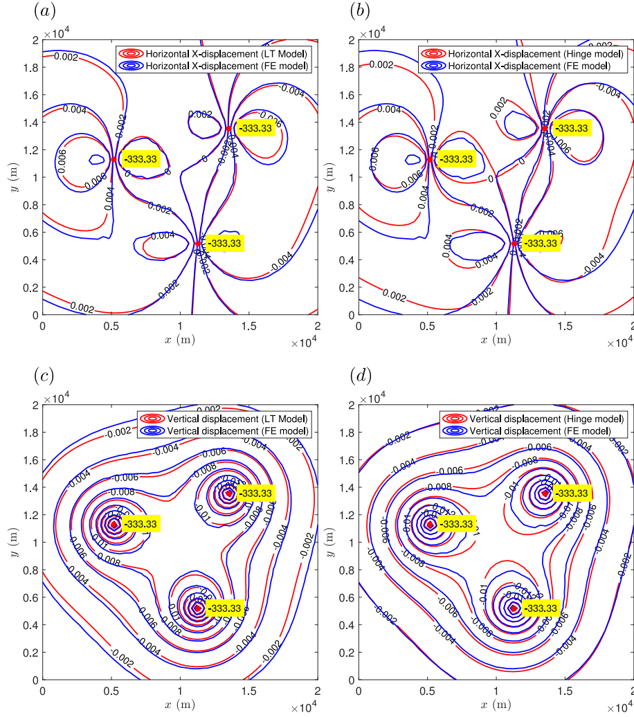
Fig. 8. Maps of the surface displacement u_x and u_z after 5 years of continuous operation of 3 wells extracting 333.33 \text{ m}^3/\text{d} continuously for 5 years. The three wells are equidistant from one another (8660.25 m) and at a distance of 5000 m from the well location in Well field #1, that is, (10,000 m, 10,000 m). Subpanels (a) and (b) present, for purposes of comparison, the u_x fields obtained with the FE model, the LT model and the hinge model, respectively. Subpanels (c) and (d) present the same comparisons for the u_z fields.
