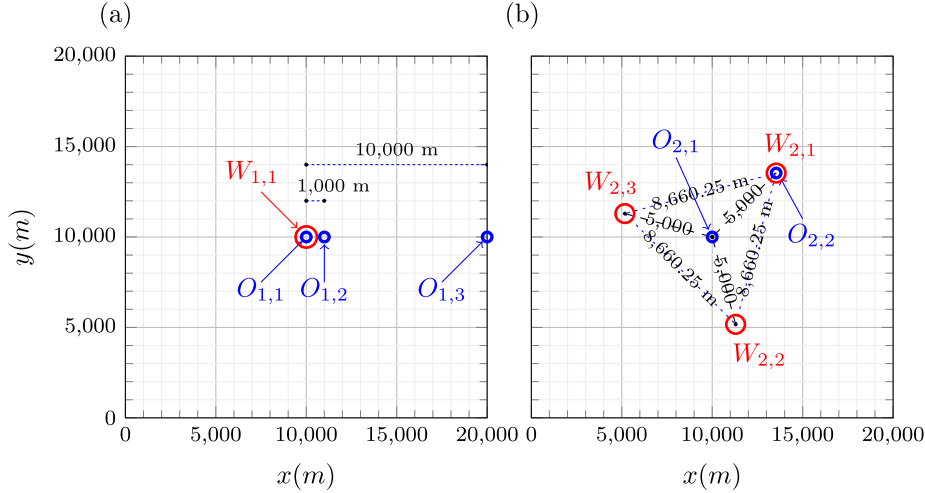
Fig. 5. Plan views of the well fields #1 (a) and #2 (b) adopted for model testing. Well field #1 includes a single well at W_{1,1} \equiv (10,000 \text{ m}, 10,000 \text{ m}) . Well field #2 consists of 3 wells, W_{2,1} , W_{2,2} , and W_{2,3} , at the vertices of an equilateral triangle with radius 5000 m and centred at the location W_{1,1} . Both subpanels show the location of observation points ( O_{1,1} , O_{1,2} , ...) chosen to plot profiles of the displacement vs. time.
