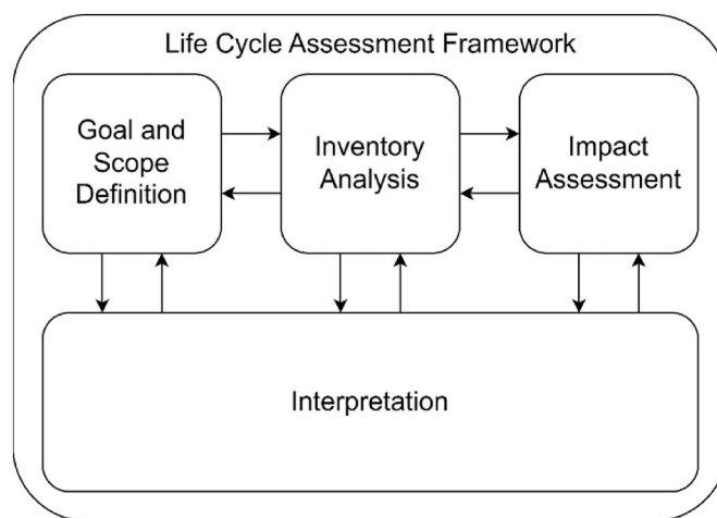
Fig. 1. LCA Framework, adapted from (INTERNATIONAL ORGANIZATION FOR STANDARDIZATION, 2006a).
