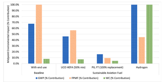
Fig. 4. Environmental impact assessment results (percentage contribution) for the SAF scenarios (GWP, ReCiPe Midpoint H – characterisation phase).
