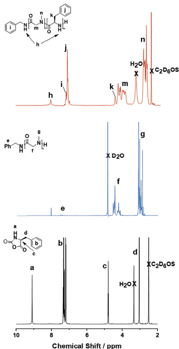
Figure 1. ^1\text{H} NMR spectra of Phe-NCA, the PSar macro-initiator, and PSar 113 -b-PPhe 16 , illustrating the loss of resonances attributable to Phe-NCA and indicating successful PPhe synthesis. Spectra obtained at 400 MHz using DMSO-d 6 and D 2 O.
