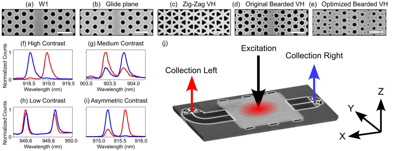
FIG. 3. SEM images of the fabricated waveguide for (a) W1, (b) glide plane, (c) zigzag VH, (d) original bearded VH, and (e) optimized bearded VH. Scale bars are 0.4 \mu\text{m} . Examples of dot lines split by B \neq 0 magnetic fields, with (f) high directional contrast, (g) medium contrast, (h) low contrast, and (i) asymmetric contrast. (j) Schematic of the on-chip device layout, indicating the location of the left out-coupler collection (red) and the right out-coupler collection (blue).
