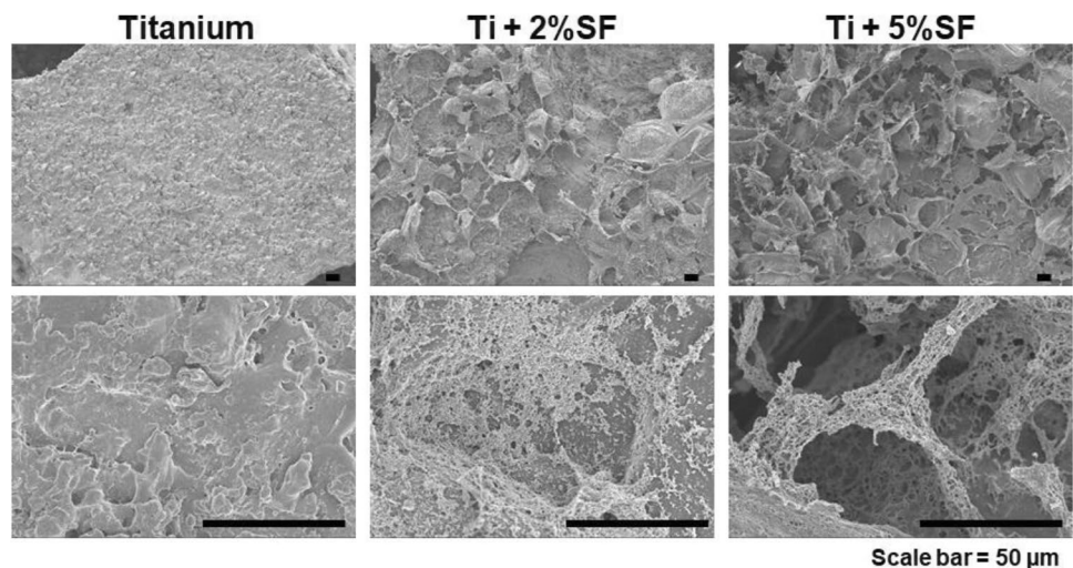
Fig. 12 SEM images showing thick deposition of SF coating with overlapping sheets, open porosity, formation of beads and anchoring fibrils which are the characteristics of SF. Scale bar = 50 μm
