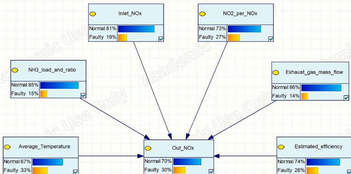
Fig. 7. BN structure for SCR system, built based on a method introduced in the literature [2].
