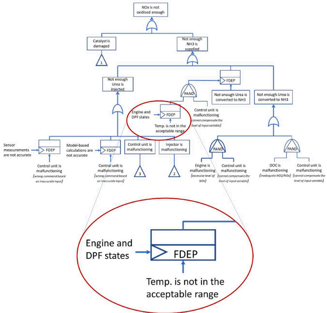
Fig. 8. The range of temperature is the true cause of the fault in the SCR system.
