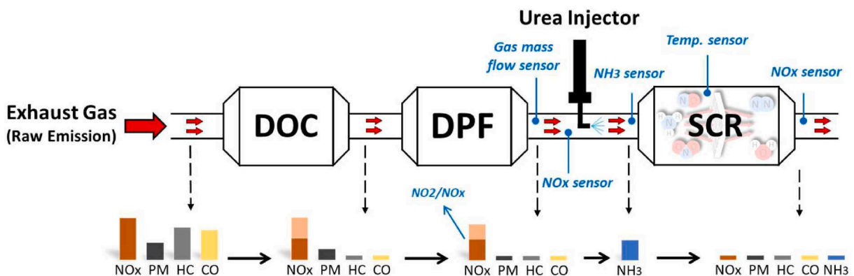
Fig. 2. A schematic illustration of the automotive Aftertreatment system, focused on SCR subsystem (Modified from [2]).
