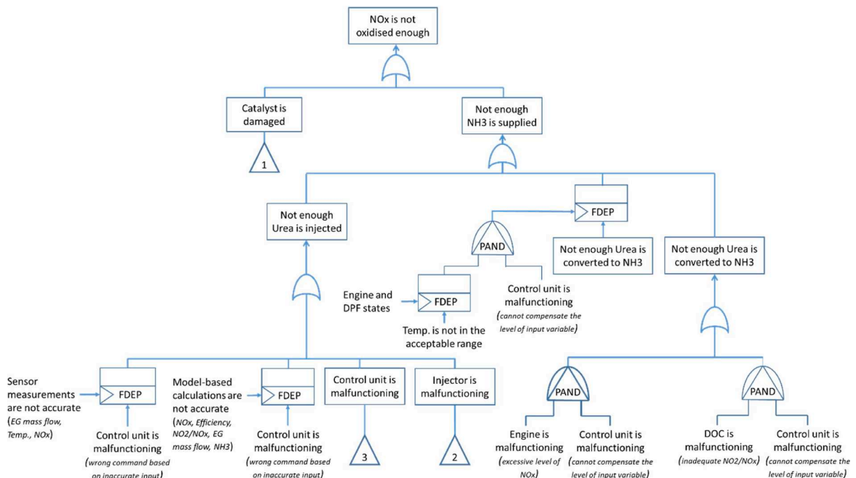
Fig. 6. Dynamic fault tree for SCR system.
