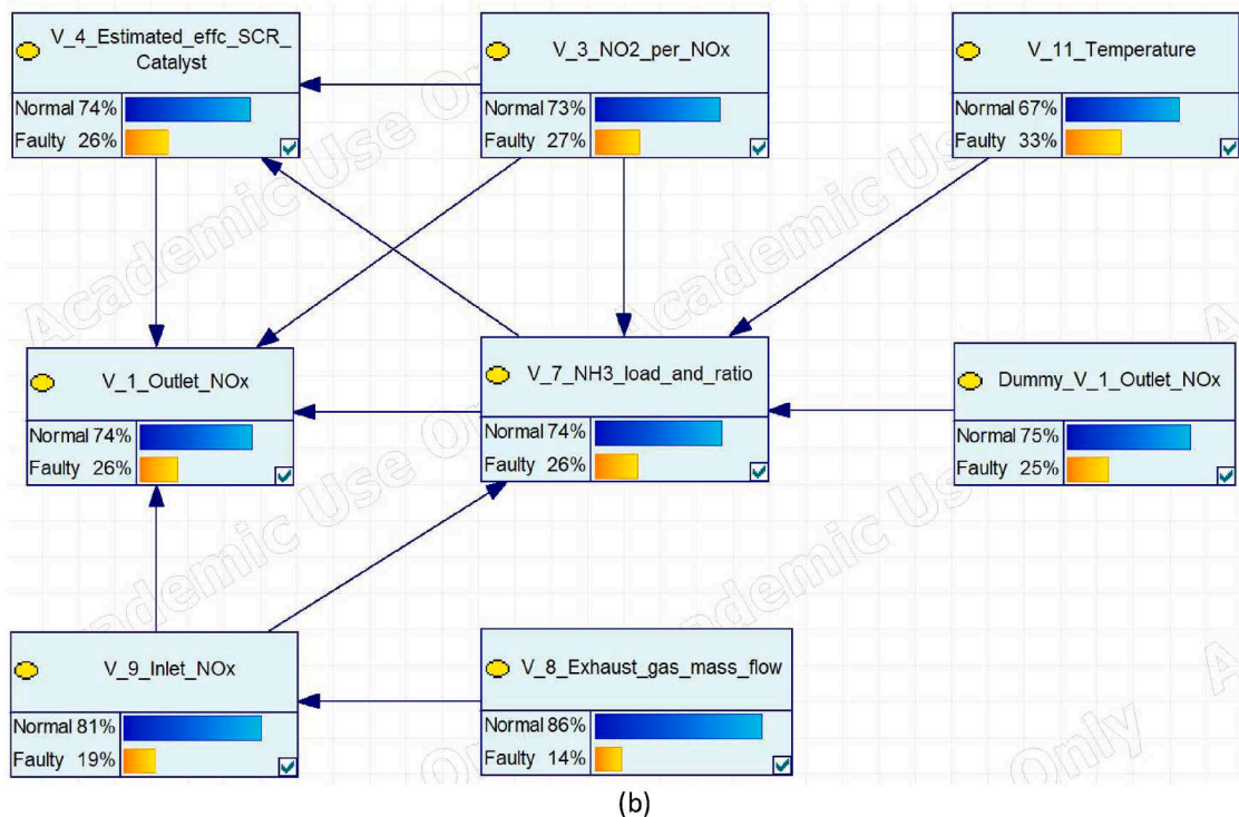
Fig. 5. (a) Simplified CLD for the SCR system, (b) The Bayesian network for SCR system based on engineering analysis.
