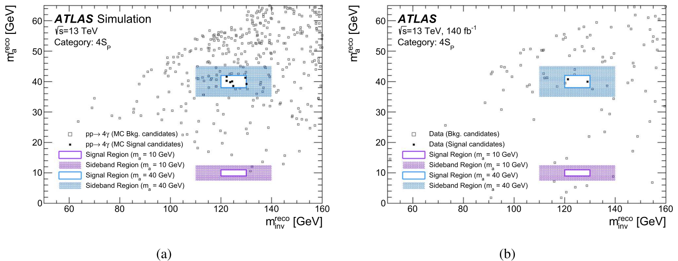
Fig. 4 m_{\text{inv}}^{\text{reco}} vs. m_a^{\text{reco}} for the 4S_P categories in the search for promptly decaying ALPs, for a simulated pp \rightarrow 4\gamma sample and b for data. The signal (sideband) regions are indicated by solid lines (shaded areas)
