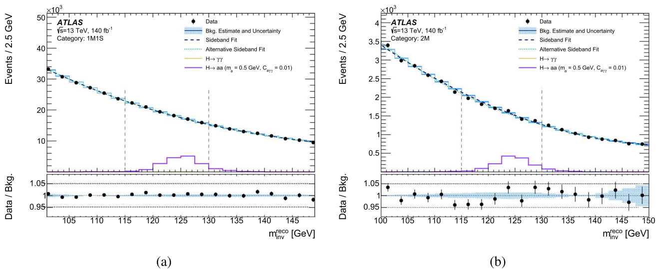
Fig. 2 m_{\text{inv}}^{\text{reco}} distribution for the nominal signal selection for the a 1M1S and b 2M category. The nominal sideband fitting function is shown as the blue dashed line. The background, estimated from a fit in the side-band regions, and its systematic uncertainty is shown as a blue histogram for both cases. The green dotted line shows the alternative fitting function used to estimate the spurious signal uncertainty (discussed in Sect. 6). The expected signal shape for m_a = 0.5 GeV, C_{a\gamma\gamma} = 0.01
