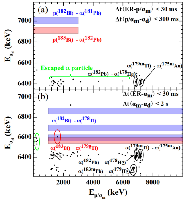
FIG. 2. (a) Two-dimensional E_{p/\alpha_m} - E_{\alpha_d} plot for \Delta t(\text{ER} - \alpha_m) < 30 ms and \Delta t(\alpha_m - \alpha_d) < 300 ms in the ^{78}\text{Kr} + ^{107}\text{Ag} reaction. (b) The same as (a) but with the time interval of \Delta t(\alpha_m - \alpha_d) < 2 s. The regions for the candidate p/\alpha_m (including the escaped events) - \alpha_d decay chains of ^{182,183}\text{Bi} are marked with transparent blue and red boxes, respectively. The events in the green ellipse in panel (b) could be associated with the CE of internal transition in the cascade depopulating the 11/2^- isomer of ^{179}\text{Tl} (see text for details). The event in red ellipses in panel can be interpreted as a proton decay of ^{185}\text{Bi} (see text for details).
