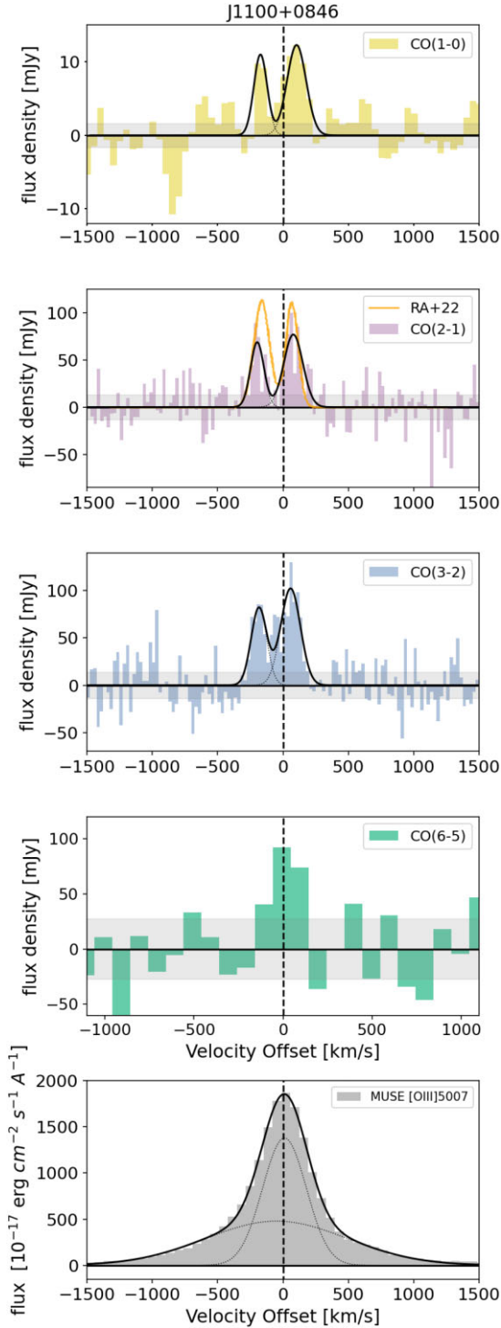
Figure 3. Example of multiple CO spectra and MUSE data obtained, here showing J1100+0846. Top panel: CO(1-0) from ACA. Second panel CO(2-1) from APEX (in this case, the data were from Jarvis et al. 2020). Third panel: CO(3-2) data from APEX. Fourth panel: CO(6-5) data from APEX. Fifth panel: MUSE spectra for the [O III] line extracted from a 30 arcsec diameter aperture. In all cases, solid black lines denote fits to the data. Here, more distant and there are multiple components and as such, the dotted black lines denote the different components that make the total fit to the spectra. In the CO(2-1) spectra, we also show the fit from higher resolution ALMA observations (solid orange line labelled RA+22, Ramos Almeida et al. 2022). Shaded grey regions represent the 1\sigma level. Spectra for all targets are shown in the appendix, using the same presentation methods.
