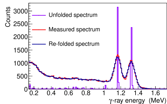
Fig. 7 Experimental, unfolded and refolded spectra for a response of a single detector to a ^{60}\text{Co} calibration source
