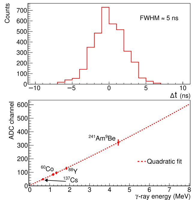
Fig. 2 Top: The time \Delta t between signals in different detectors corresponding to detected photo-peak \gamma -rays from a ^{60}\text{Co} source for a single NaI detector within the array. These \gamma -rays are emitted simultaneously, thus the measured distribution in time shows our intrinsic timing resolution. Bottom: Energy calibration for the same NaI detector. The quadratic fit is shown with a dashed line. The error bars on the data points represent full-width half-maxima of the \gamma -ray peaks
