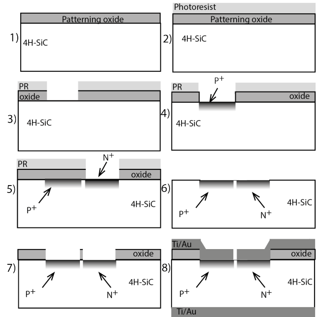
Fig. 5. Process steps
