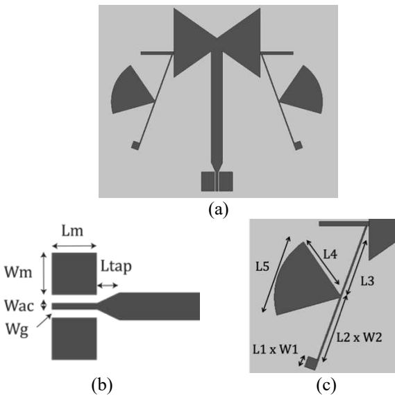
Fig. 4. (a) Antenna design. (b) zoom on the coplanar access. (c) zoom on the polarization circuit.
