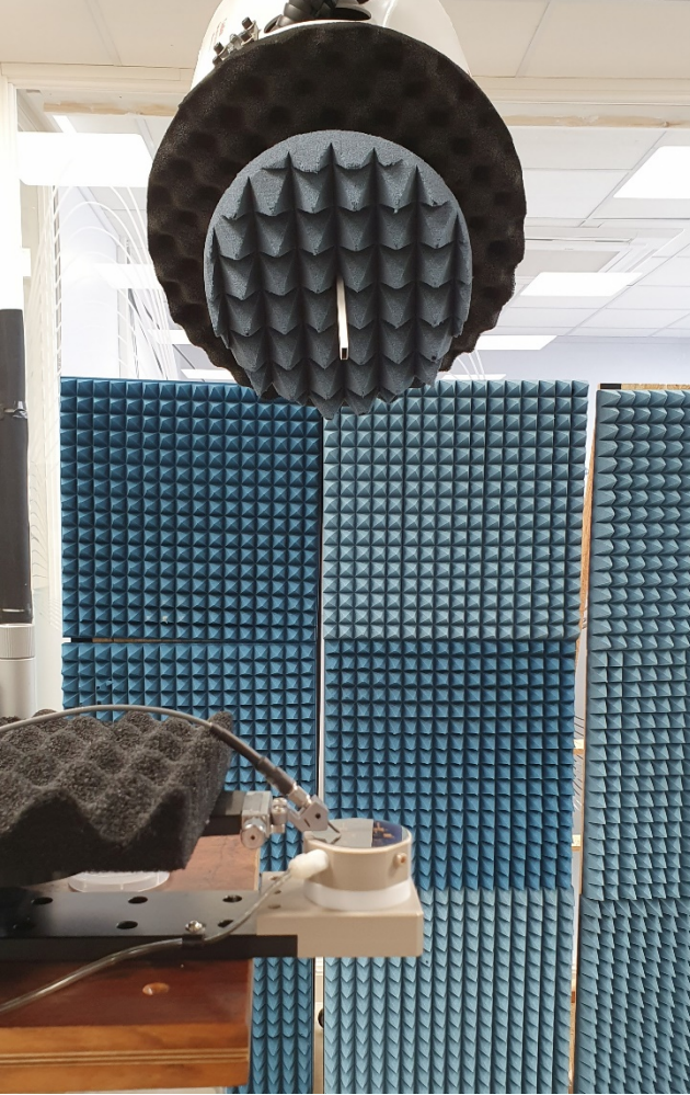
Fig. 7. Antenna undergoing radiated test on special mini probe station (phi sweep is vertically downwards as viewed here) [10].
