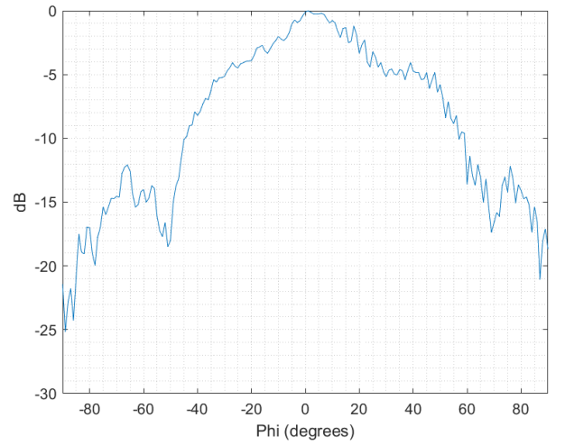
Fig. 9. Normalized Measured Radiation Pattern at location of peak power (diodes unbiased).
