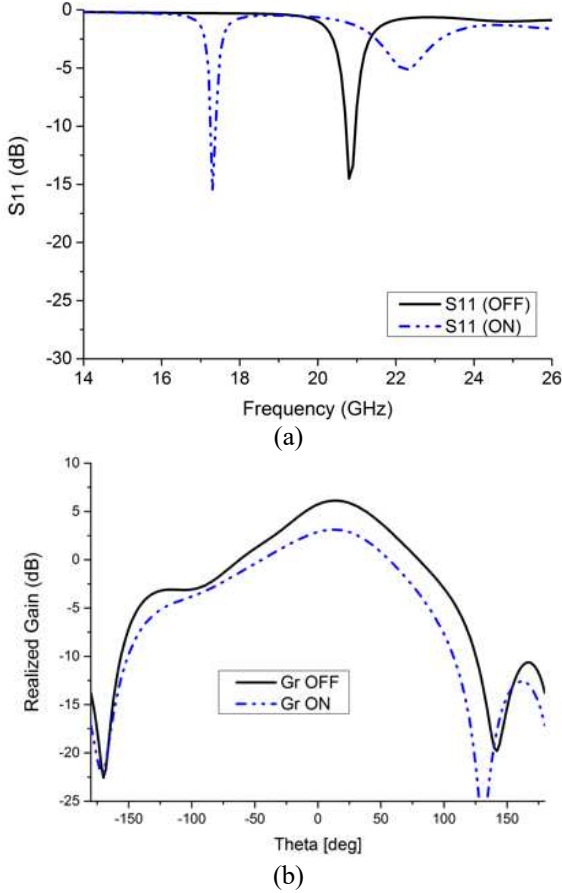
Fig. 3. Simulated results of the antenna. (a) S_{11} . (b) Realized Gain.
