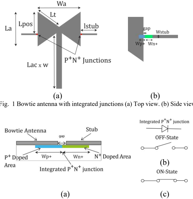
Fig. 2. (a) Side view of the antenna, zoom on the integrated junction. (b) OFF-state simplified model of the junction. (c) ON-state simplified model of the junction.
