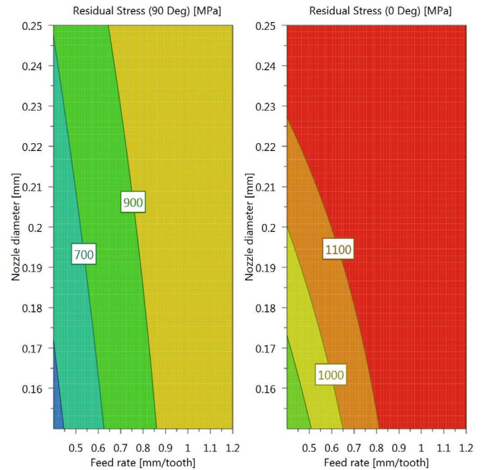
Fig. 6. A response contour plot of mean residual stresses (relationship between feed per tooth and nozzle diameter).
