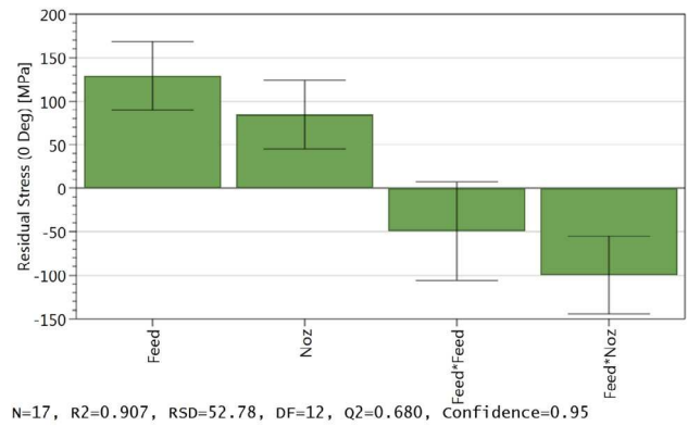
Fig. 3. Regression coefficient plot: influence of feed per tooth, nozzle diameter, and interactions on transverse residual stress ( \phi = 0^\circ ).
