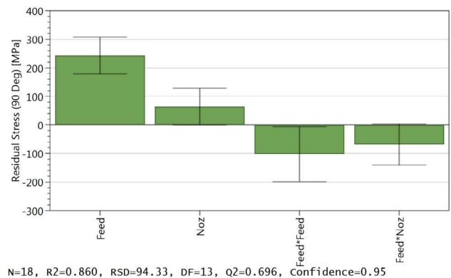
Fig. 4. Regression coefficient plot: influence of feed per tooth, nozzle diameter, and interactions on longitudinal residual stress ( \phi = 90^\circ ).
