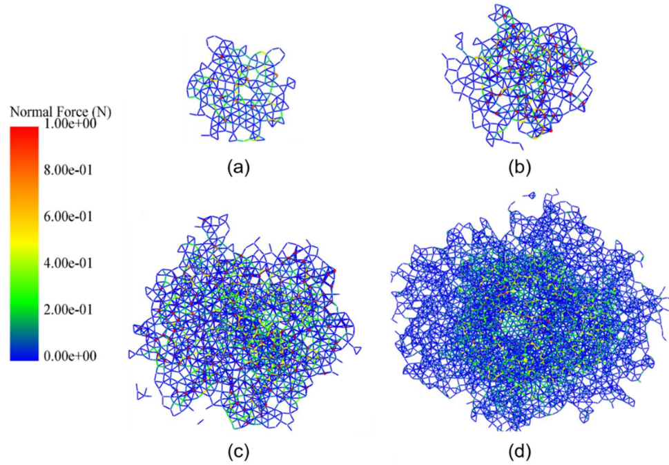
Fig. 13. The contact force network formed during crushing of a particle with a diameter of: (a) 0.83mm, (b) 1.0mm, (c) 1.5mm, and (d) 2.0mm obtained from the DEM models
