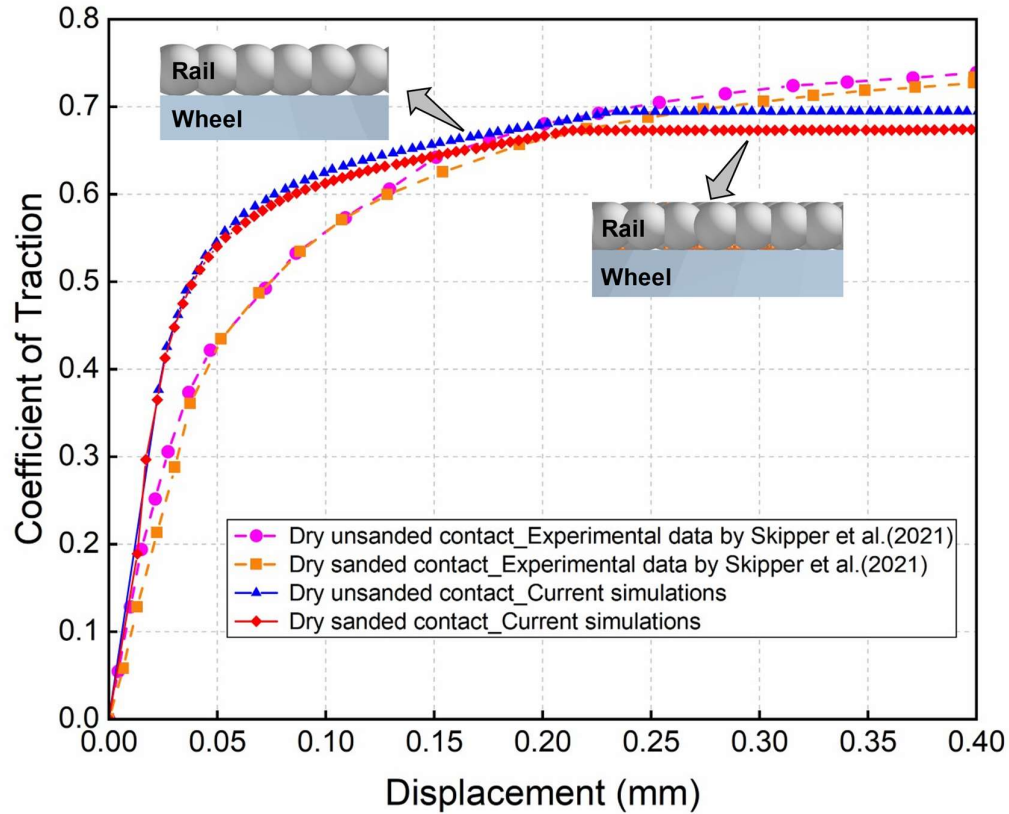
Fig. 5. Comparison of the coefficient of traction obtained from DEM modelling of the HPT set-up with and without the presence of sand particles under dry contact condition with the corresponding experimental data. (The light grey particles represent the rail specimen, and the orange particles represent the fragments of sand particles)
