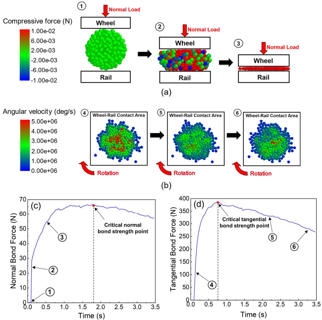
590 Fig. 9. The breaking behaviour of the sand particle and the evolution of the bond force in the 591 normal and tangential directions for particle with a 1.0 mm diameter, and a bond strength and 592 stiffness of 1.0 \times 10^8 [Pa] and 1.0 \times 10^{11} [N/m 3 ], respectively during the DEM modelling: (a) Changes 593 in the compression force of fragments during compaction (side view), (b) Changes in the 594 angular velocity of the fragments during torsion (top view), (c) Normal bond force, and (d) 595 Tangential bond force
