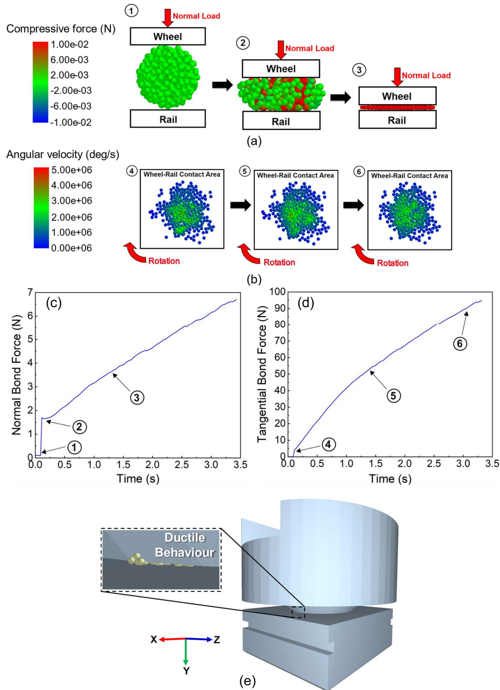
Fig. 7. The breaking behaviour of the sand particle and the evolution of the bond force in the normal and tangential directions for particle with a 1.0 mm diameter, and a bond strength and stiffness of 1.0 \times 10^{10} [Pa] and 1.0 \times 10^{10} [N/m 3 ], respectively, during the DEM modelling: (a) Changes in the compression force of fragments during compaction (side view), (b) Changes in the angular velocity of the fragments during torsion (top view), (c) Normal bond force, (d) Tangential bond force, and (e) the particle showing ductile behaviour when breaking
