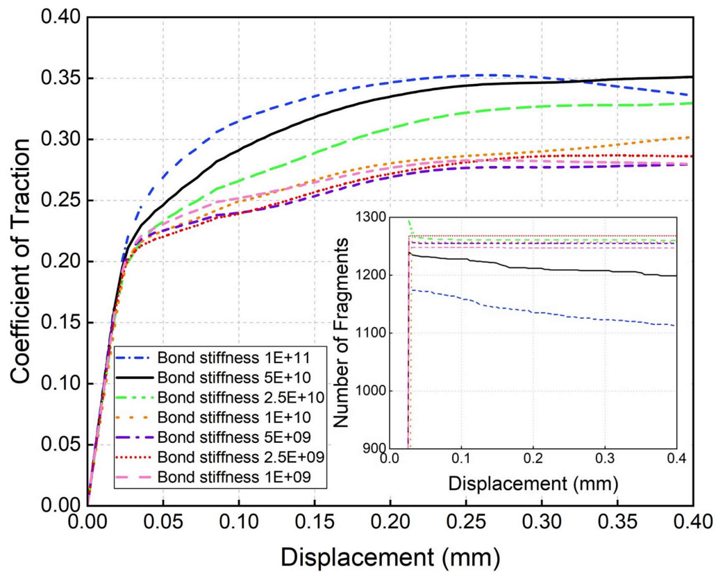
Fig. 8. Comparison of the coefficient of traction obtained from DEM modelling of the HPT set-up using different values of bond stiffness (The insert graph shows the number of fragments remaining on the contact area for each value of the bond stiffness)
