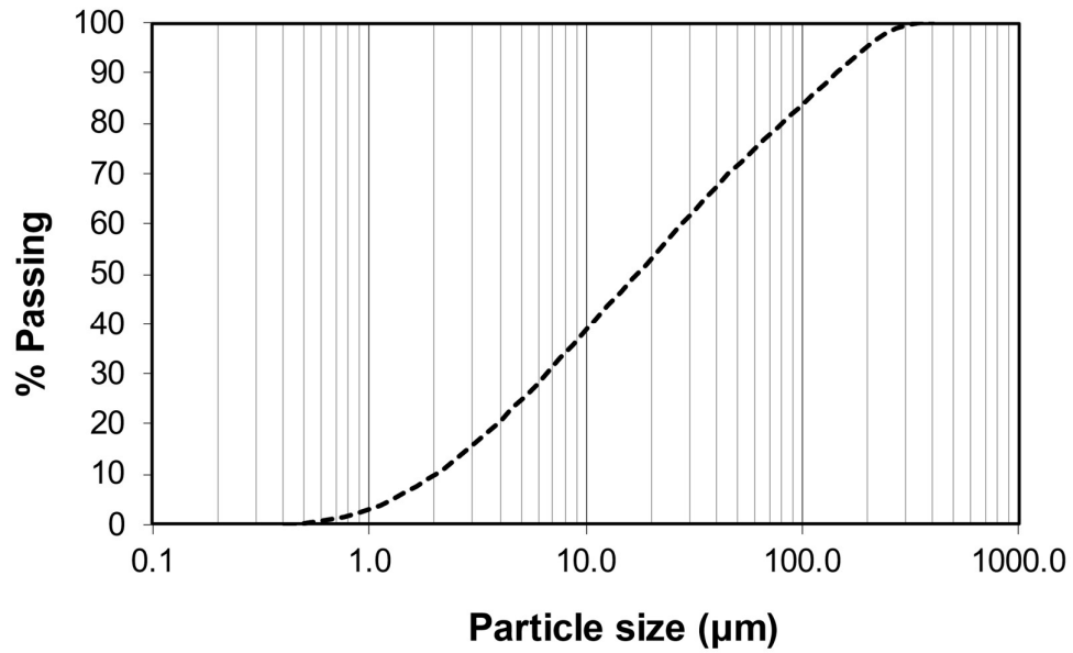
Fig. 3. Particle size distribution of the crushed sand obtained using laser diffraction (“% Passing” on the y-axis represents the percentage of particles in the sample that have a size smaller than or equal to a particular particle size on the x-axis)
