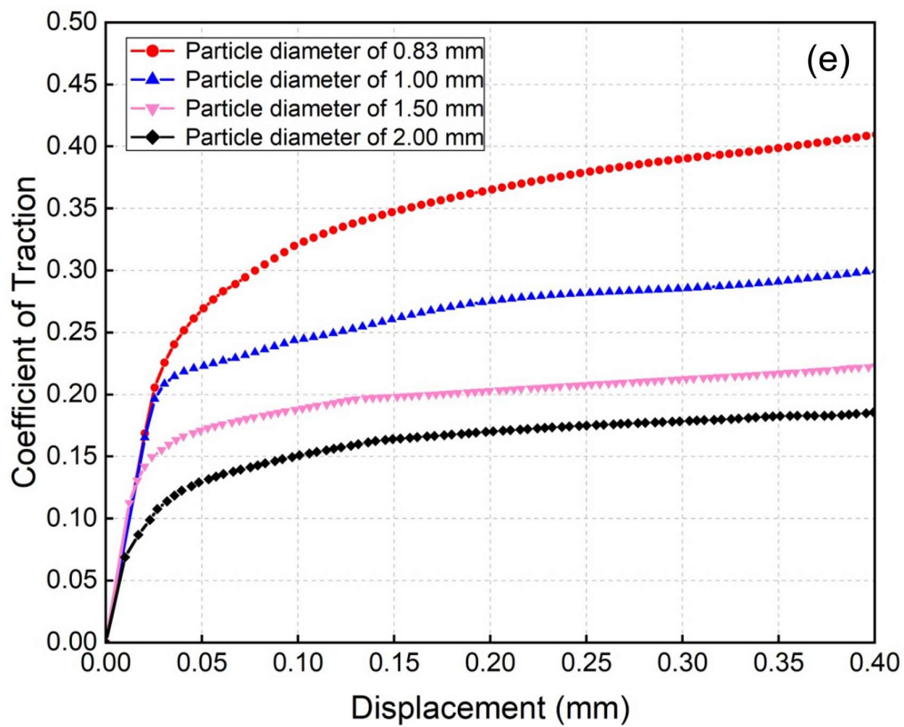
600 Fig. 10. Sand particles of different size with a diameter of: (a) 0.83mm, (b) 1.0mm, (c) 1.5mm, 601 and (d) 2.0mm used in the DEM models and (e) comparison of the coefficient of traction 602 obtained from DEM modelling of the HPT set-up using different particle sizes 603
