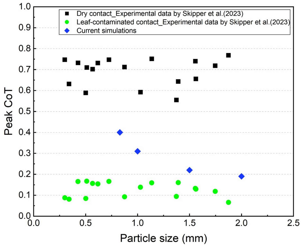
613 Fig. 12. Comparison of the peak coefficient of traction obtained from DEM modelling of the HPT 614 set-up (blue diamond) using different particle sizes to the experimental results for dry (black 615 square) and leaf-contaminated (green circle) contact condition by Skipper et al. (2023)
