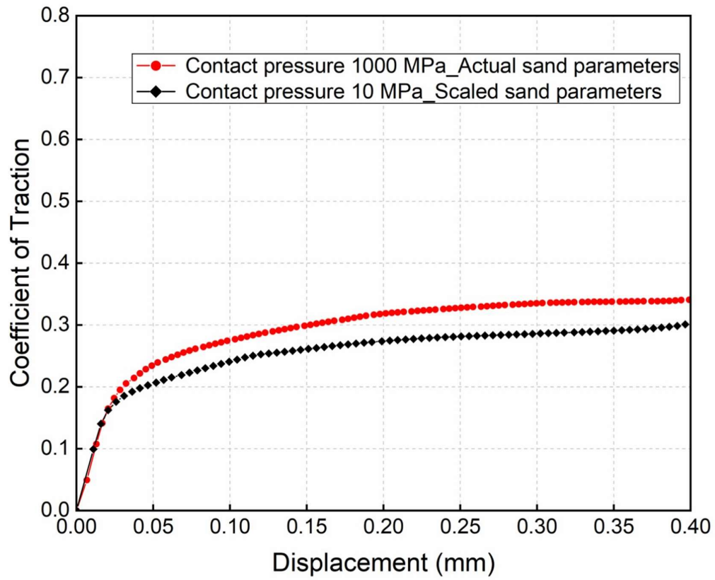
Fig. 1. Comparison of the coefficient of traction obtained from DEM modelling of the HPT set-up for the two cases using actual (red) and scaled (black) sand parameters
