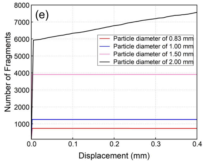
Fig. 11. Particle breakage in the contact area, the variation in the number of fragments depending on the particle size, and the possibility of the formation of fragment clusters and weak shear bands during the DEM simulation for particles with a diameter of: (a) 0.83mm, (b) 1.0mm, (c) 1.5mm, and (d) 2.0mm, and (e) comparison of the number of fragments produced during the DEM modelling of the HPT set-up for the above four particle sizes
