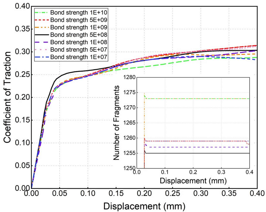
Fig. 6. Comparison of the coefficient of traction obtained from DEM modelling of the HPT set-up using different values of bond strength (The insert graph shows the number of fragments remaining on the contact area for each value of the bond strength)
