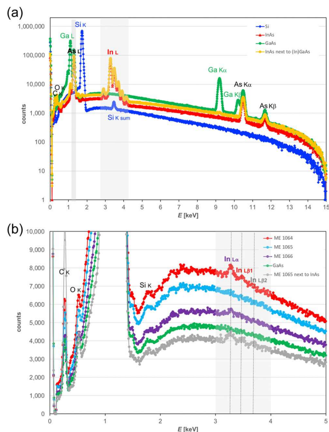
FIGURE 5 X-ray spectra at 15 kV from the surfaces of Si, InAs and GaAs wafers as well as the same InAs wafer adjacent to a piece of (In)GaAs wafer (a) and from GaAs wafers with different InGaAs layers on top (nominally 10, 5 and 2 nm of In 0.2 Ga 0.8 As for ME1064, 1065 and 1066, respectively) as well as InGaAs next to a piece of InAs wafer (b). The orange and grey spectra show that Ga K stray signals are very low while In L stray signals could be high and contribute an unwanted background. The Si K signal comes from the silicon drift detector itself. Source: Adapted from Walther [9].
