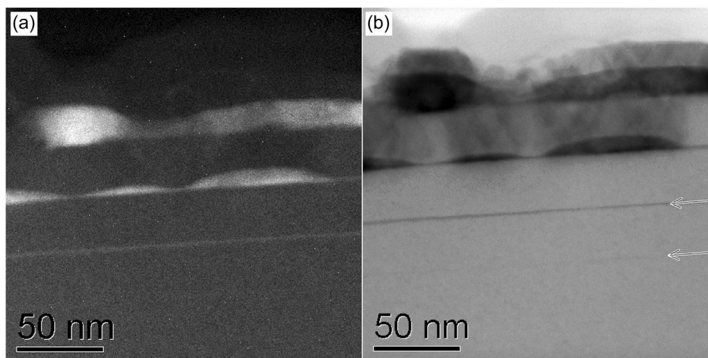
FIGURE 12 Annular dark field (a) and bright field (b) scanning transmission electron microscope images of \text{Ge/Si}(001) .
