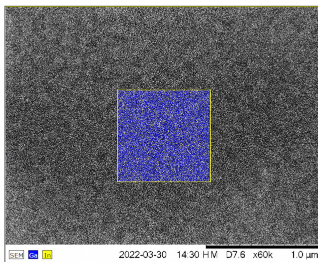
FIGURE 6 Secondary electron image with coloured X-ray map of central (0.8 µm) 2 region of a thin pure InAs layer on surface of GaAs at 15 kV (nom. thickness: 0.45 nm, exp. value calculated: 0.81 \pm 0.24 nm) [9].
