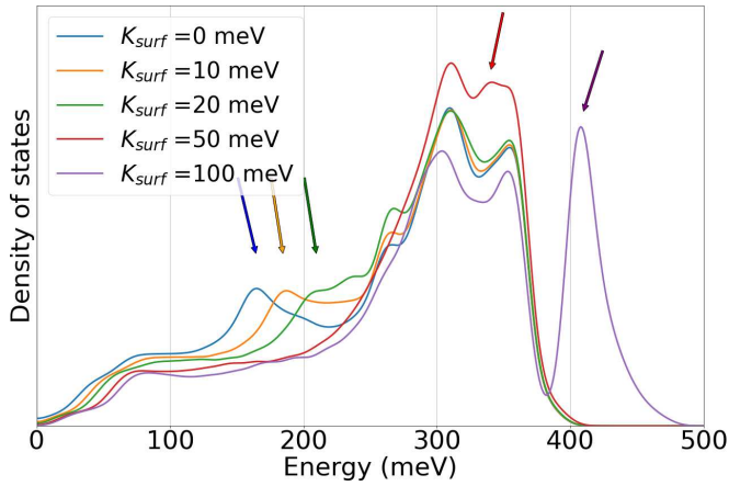
FIG. 3. Density of states of bcc Fe thin film with size 10 monolayers, for varying intensities of K_{surf} with 25 nearest neighbors. A broadening of \Delta = 6.5 meV, was used.
