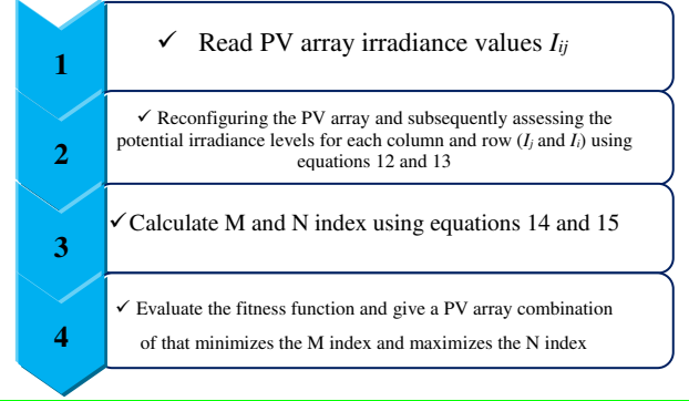
Fig. 8. General procedure for reconfiguring photovoltaic panels based on the proposed approach.
