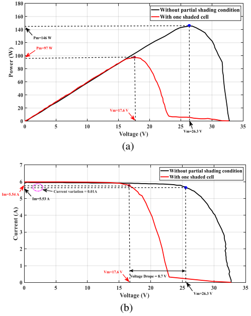
Fig. 4. Experimental PV module's characteristics under partial shading conditions; (a) P-V curve and (b) I-V curve.
