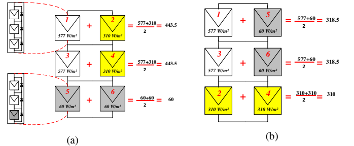
Fig. 6. PV array under shading; (a) initial configuration and (b) reconfiguration using IEq strategy.
