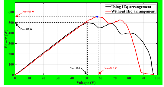
Fig. 7. P-V and I-V characteristics of the TCT and IEq arrangements.
