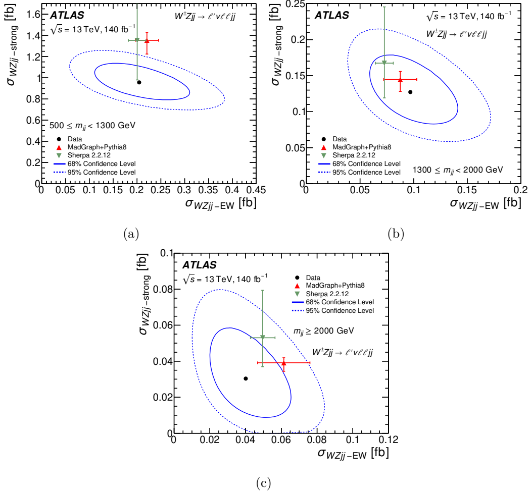
Figure 6. The measured \sigma_{WZjj\text{--}EW} and \sigma_{WZjj\text{--}strong} cross-sections per m_{jj} bin, (a) 500 \leq m_{jj} < 1300 GeV, (b) 1300 \leq m_{jj} < 2000 GeV, (c) m_{jj} \geq 2000 GeV, compared with predictions from MADGRAPH+PYTHIA8 (upward pointing triangle) and SHERPA 2.2.12 (downward pointing triangle). The full and dashed contours around the data points correspond to 68% and 95% CL, respectively.
