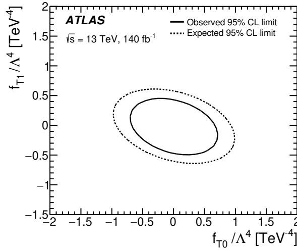
Figure 12. Two-dimensional expected (dashed line) and observed (solid line) 95% CL intervals on Wilson coefficients corresponding to the pair of O_{T0} and O_{T1} operators. No unitarisation procedure is used.
