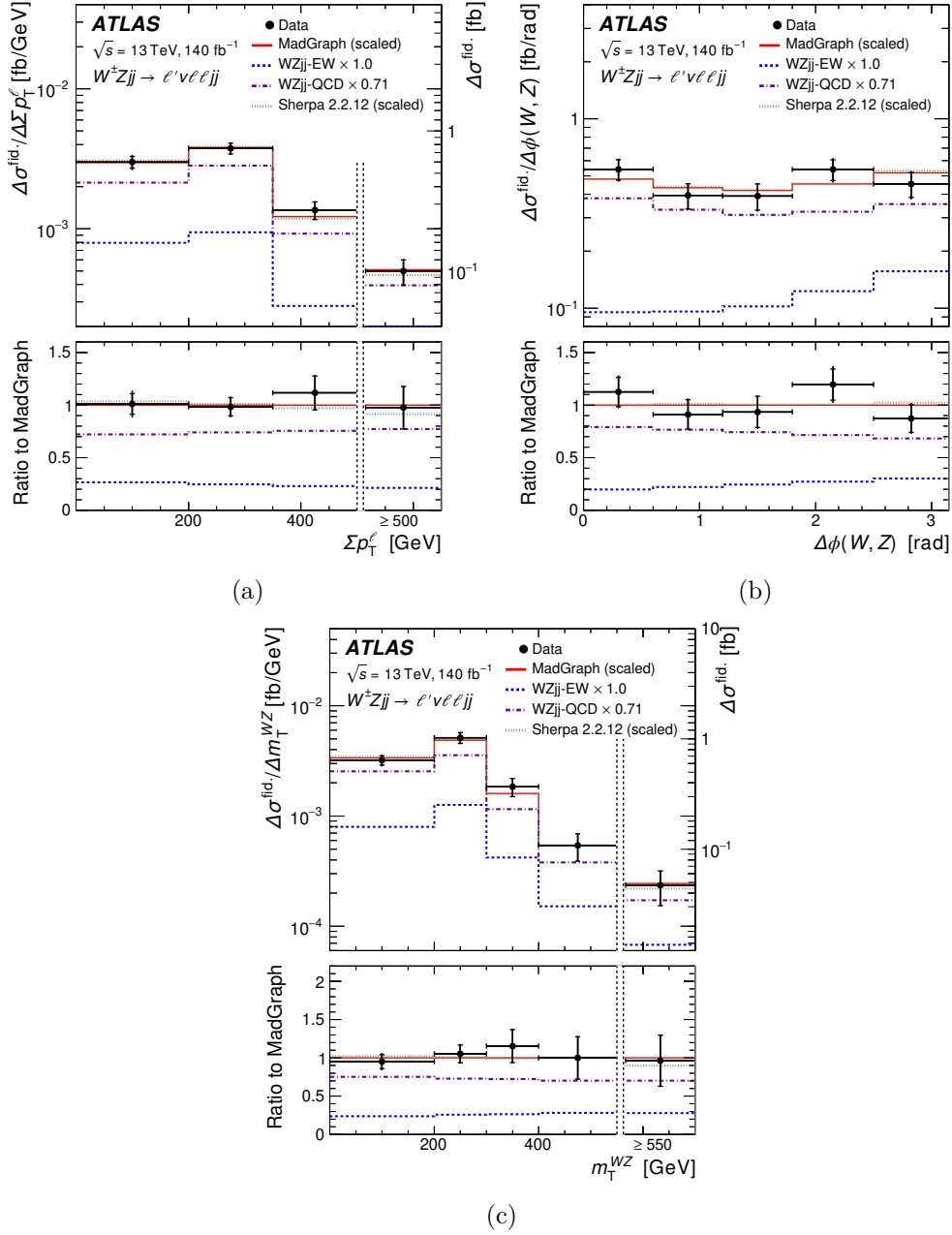
Figure 7. The measured W^\pm Z jj differential cross-section in the VBS fiducial phase space as a function of (a) \sum p_T^\ell , (b) \Delta\phi(W, Z) and (c) m_T^{WZ} . The inner and outer error bars on the data points represent the statistical and total uncertainties, respectively. The measurements are compared with the sum of the rescaled WZjj -QCD and WZjj -EW predictions from MADGRAPH+PYTHIA8 (solid line) and SHERPA 2.2.12 (dotted line). The WZjj -EW and WZjj -QCD contributions are also represented by dashed and dashed-dotted lines, respectively. In (a) and (c), the right y -axis refers to the last cross-section point, separated from the others by a vertical dashed line, as this last bin is integrated up to the maximum value reached in the phase space. The lower panels show the ratios of the data to the predictions from MADGRAPH+PYTHIA8.
