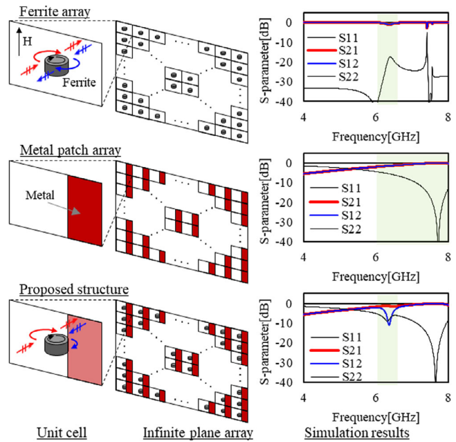
Fig. 1 Proposed nonreciprocal metasurface concept
