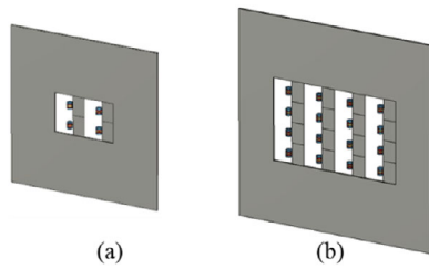
Fig. 3 Simulation model, 2 \times 2 (a) and 4 \times 4 (b)
