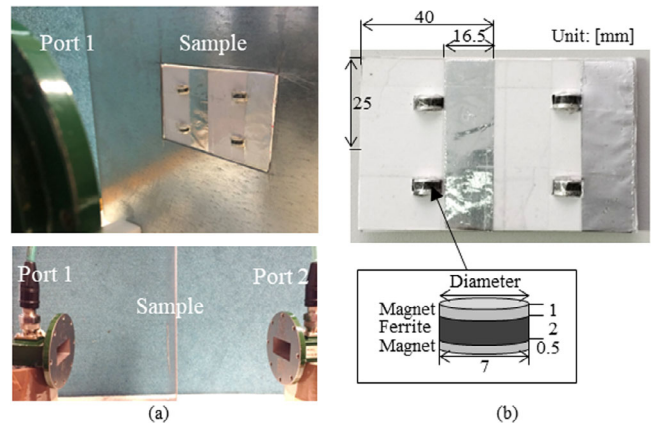
Fig. 2 Experimental setup (a) and 2 \times 2 array sample (b)
