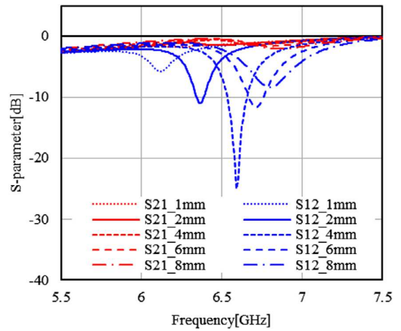
Fig. 5 Simulation results with changing the height of the ferrite
