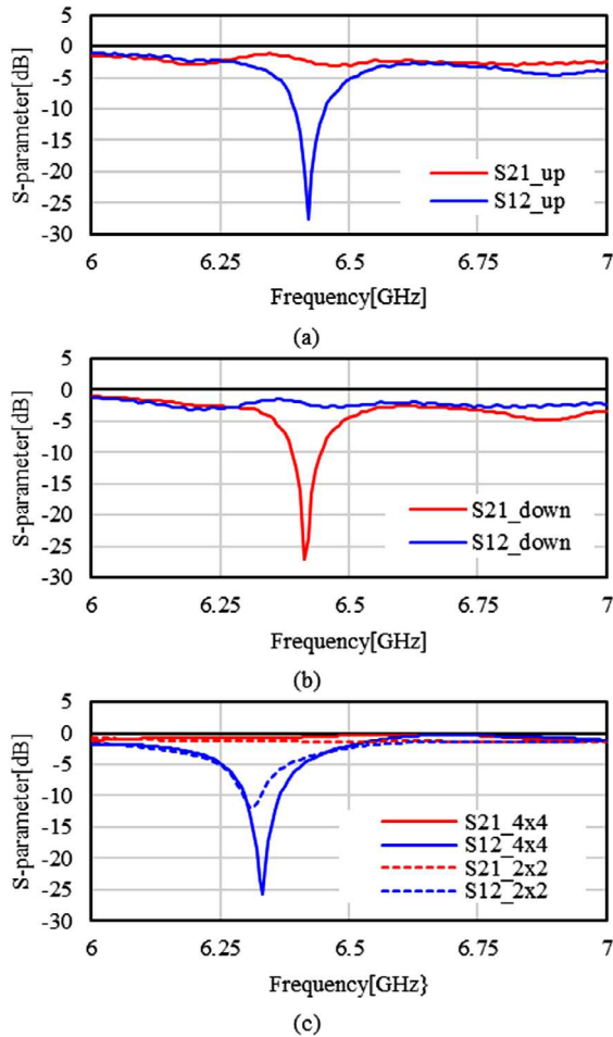
Fig. 4 Experimental results with changing the direction of the magnetic field. Upward magnetic field (a) and downward magnetic field (b), and simulation results for comparison (c)
