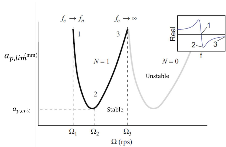
Figure 3: Example SLD plot for N=\{0,1\} , relating points on the real part FRF of the system to the SLD, from [4].
