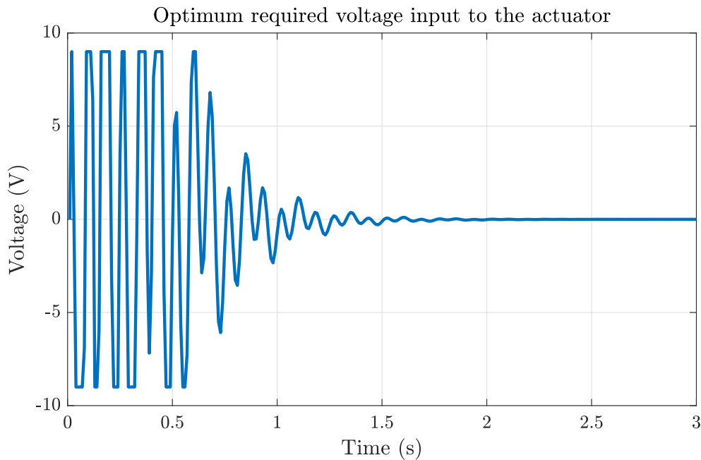
Figure 6: Optimum required voltage input to the actuator.
