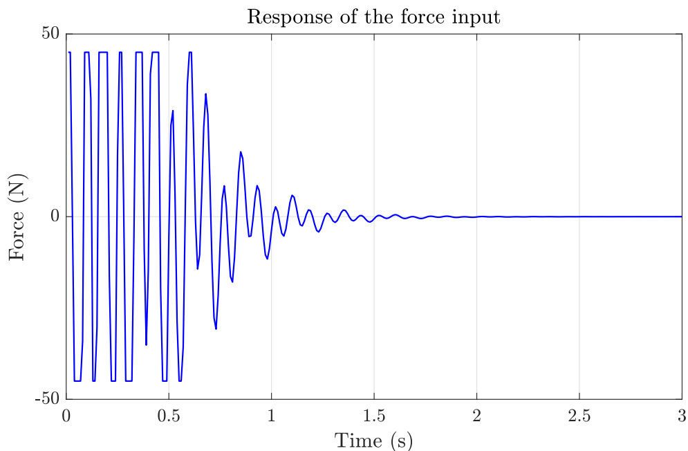
Figure 2: Control input of the cantilever beam.
