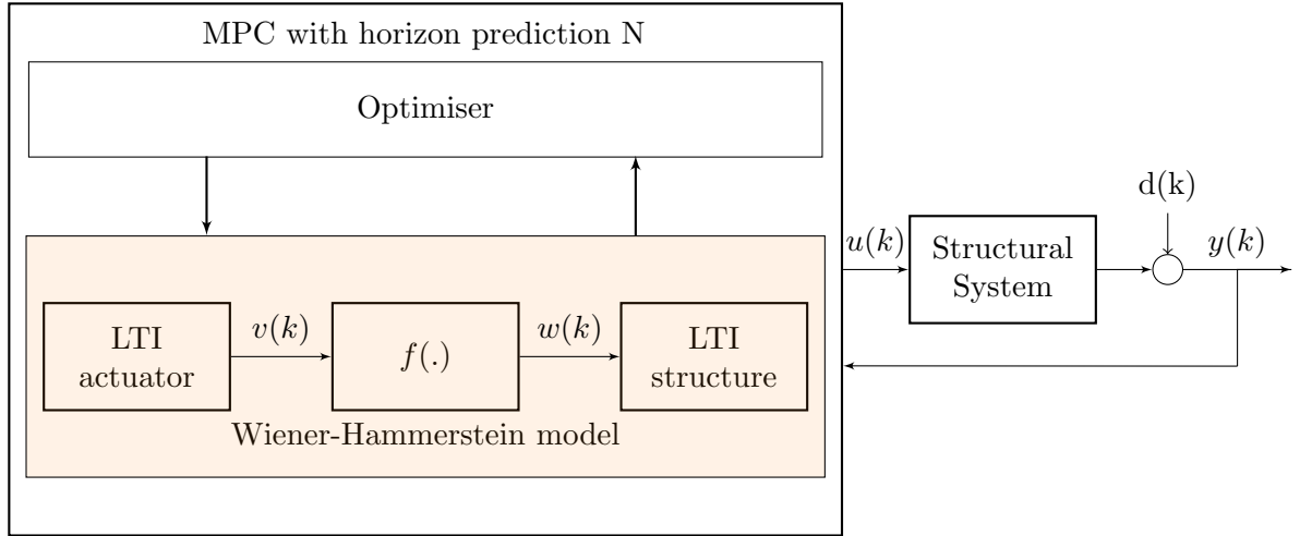
Figure 1: Overview of the proposed control system.
