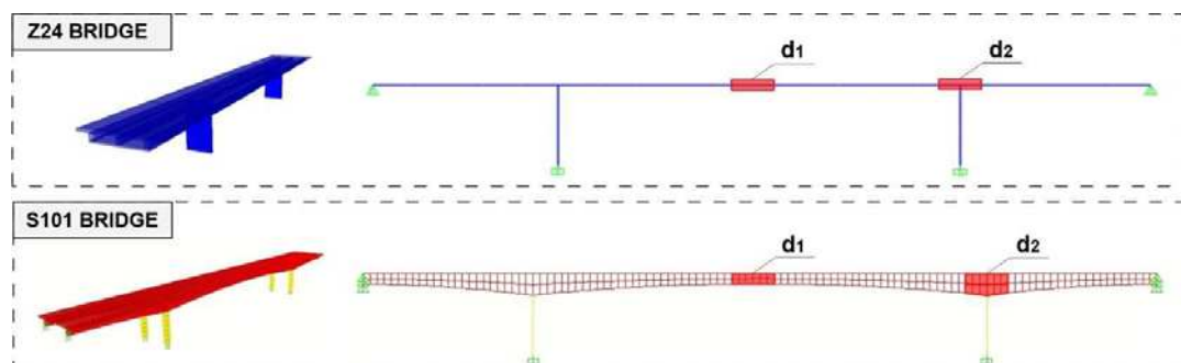
Figure 3. Two damage scenarios are introduced into the FEMs: d_1 and d_2 indicate \sim 12\% and \sim 40\% reduction of E_c , respectively, in the mid span and at the connection between the deck and the pier.
