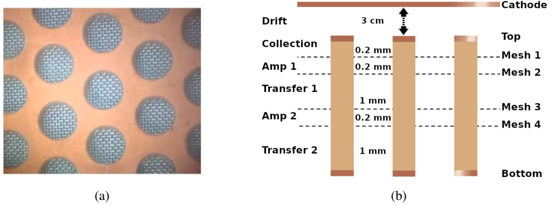
Figure 1. (a) Image of the MMThGEM hole structure as viewed from above. (b) Cross sectional diagram of the MMThGEM device/TPC.
