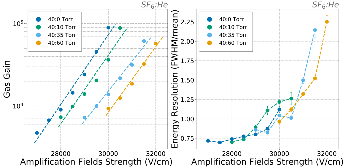
Figure 4. Effective gas gain vs amplification fields strength in \text{SF}_6\text{:He} mixtures (left). Energy resolution vs amplification fields strength in \text{SF}_6\text{:He} mixtures (right). Some error bars are smaller than the marker size and are therefore omitted from the graph.
