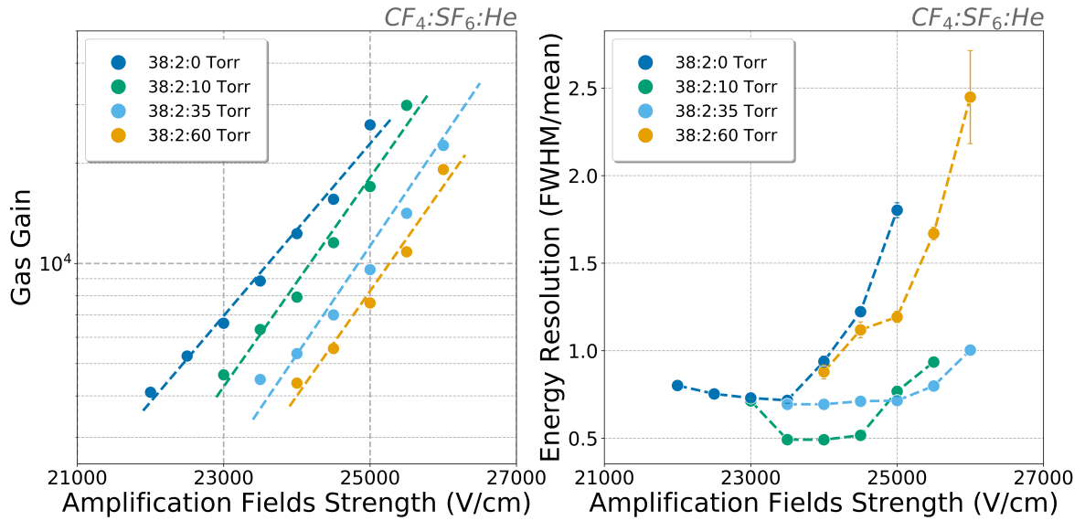
Figure 6. Effective gas gain vs amplification fields strength in \text{CF}_4\text{:SF}_6\text{:He} mixtures (left). Energy resolution vs amplification fields strength in \text{CF}_4\text{:SF}_6\text{:He} mixtures (right). Some error bars are smaller than the marker size and are therefore omitted from the graph.
