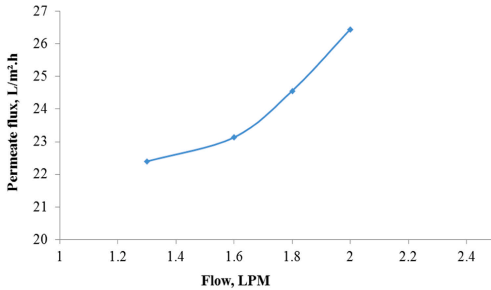
Fig. 14. Effect of recirculation flow rate on permeate flux in the AGMD configuration.
