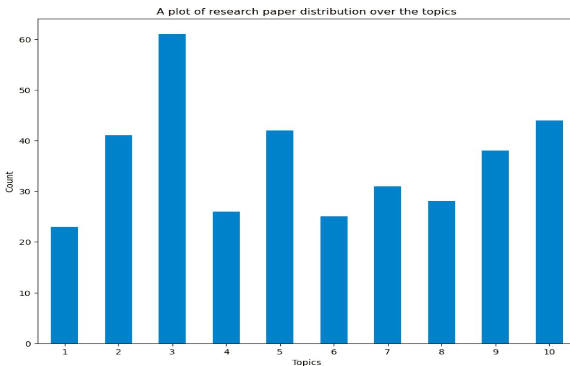
Figure 10. Topic distribution.
